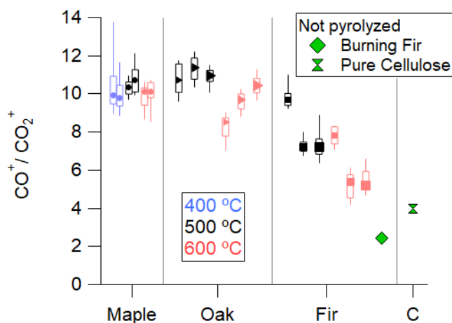
Figure 6. The ratio of particle phase CO^+ to CO_2^+ fragments for maple, oak, Douglas fir, and cellulose (“C”). The order is by fuel, then temperature, then size, markers at median are sized by wood size. Bars of the box correspond to 25 th and 75 th percentiles, and whiskers correspond to 10 th and 90 th percentiles. Default AMS fragmentation table value is unity.
