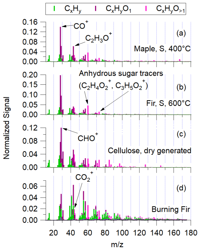
Figure 4. The experiment-averaged mass spectra for small maple at 400 °C (a) and small fir at 600 °C (b) pyrolysis, as well as dry generated cellulose (c) and Douglas fir burning (d).
