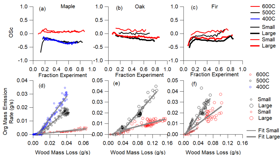
370 Figure 2. The average oxidation state of condensed aerosol over the course of an experiment (a-c), and the emission rate of aerosol compared with the mass loss rate of the wood (emission index, d-f) for each experimental condition.
