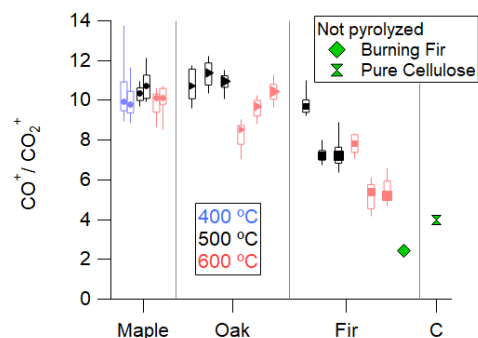
555 Figure 6. The ratio of particle phase CO^+ to CO_2^+ fragments for maple, oak, Douglas fir, and cellulose (“C”). The order is by fuel, then temperature, then size, markers at median are sized by wood size. Bars of the box correspond to 25 th and 75 th percentiles, and whiskers correspond to 10 th and 90 th percentiles. Default AMS fragmentation table value is unity.
