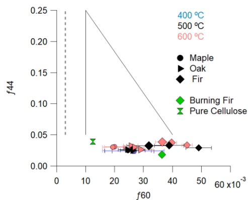
Figure 8 Fraction of \text{CO}_2^+ ( m/z 44) to fraction of \text{C}_2\text{H}_3\text{O}^+ ( m/z 60) as an indicator of atmospherically relevant biomass burning. Each value is an experiment average with bars indicating the standard deviation. The dotted vertical line represents the nominal ambient background value of 0.3% from Cubison et al. (2011). The solid lines forming two-thirds of a triangle represent the bounds observed by Cubison et al. (2011), which would be generally expected for measurements of fresh to aged biomass burning in the atmosphere.
