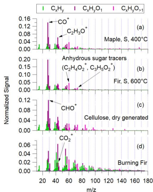
450 Figure 4. The experiment-averaged mass spectra for small maple at 400 °C (a) and small fir at 600 °C (b) pyrolysis, as well as dry generated cellulose (c) and Douglas fir burning (d).
