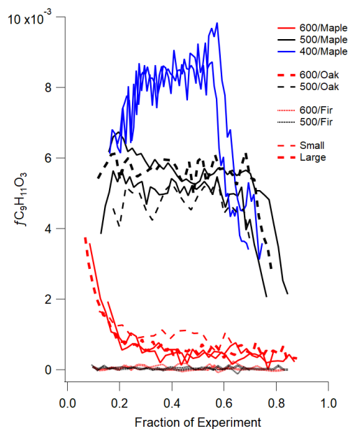
570 Figure 7. The fraction of C_9H_{11}O_3^+ in the total organics for each small and large wood size experiment. The fragment is only in maple and oak spectra and is only emitted at the beginning of higher temperature set points before wood temperature has increased.
