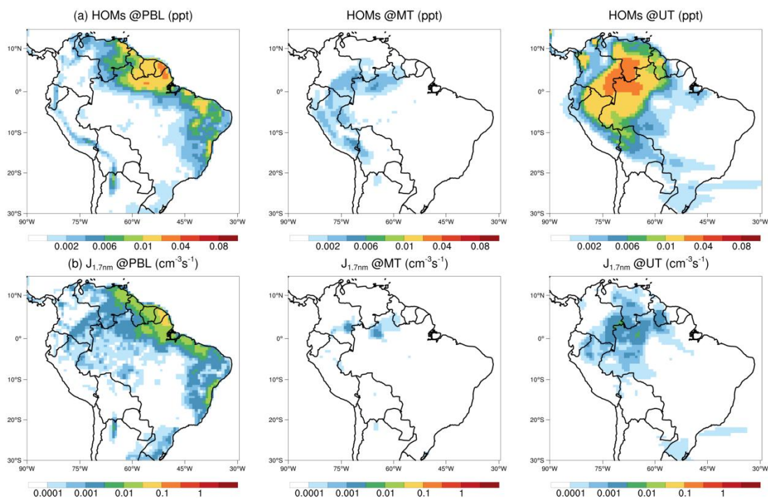
Figure A11. Horizontal distribution of (a) HOMs and (b) organic nucleation rate averaged over 1 Sep–1 Oct 2014 from the BNUnOT case, all at STP.
