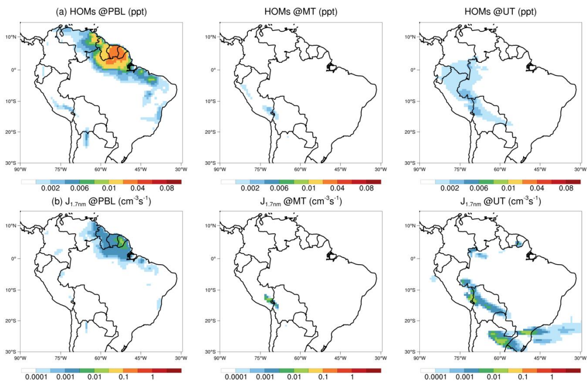
760 Figure A15. Horizontal distribution of (a) HOMs and (b) organic nucleation rate averaged over 1 Sep–1 Oct 2014 from the NoOH case, all at STP.
