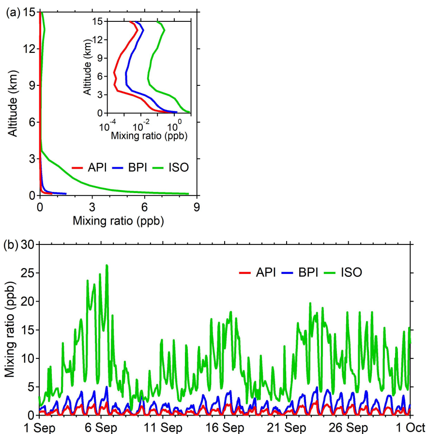
655 Figure A4. Simulated (a) vertical profiles and (b) time series of \alpha -pinene (API), \beta -pinene (BPI), and isoprene (ISO) mixing ratios (STP) at the location of ATTO. The embedded figure in (a) is the same as the outer figure but on a log scale.
