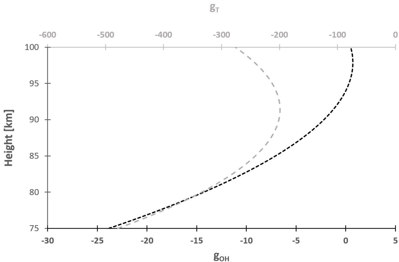
220 Figure 2 Height-dependent development of g_T (grey) and g_{OH} (black) according to the formulas (42) and (29) of Swenson and Gardner (1998) calculated for January: while g_{OH} decays nearly linearly to zero, this is not the case for g_T . Among other arithmetic operations, these factors are multiplied by the relative density perturbation and the undisturbed VER in order to derive the rotational temperature and the relative intensity perturbation. So, it becomes clear that relative intensity perturbations suffer less from averaging effects than the rotational temperature perturbation.
