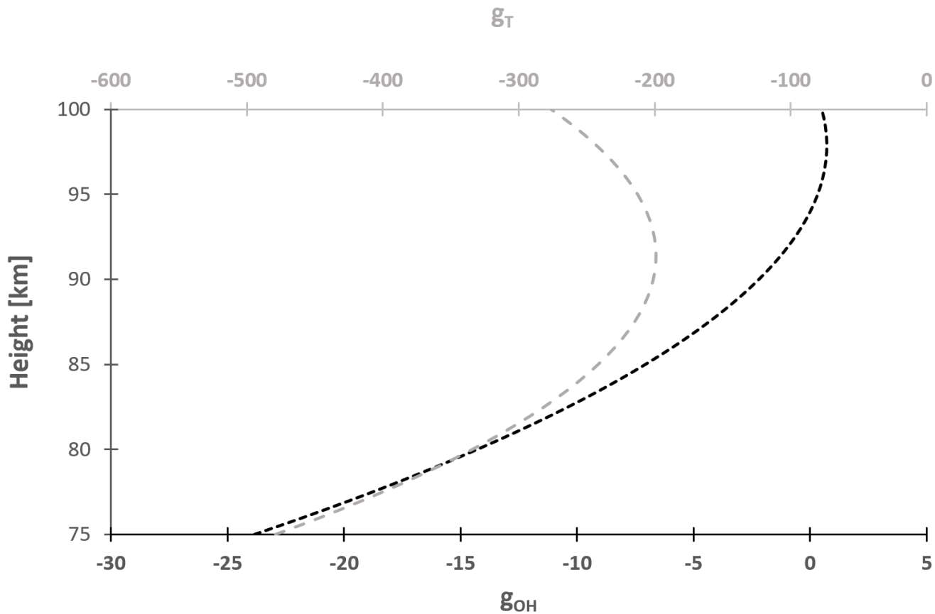
230 Figure 2 Height-dependent development of g_T (grey) and g_{OH} (black) according to the formulas (42) and (29) of Swenson and Gardner (1998) calculated for January: while g_{OH} decays nearly linearly to zero, this is not the case for g_T . Among other arithmetic operations, these factors are multiplied by the relative density perturbation and the undisturbed VER in order to derive the rotational temperature and the relative intensity perturbation. So, it becomes clear that relative intensity perturbations suffer less from averaging effects than the rotational temperature perturbation.
