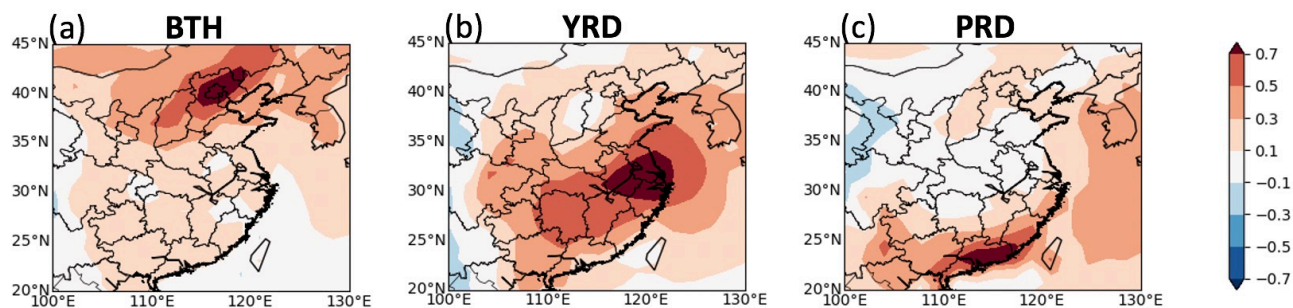
Figure 2: Correlation coefficients of daily mean \text{PM}_{2.5} concentrations over all UKESMI grid cells with those in the grid cells covering (a) Beijing, (b) Shanghai and (c) Guangzhou during DJF 1999–2018. Regions where correlations are higher than 0.7 (dark red shading) are selected to represent the Beijing–Tianjin–Hebei (BTH), Yangtze River Delta (YRD) and Pearl River Delta (PRD) regions.
