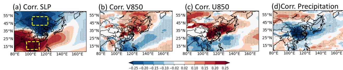
Figure 5: Correlation coefficients of daily \text{PM}_{2.5} concentrations in YRD with (a) SLP, (b) V850, (c) U850 and (d) precipitation from nudged UKESM1 during DJF 1999–2018. Dotted regions indicate significant correlations at the 95% level from a two-tailed Student's t -test. Grey shading represents the YRD region. The regions used for the definition of a circulation-based index for YRD (eq. 1) are marked by two yellow rectangles in panel a.
