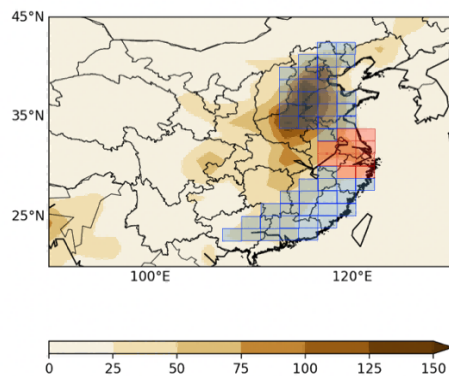
Figure 8: Spatial distribution of the winter mean daily \text{PM}_{2.5} concentrations ( \mu\text{g}/\text{m}^3 ) simulated by UKESM1 across China during DJF 2014–2018 (shaded colours) and UKESM1 model grid cells representing north China (top blue grid cells), YRD (red grid cells) and south China (bottom blue grid cells).
