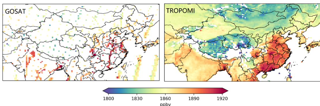
130 Figure 1: 2019 annual average methane column mole fractions over the East Asia domain for GOSAT (UoL proxy v9.0 retrieval) and TROPOMI (Lorente et al. (2021) full-physics retrieval), presented on the 0.5^\circ \times 0.625^\circ GEOS-Chem grid.
