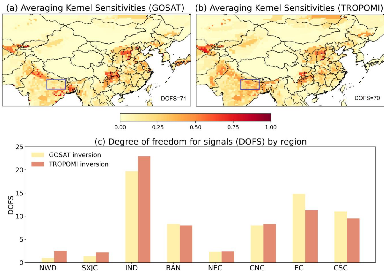
390 Figure 7: Averaging kernel sensitivities for GOSAT (a) and TROPOMI (b) inversions. Values represent the ability of observations to constrain methane emissions (0 = not at all, 1 = perfectly). The east Ganges Plain is marked by blue rectangles. Panel (c) compares the DOFS of regional emissions constrained by TROPOMI and GOSAT inversions.
