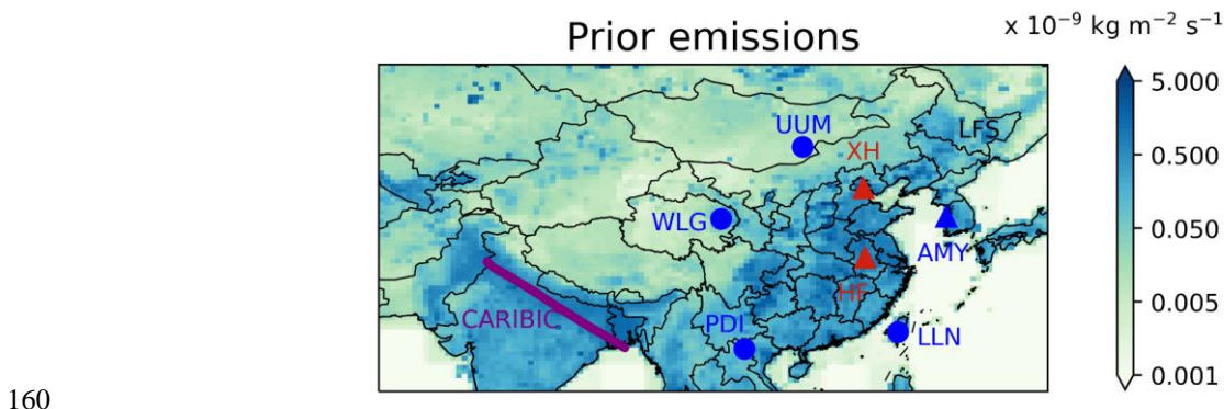
Figure 2: Spatial distribution of prior emissions. Locations of independent data for evaluation (seven surface sites and aircraft route) are shown. Circles represent background sites and triangles source-region sites. Total column measurements are coded in red and in situ measurements in blue. Purple solid line shows a CARIBIC aircraft route that measured tropospheric methane over India on November 22, 2012.
