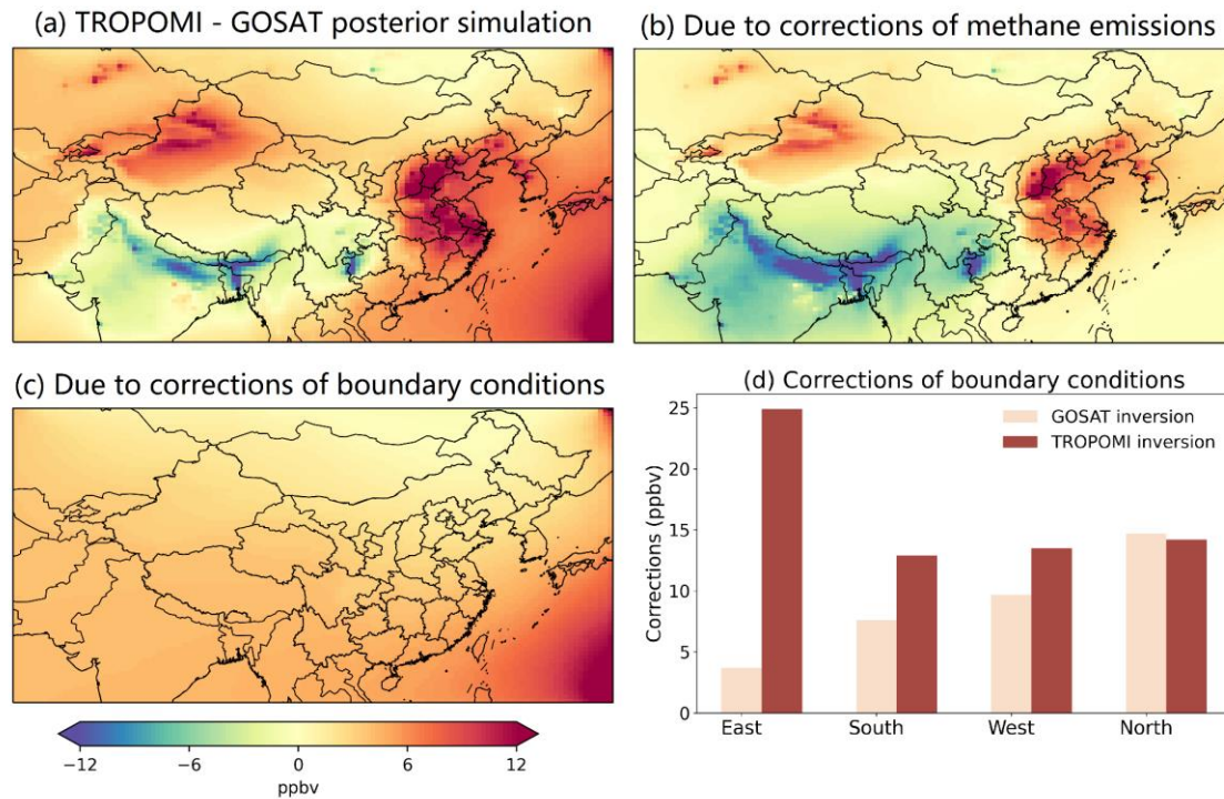
340 Figure 5: Differences in tropospheric methane concentrations (TROPOMI - GOSAT) between GOSAT and TROPOMI posterior simulations. (a) shows the total differences while (b) and (c) decompose the differences to methane emissions and boundary condition bias corrections. The corrections of boundary conditions (in ppbv) by the two inversions are shown.
