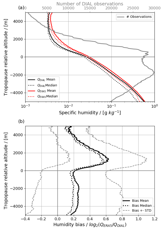
290 Figure 5: Tropopause-relative (a) vertical profiles of the DIAL (black lines) and the ERA5 (red lines) mean (solid) and median (dotted) specific humidity and the number of observations (grey). Note the log-scale notation of the x-axis. (b) Mean/median bias (solid/dotted lines) and standard deviation (grey dotted lines).
