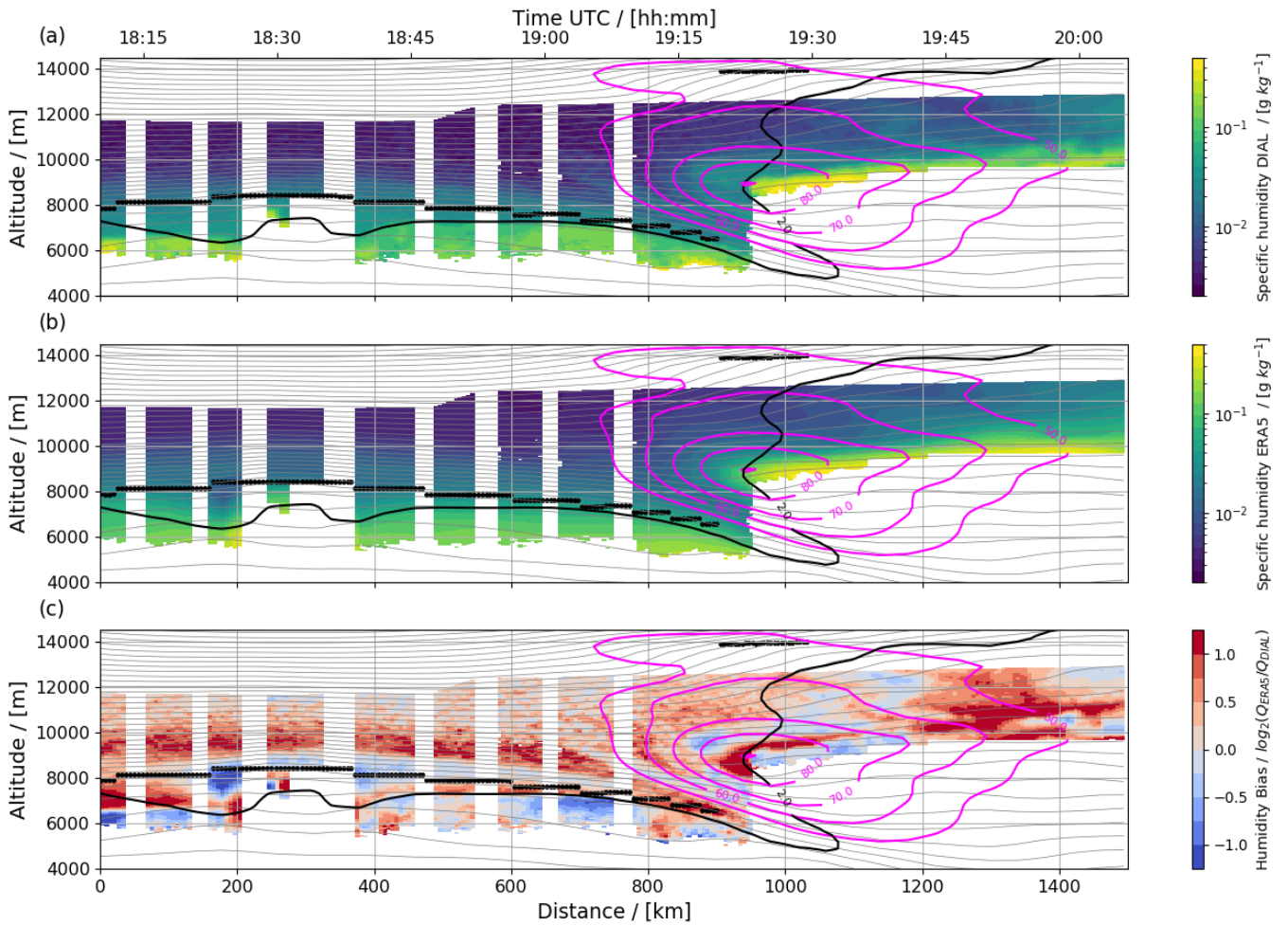
270 Figure 4: Vertical cross sections of (a) the DIAL specific humidity (colour shading, \text{g kg}^{-1} ), (b) ERA5 specific humidity (colour shading, \text{g kg}^{-1} ) as well as (c) the corresponding humidity bias (colour shading) on the 1 st October 2017. (a) – (c) are superimposed by ERA5 fields of the potential temperature (grey contours, \Delta\theta = 3\text{K} ) and the isopleths of the wind speed (magenta contours, in \text{m s}^{-1} ), and the thermal (thick black dots) and the dynamical tropopause (2 PVU, black isoline).
