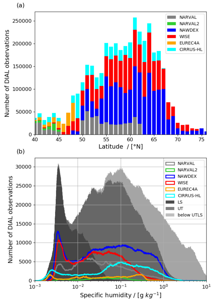
Figure 2: (a) Stacked distribution of the number of observations in 1^\circ latitude bins per individual campaigns (coloured bars). (b) Histogram of observations per humidity bin with a size of 0.01 \text{ g kg}^{-1} of \log_{10}(q_{\text{DIAL}}) for individual campaigns in the UTLS (coloured lines). Shading shows frequencies separated for the LS (all data above the thermal tropopause, dark grey shading), the UT (all data between the tTP and 5 km below, medium grey shading) and the remaining tropospheric data (light grey shading).
