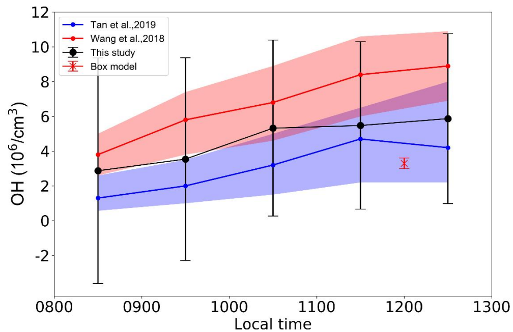
Figure 4: Hourly average OH concentrations between 08:00 and 13:00 derived from the OBM are shown in black line with black dots; observed OH concentrations by Tan et al. (2019) are shown in blue line and blue shade; calculated OH concentrations by Wang et al. (2018) are shown in red line and red shade. The blue shade denotes the 25% and 75% percentiles of the data, the red shade indicates the 95% C. I. of the data. The red cross with red vertical whiskers denotes the mean OH concentration and 1-standard deviation, respectively, calculated by a box model constrained by observed ambient conditions during the two episodes.
