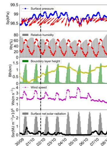
Figure 4: Same as Fig. 3 except for meteorological parameters.
