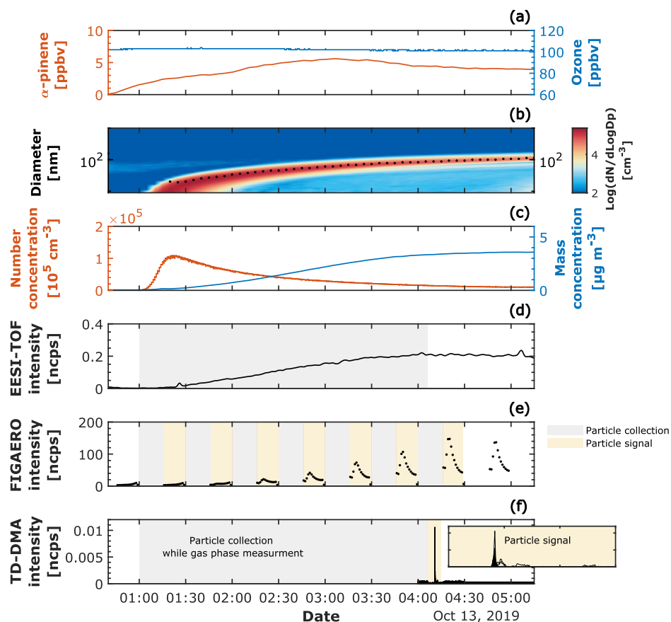
835 Figure 1. Experimental overview of a representative biogenic new particle formation experiment ( \alpha -pinene ozonolysis at -30\text{ }^{\circ}\text{C} and 20 % RH). (a) Mixing ratio in ppbv for the precursor gases, \alpha -pinene and ozone. (b) Particle size distribution measured by the SMPS; the color scale represents the log 10 of the normalized particle concentration per cubic centimeter ( \text{cm}^{-3} ). The median mass diameter (MMD) is shown with a black dashed line. (c) Particle number concentration in \text{cm}^{-3} measured by the CPC with a cut-off diameter of 2.5 nm and mass concentration in \mu\text{g m}^{-3} (obtained by integrating the normalized mass concentration from the SMPS). 840 (d) Particle-phase signal measured continuously by the EESI-TOF, the gray shaded area refers to the period where the EESI-TOF was averaged for the intercomparison with TD-DMA and FIGAERO. (e) Particle-phase measured by FIGAERO, the gray shaded areas refer to the particle collection period and the yellow shaded areas to the desorption period. FIGAERO measured in a semicontinuous mode, namely 15-minute particle collections followed by 15-minute desorption periods. In order to intercompare with EESI-TOF and TD-DMA, FIGAERO signals were integrated during the period where the TD-DMA collected particles (~3 845 hours), seven FIGAERO particle samples were integrated during the 3 hours comparison period. (f) Particle-phase measured by the TD-DMA; The TD-DMA particle collection period was approximately 3 hours while the desorption period lasted around 1 minute followed by a second heating for estimating the background.
