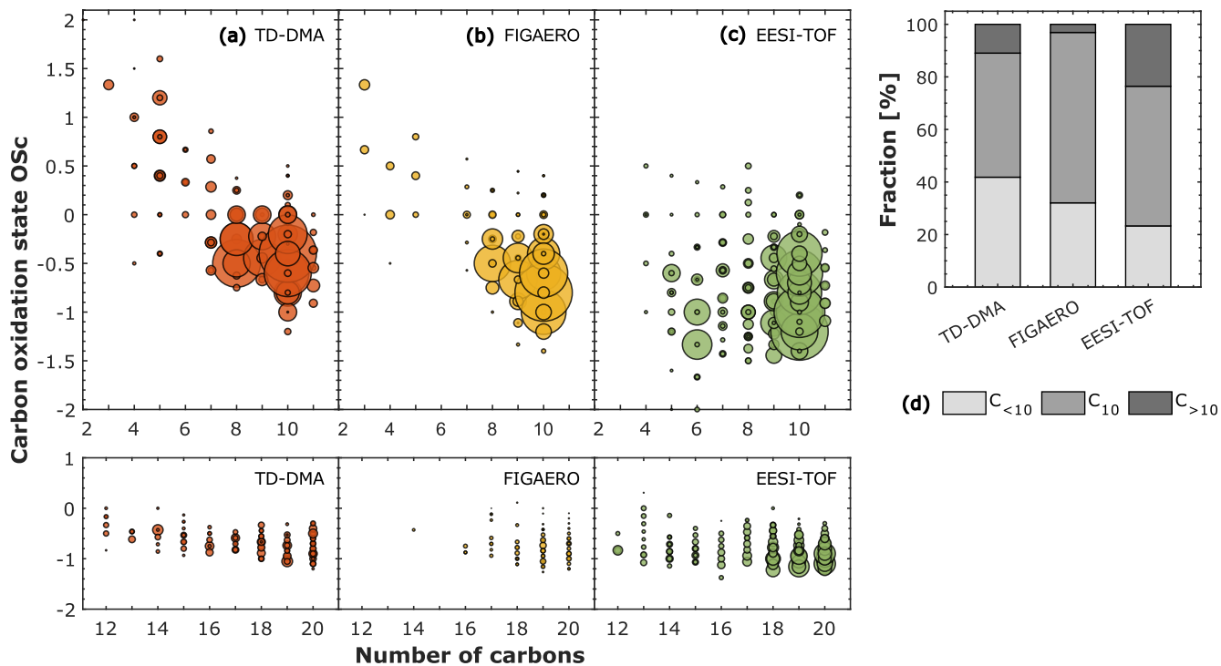
865 Figure 2. Carbon oxidation state Osc against the number of carbon atoms for \alpha -pinene oxidation products in the particle-phase at -30\text{ }^{\circ}\text{C} and 20\text{ }\% RH measured by three different techniques. (a) TD-DMA: Thermal Desorption-Differential Mobility Analyzer coupled to a \text{NO}_3^- chemical ionization-atmospheric-pressure-interface-time-of-flight mass spectrometer. (b) FIGAERO: Filter Inlet for Gases and AEROsols coupled to an I - high-resolution time-of-flight chemical-ionization mass spectrometer, and (c) EESI-TOF: Extractive Electrospray \text{Na}^+ Ionization time-of-flight mass spectrometer. The level of \alpha -pinene was between 1 and 6 ppbv while the ozone level was \sim 100 ppbv. The carbon oxidation state is calculated as follows: \text{Osc} = 2x\text{O}:\text{C} - \text{H}:\text{C} . The marker sizes in (a), (b), and (c) represent the intensities normalized by the total signal in each system. (d) Fraction of species in the particle-phase containing less than 10 carbon atoms ( \text{C}_{<10} ), 10 carbon atoms ( \text{C}_{10} ), and more than 10 carbon atoms ( \text{C}_{>10} ). The fraction was calculated by normalizing the intensities by the total signal in each system.
