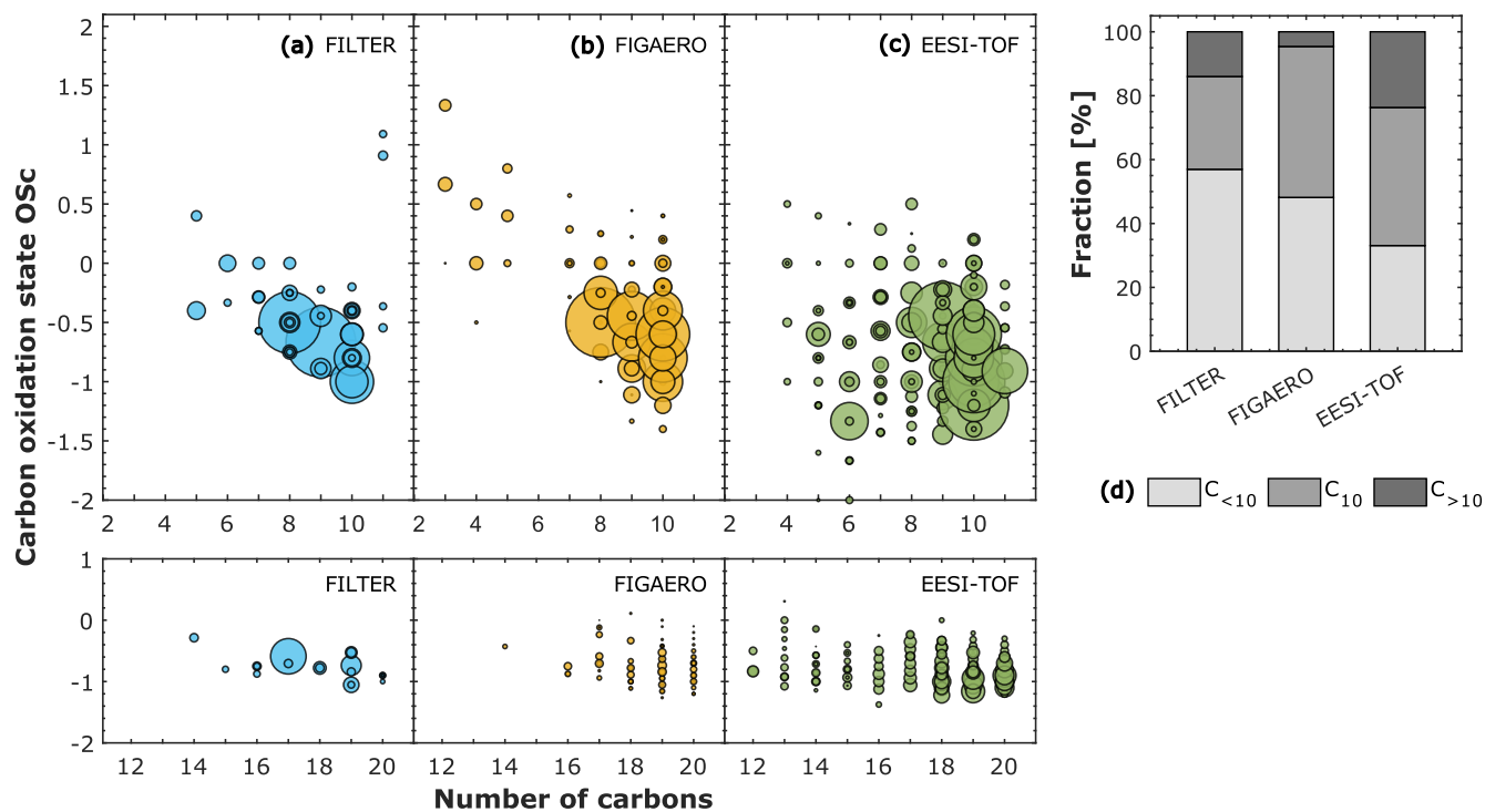
890 Figure 3. Carbon oxidation state OSc against the number of carbon atoms for \alpha -pinene oxidation products in the particle-phase at -10 °C and 80 % RH measured by three different techniques. (a) FILTER: Offline analysis of filters using Ultra-high-performance liquid chromatography (UHPLC) and heated electrospray ionization (HESI) coupled to an Orbitrap high-resolution mass spectrometer (HRMS). (b) FIGAERO: Filter Inlet for Gases and AEROSols coupled to an I high-resolution time-of-flight chemical-ionization mass spectrometer, and (c) EESI-TOF: Extractive Electrospray Na + Ionization time-of-flight mass 895 spectrometer. The level of \alpha -pinene was between 1 and 3 ppbv while the ozone level was ~100 ppbv. The carbon oxidation state is calculated as follows: OSc = 2 \cdot O:C - H:C . The symbol sizes in (a), (b), and (c) represent the intensities normalized by the total signal in each system. (d) Fraction of species in the particle-phase containing less than 10 carbon atoms ( C_{<10} ), 10 carbon atoms ( C_{10} ), and more than 10 carbon atoms ( C_{>10} ). The fraction was calculated by normalizing the intensities by the total signal in each system.
