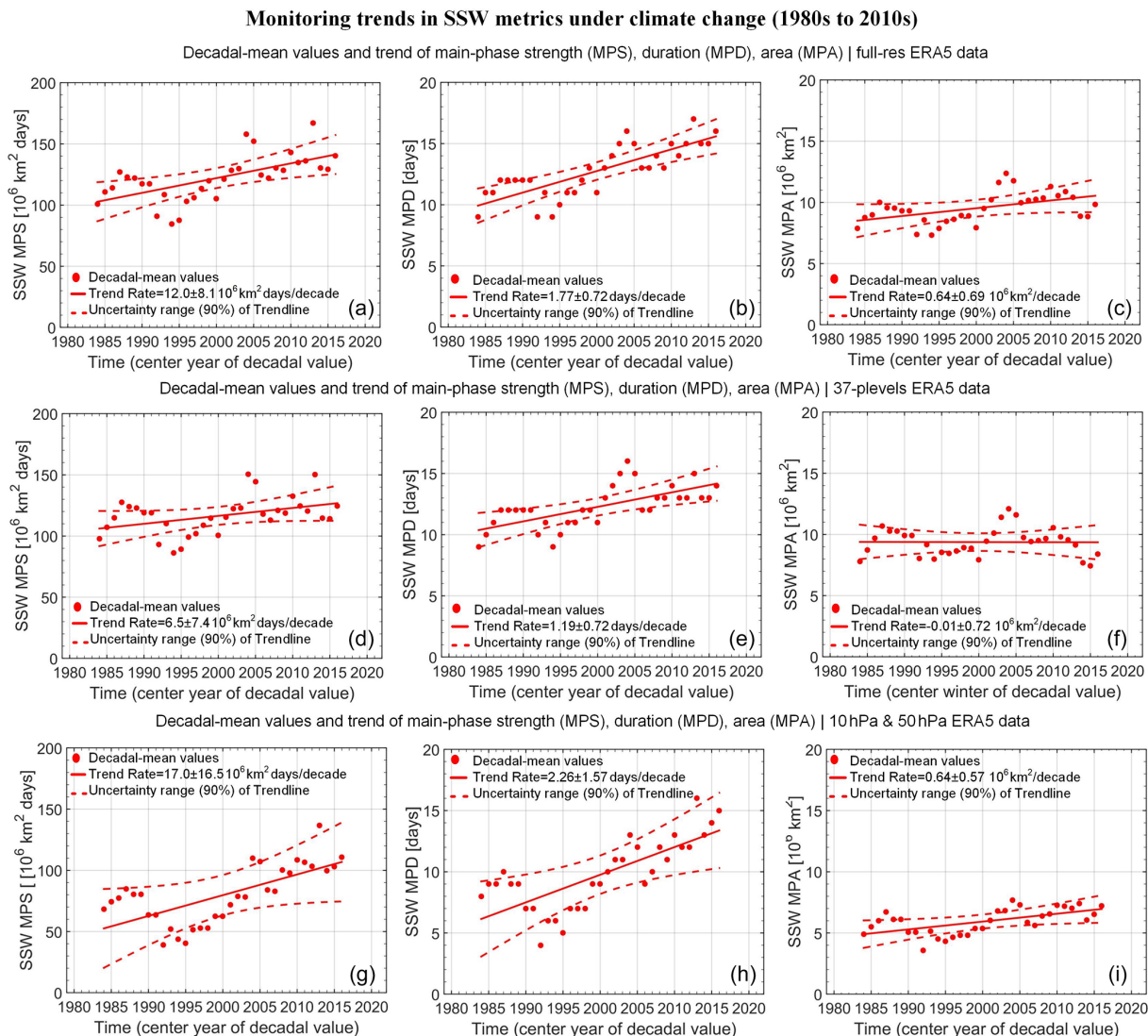
Figure 11. Monitoring and assessment of long-term trends in the three core SSW metrics (main-phase strength, duration, and area) along the recent climate change period from the 1980s decade to the 2010s decade, noting also main statistical numbers within the respective panel legends. The results derive from the metrics as illustrated in Fig. 10 and are intercompared for the ERA5 temperature data input either taken in at full 137-model-levels resolution (“full-res ERA5 data”) (a–c), coarser standard 37-pressure-levels resolution (“37-plevels ERA5 data”) (d–f), or simple two-levels data extraction (“10 hPa & 50 hPa ERA5 data”) (g–i), respectively. For a description, see Sect. 5.2.
