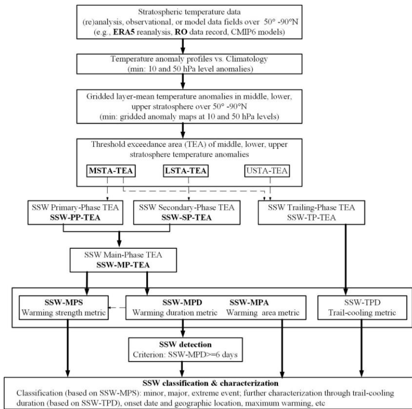
1080 Figure 2. Schematic overview of the new SSW detection and monitoring approach and its main algorithmic steps from the 1085 temperature input data (top) to the final SSW metrics (in particular SSW-MPD, SSW-MPA, SSW-MPS) and their use for detection, classification and further event characterization (bottom). For implementation details see Tables 1 and 2 and the description in Section 3.3.
