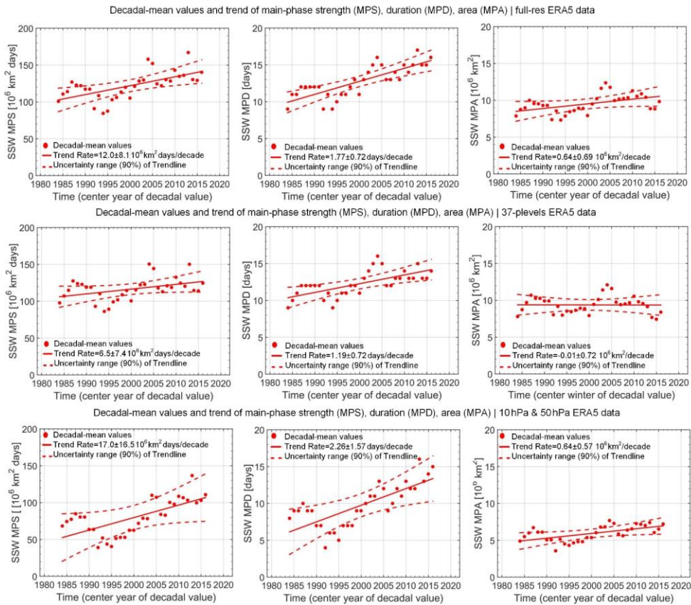
1170 Figure 11. Monitoring and assessment of long-term trends in the three core SSW metrics (main-phase strength, duration, and area) along the recent climate change period from the 1980s decade to the 2010s decade, noting also main statistical numbers within the respective panel legends. The results derive from the metrics as illustrated in Figure 10 and are intercompared for the ERA5 temperature data input either taken in at full 137-model-levels resolution (“full-res ERA5 data”) (top row), coarser standard 37-pressure-levels resolution (“37-levels ERA5 data”) (middle row), or simple two-levels data extraction (“10hPa & 50hPa ERA5 data”) (bottom row), respectively. For description see Section 5.2.
