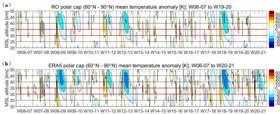
Figure 4. Temporal evolution of polar-cap mean ( 60^{\circ}\text{N} - 90^{\circ}\text{N} ) daily mean temperature anomaly profiles from RO (a) and ERA5 (b), over four winter months each (December, January, February, March), for the winters from 2006-07 (W06-07) to 2019-20 for RO (W19-20) and 2020-21 for ERA5 (W20-21). The RO dataset did not yet cover the W20-21 time period.
