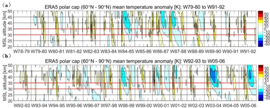
Figure 5. Temporal evolution of polar-cap mean ( 60^{\circ}\text{N} - 90^{\circ}\text{N} ) daily mean temperature anomaly profiles from ERA5, over four winter months each (December, January, February, March), for the winters from W79-80 to W91-92 (a) and from W92-93 to W05-06 (b), respectively. The W78-79 time period was not covered by the ERA5 dataset used.
