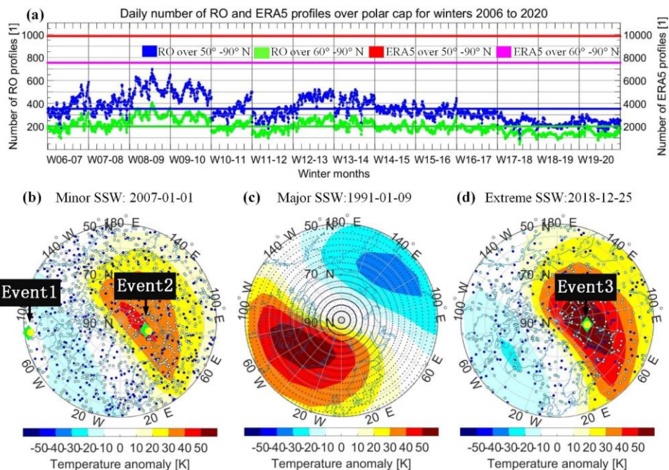
Figure 1. Number and distribution of RO and ERA5 profile data over the Northern polar region. (a): Daily number of RO events over 50°-90° N (blue dots) and 60°-90° N (green dots) for 14 winters from W06-07 to W19-20, with the blue and green horizontal lines showing the related long-term average number, as well as the (constant) daily number of ERA5 grid-point profiles (four analysis times per grid point per day: red and magenta lines); (b): illustrative distribution of RO event locations on 01 Jan 2007 (blue dots), and on the previous and next days (light blue dots), over-plotted on the middle-stratosphere temperature anomaly (MSTA) of the day (color bar), on which a minor SSW prevailed; (c): distribution of the regular ERA5 grid-point profile locations (2.5° latitude × 2.5° longitude grid), over-plotted on the MSTA of 09 Jan 1991, where a major SSW prevailed; (d): illustrative distribution of RO event locations on 25 Dec 2018 in the same style as in (b), over-plotted on the MSTA of the day, on which an extreme SSW prevailed. The green diamonds / yellow circles in (b) and (d) show the location of three exemplary RO events / ERA5 profiles (Event1 to Event3) that are located in different SSW anomaly strength conditions and used in Fig. 2 to illustrate the anomalies construction concept.
