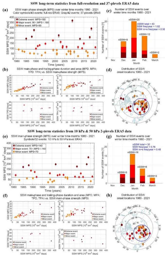
Figure 10. Overview of main characteristics of the SSW events recorded over the 42 winters from 1980 to 2021 using the new monitoring approach based on ERA5 temperature data input at full 137-model-levels resolution (“full-res ERA5”) (upper-half part, a-d ), coarser standard 37-pressure-levels resolution (“37-levels ERA5”) (co-illustrated in a-b with non-filled symbols),
