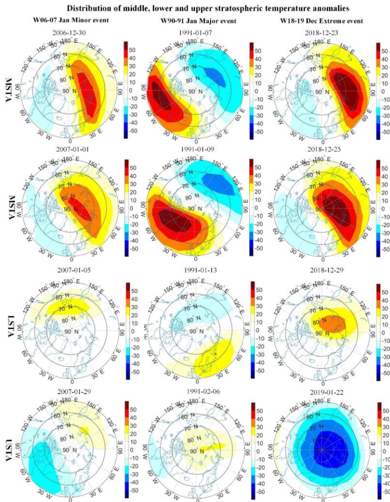
Figure 6. Polar-view (50°–90°N) contour maps of W06-07 Jan Minor (left), W90-91 Jan Major (middle) and W18-19 Dec Extreme (right) SSW example events (cf. Figs. 1 and 6), illustrating ERA5-based Middle Stratosphere Temperature Anomalies (MSTA), Lower Stratosphere Temperature Anomalies (LSTA), and Upper Stratosphere Temperature Anomalies (USTA). MSTA (top and second row) is shown two days before and on the defined onset date (see Table 2 for definition), LSTA (third row) 4 days after the onset date, and USTA (bottom) 4 weeks after the onset date, respectively.
