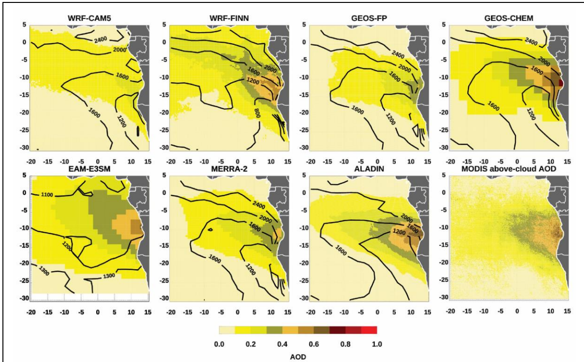
Figure 8. Monthly mean modeled AOD in the FT at 12Z and MODIS (Terra and Aqua) ACAOD for September 2016. Contours are PBL heights in meters.
