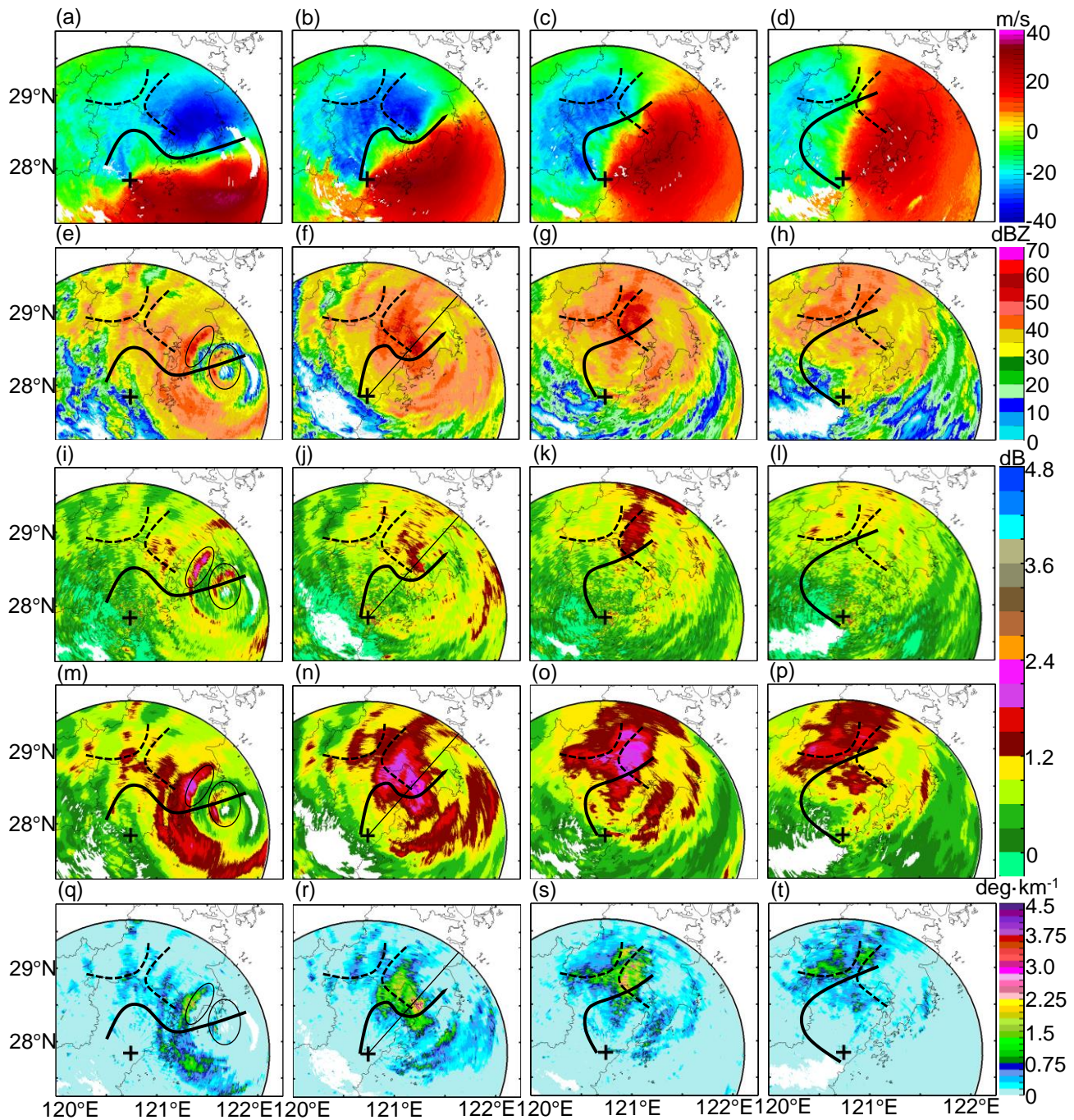
850 Fig. 11. WZ-SPOL radar measurements during typhoon Lekima: (a)-(d) are Doppler velocity V_R at 1601 UTC, 1759 UTC, 2002 UTC, and 2200 UTC, 09 August 2019, respectively; (e)-(h), (i)-(l), (m)-(p), (q)-(t) are Z_H^C , Z_{DR}^C , Z_{DR} and K_{DP} simultaneously as (a)-(d). The solid black lines refer to wind shear deduced from V_R . The black dashed lines refer to the GWS of KCM and YDM, and “+” indicates the location of the WZ-SPOL radar. The ellipses in (e), (i), (m), and (q) indicate where hydrometeor size sorting occurred. The black lines along the radial profiles in (f), (j), (n), and (r) indicate the azimuthal angle shown in Fig. 18.
