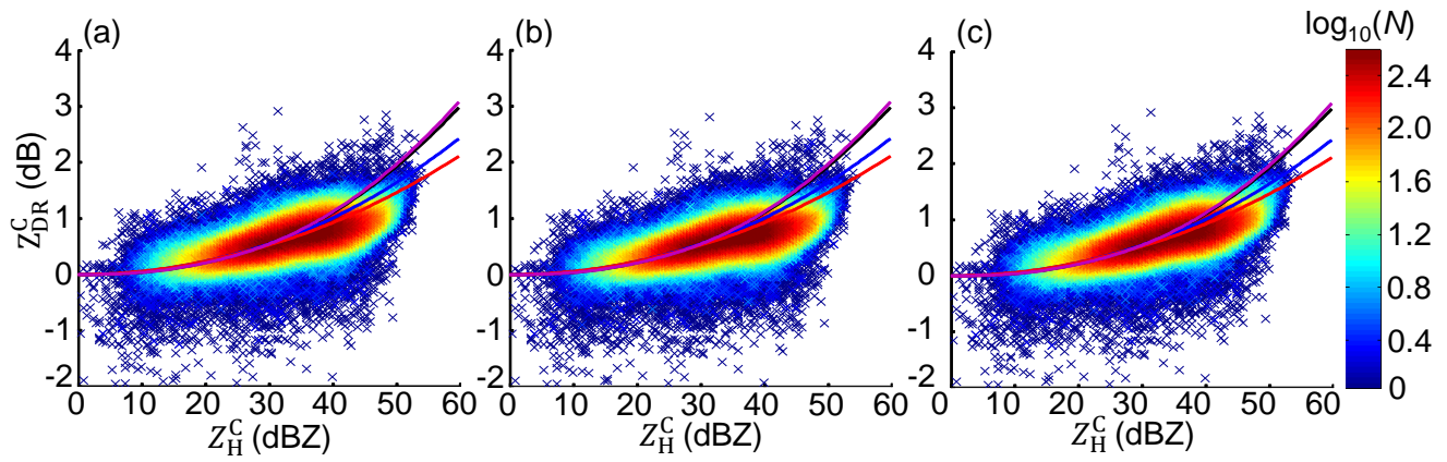
Fig. 24. Scattergrams between Z_{DR}^C and Z_H^C , respectively, utilizing \hat{Z}_{DR} estimated by (a) Eq. 11a (the blue curve), (b) Eq. 11b (the red curve), and (c) Eq. 11c (the purple curve). The black curve stands for Eq. 2a.
