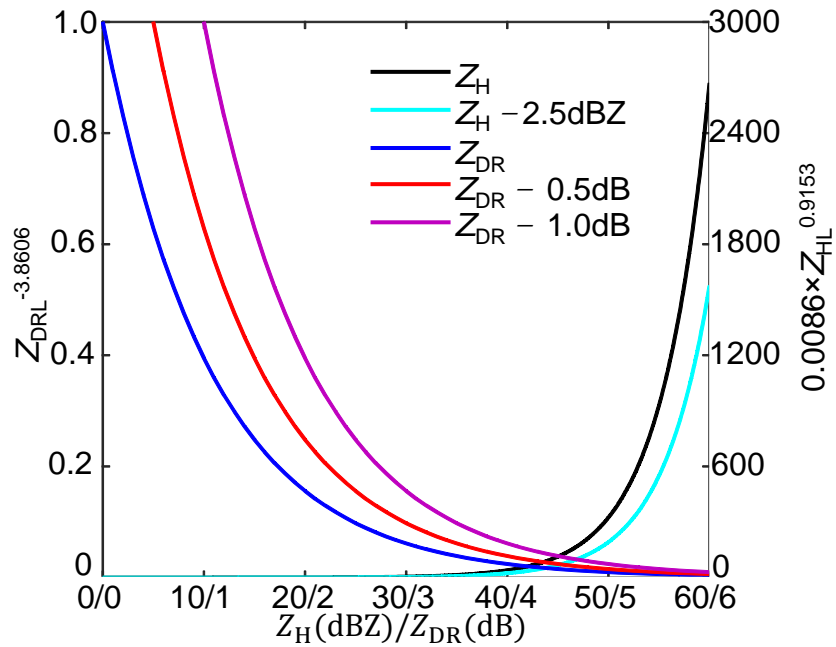
Fig. 23. The contribution of Z_H -related and Z_{DR} -related terms in the R(Z_H, Z_{DR}) relationship with different Z_H and Z_{DR} biases. The R(Z_H, Z_{DR}) relationship is detailed in Eq. 12c. Z_{HL} and Z_{DRL} refer to Z_H and Z_{DR} at a linear scale.
