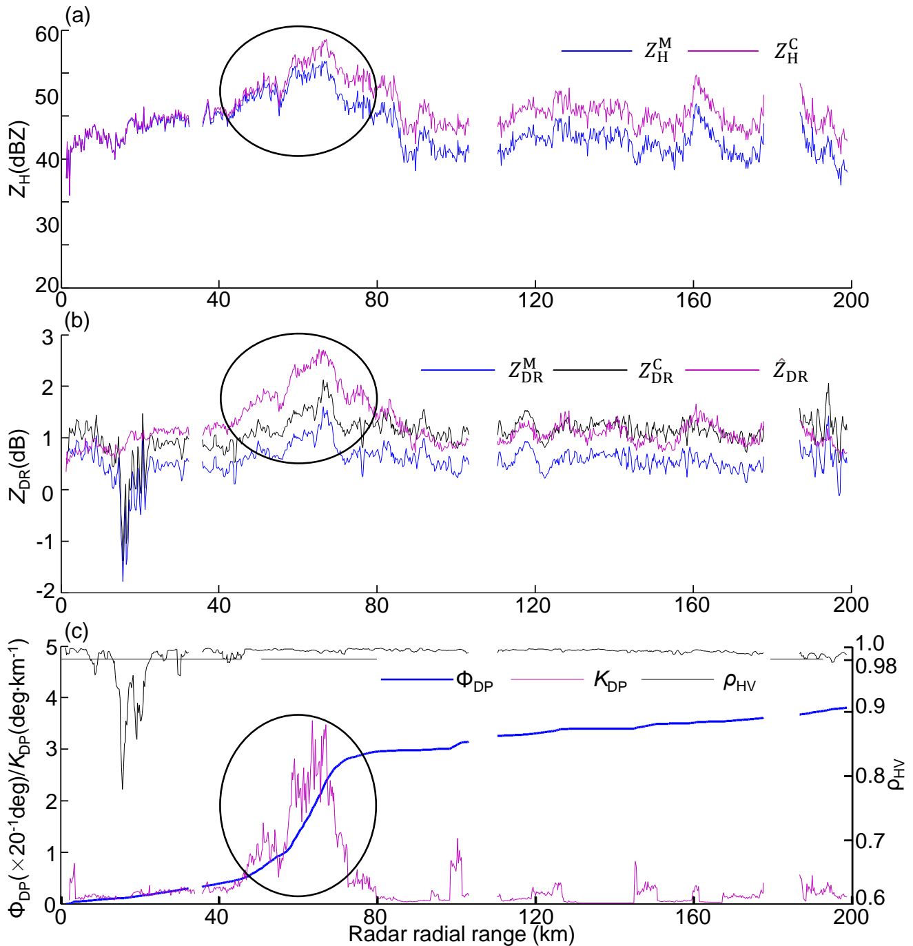
Fig. 18. WZ-SPOL radar along a radial profile (azimuth angle = 46^\circ ) at an elevation angle of 0.5^\circ at 1759 UTC, 09 August 2019: (a) Z_H^C and Z_H^M , (b) Z_{DR}^M , Z_{DR}^C and \hat{Z}_{DR} , (c) \Phi_{DP} , K_{DP} , and \rho_{HV} . This azimuth angle is marked in Fig. 11.
