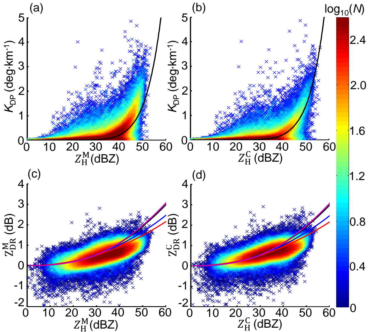
840 Fig. 9. The scattergram between polarimetric measurements from WZ-SPOL radar: (a) K_{DP} vs Z_H^M ; (b) K_{DP} vs Z_H^C ; (c) Z_{DR}^M vs Z_H^M ; (d) Z_{DR}^C vs Z_H^C . Measurements of all six stations derive the black curves; the blue, red, and purple curves in (c) and (d) stand for Eqs.11a-11c derived from S_I - S_{III} .
