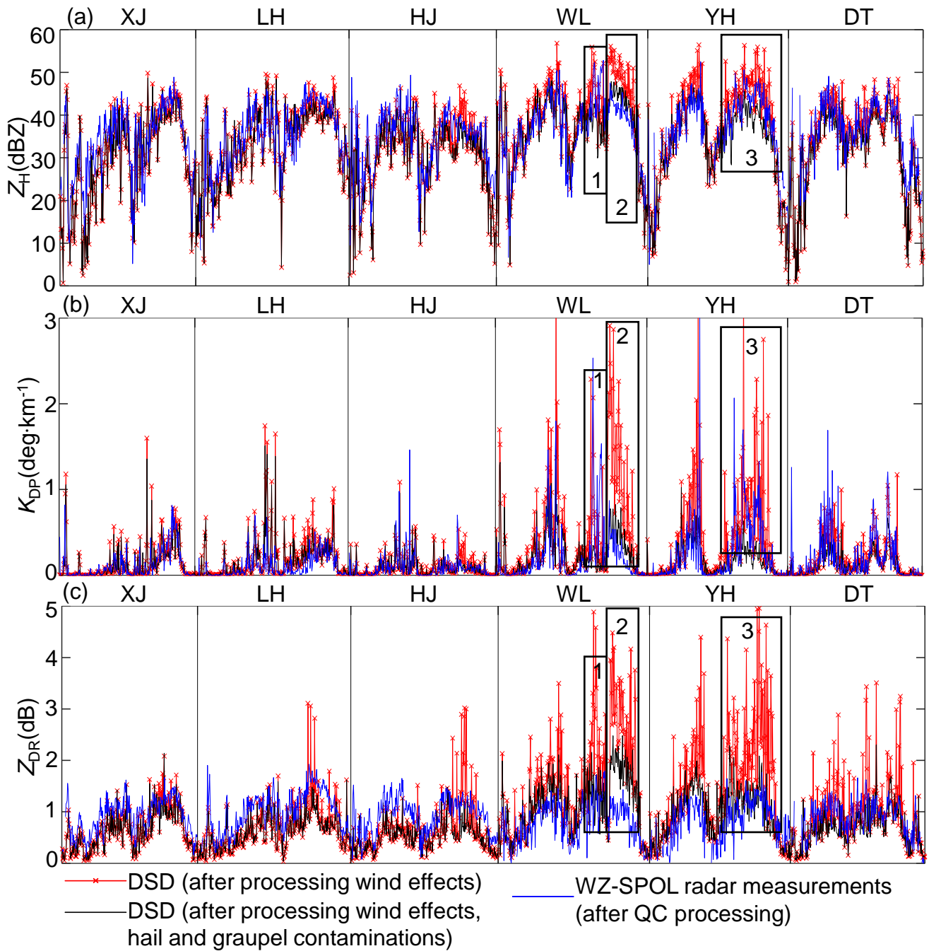
845 Fig. 10. (a) Time series of radar-measured Z_H^C and DSD-derived Z_H at the six meteorological stations shown in Fig. 6 during 2200 UTC 08 August 2019 and 0400 UTC 10 August 2019; (b) Similar to (a), but for radar-measured K_{DP} and DSD-derived K_{DP} ; (c) Similar to (a), but for radar-measured Z_{DR}^C and DSD-derived Z_{DR} .
