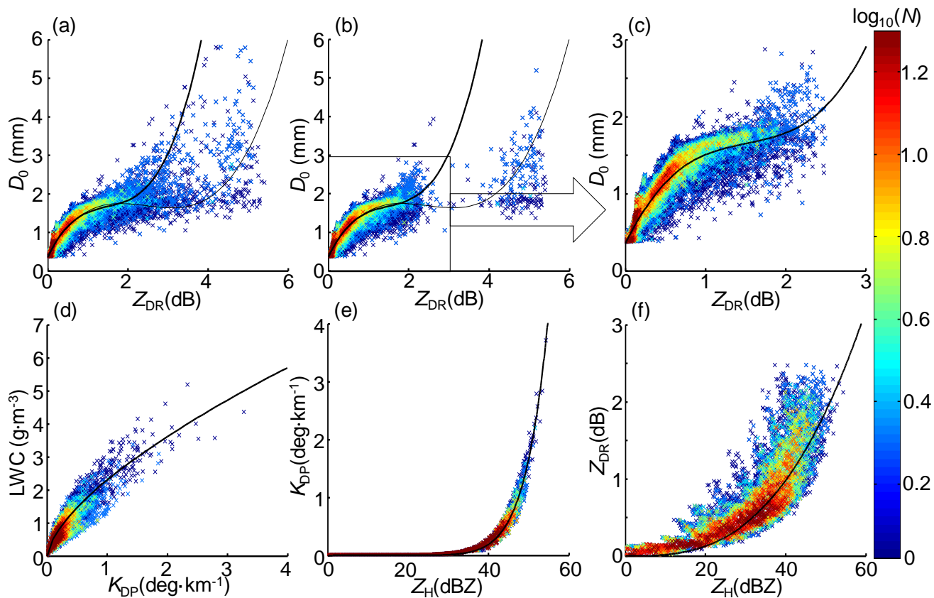
835 Fig. 8. Scattergrams between polarimetric radar variables: (a) D_0 vs. Z_{DR} after eliminating wind contaminations. (b) is based on (a), but after removing the hail and graupel contaminations further. (c) is based on (b), but after further eliminating the residual graupel contaminations with Z_{DR} > 2.5 dB. (d), (e) and (f) are LWC vs. K_{DP} , K_{DP} vs. Z_H , and Z_{DR} vs. Z_H based on the same dataset as (c). The thick black lines in (a)-(c) stand for Eq. 5; the thin black lines in (a) and (b) indicate the overfitted results, and the black curves in (d)-(f) stand for Eq. 6, Eq. 7 and Eq. 2a, respectively.
