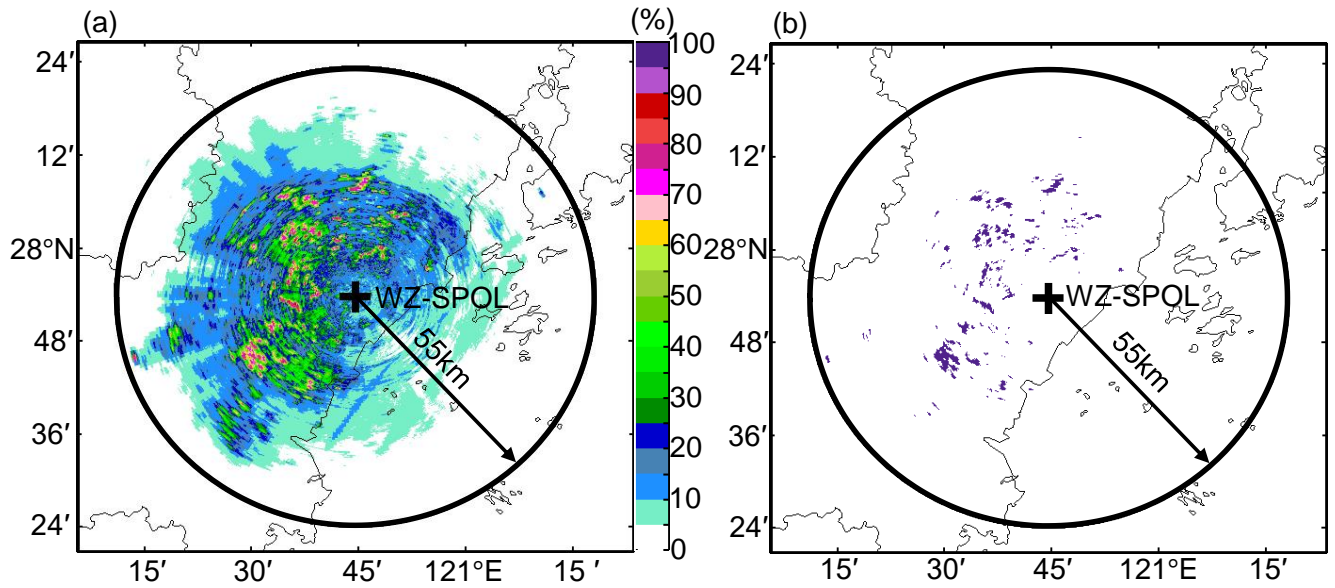
815 Fig. 3. (a) Statistics of pixels with Z_H > 0 dBZ within 55 km from the WZ-SPOL radar; (b) residual static ground clutter mask of the WZ-SPOL radar.
