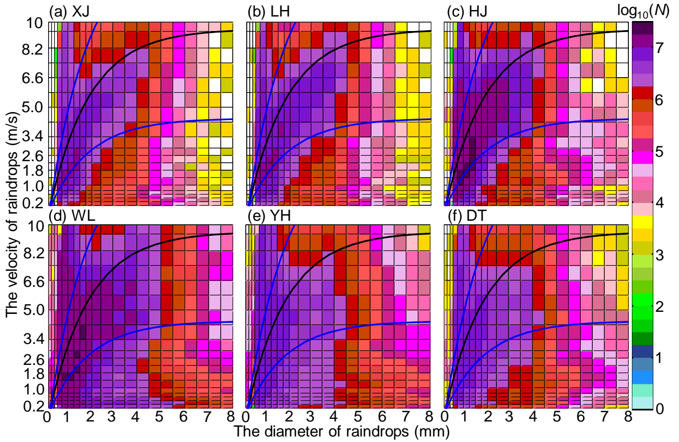
Fig. 5. The original size–velocity dataset collected at (a) XJ, (b) LH, (c) HJ, (d) WL, (e) YH, and (f) DT. The black and blue lines refer to the fall speed V_B , 0.5V_B , and 1.5V_B calculated in Eq. 3, respectively.
