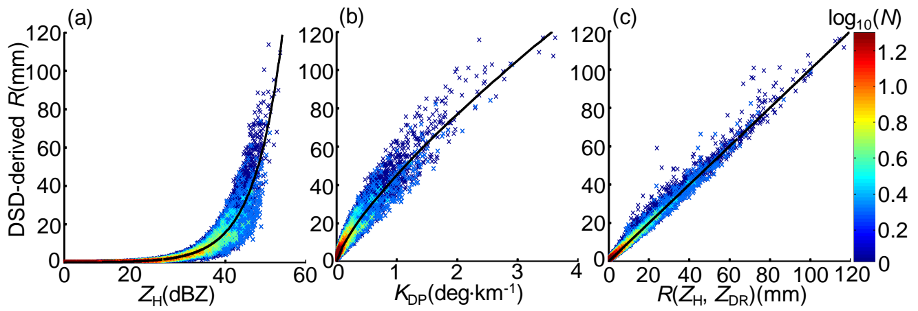
Fig. 20. The scattergram of (a) DSD-derived R vs. Z_H , (b) DSD-derived R vs. K_{DP} , and (c) DSD-derived R vs. R estimated by fitted R(Z_H, Z_{DR}) .
