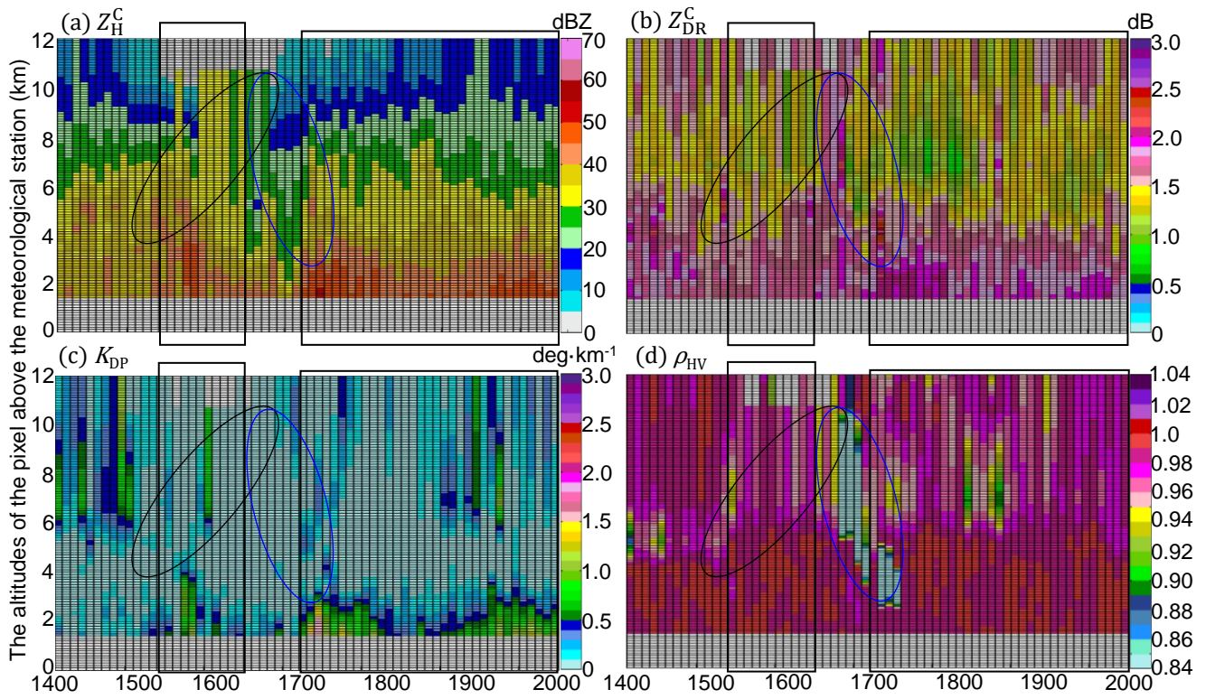
860 Fig. 13. Same as Fig. 12 but for the YH station.
