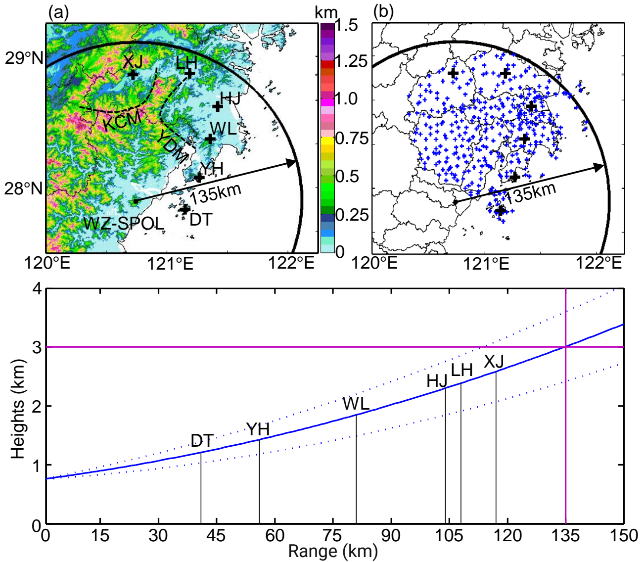
800 Fig. 2. (a) Terrain elevation and disdrometer network around the WZ-SPOL radar (735 m); (b) rain gauge network around the 805 disaster center area; (c) the height of radar beam shown as a function of measurement range in standard atmospheric conditions. Two dashed lines refer to the GWS of YDM and KCM. The black “+” in (a) and (b) refer to six national meteorological sites and the blue “+” in (b) refers to regional meteorological sites. The solid and dotted blue curves in (c) refer to the height of the radar beam center and its radius boundaries; the vertical black lines mark the range distance of national meteorological stations (heights<0.1 km) from radar; two orthogonal purple lines refer to the altitude of 3 km and range of 135 km.
