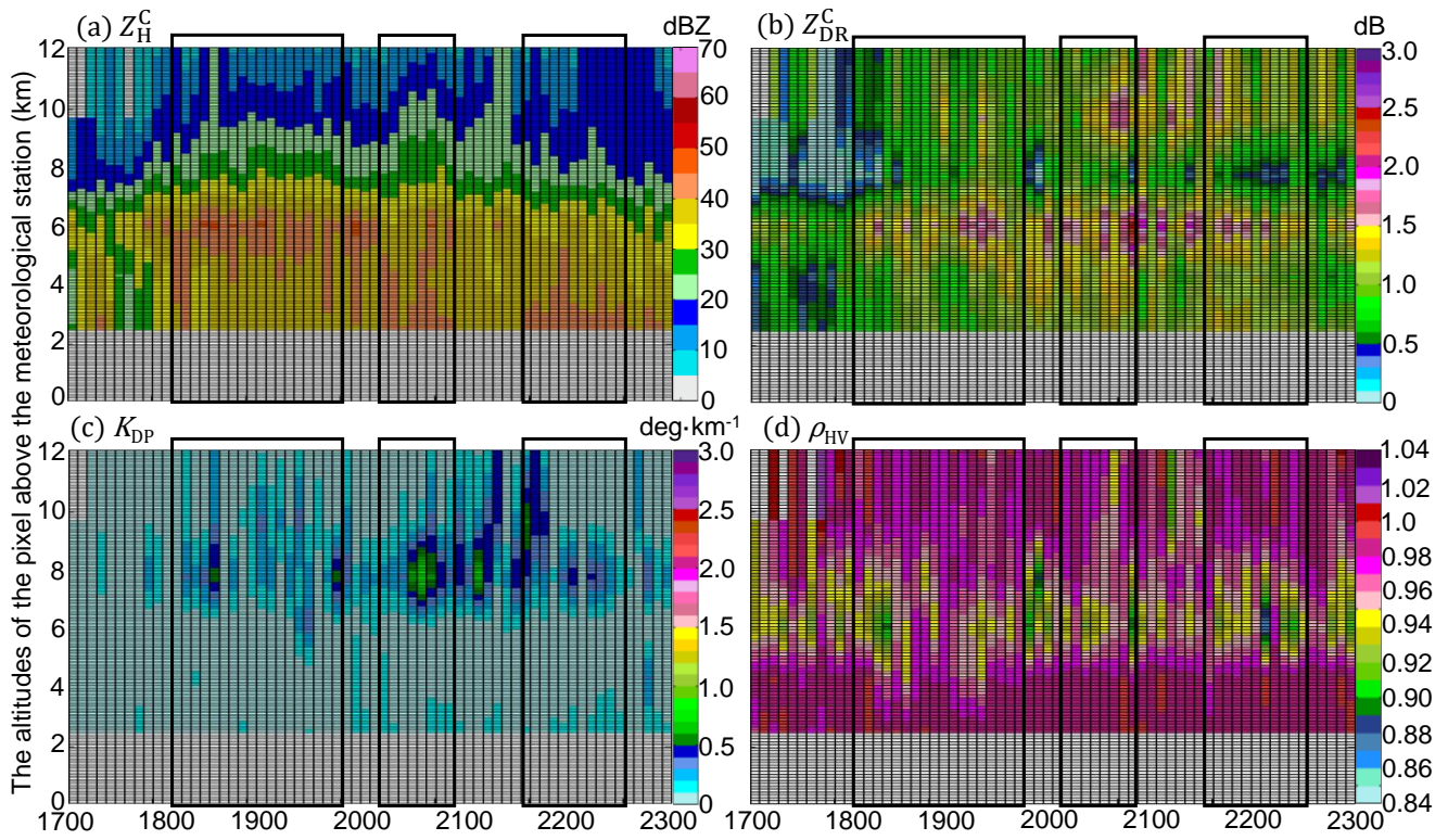
870 Fig. 17. Same as Fig. 12 but for the XJ station between 1500 UTC 08 August 2019 and 2100 UTC 09 August 2019.
