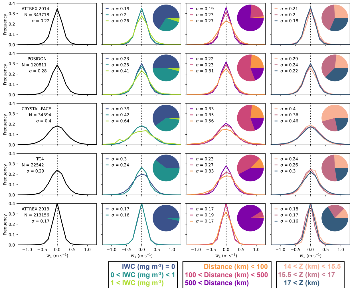
Figure 3. First column: Distributions of 1 Hz mean vertical wind ( \bar{w}_1 ) for all-corrected data from all campaigns, shown in separate rows. Campaign names and the number of 1 Hz samples are overlaid given in the leftmost column. Second, third and fourth columns show the same thing split the data into brackets-categories (relative frequencies are shown in pie charts) based on IWC, distance from deep convection, and height in the TTL, respectively. Sigma values for Standard deviations of fitted normal distributions ( \sigma ) are overlaid printed on all panels. Pie charts showing the distribution of brackets are overlaid on columns 2-4.
