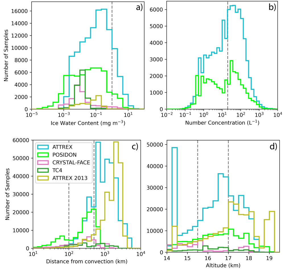
Figure B1. Histogram of (top-to-bottom) IWC, b) NI, c) distance from deep convection and d) altitude for all flight campaigns separately. Dotted NI is only shown for ATTREX 2014 and POSIDON. Dashed grey lines indicate bracket-boundaries used in the study to define categories.
