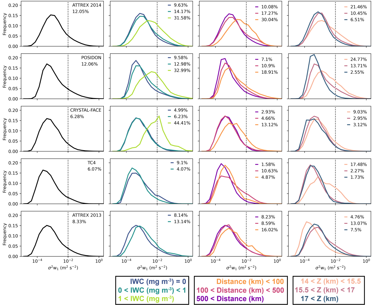
Figure 4. Same as Figure 2-3 except showing distributions of sub-high frequency (> 1 Hz) vertical wind variance ( \sigma_1^2 \sigma^2 w_1 ). The percentage of data exceeding the turbulent threshold ( 0.01 \text{ m}^2 \text{ s}^{-2} , vertical dotted line) is overlaid for each category is printed on each plot.
