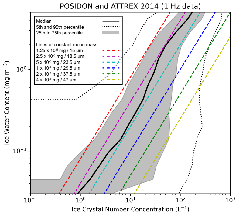
Figure 2. Statistics of ice crystal number concentrations–water content (NI, left plot/IWC) and relative humidity with respect to ice ( RH_i , right plot), are shown as a function of IWC–crystal number concentration (NI) for 1 Hz data from POSIDON and ATTREX 2014. The solid line is the median, the dotted lines are the 5th and 95 percentiles, and the shaded area spans the range of the 25th to 75th percentiles. Colored dashed lines indicate constant mean particle mass. The legend lists the mean masses and the corresponding mean equivalent sphere radii for each colored line.
