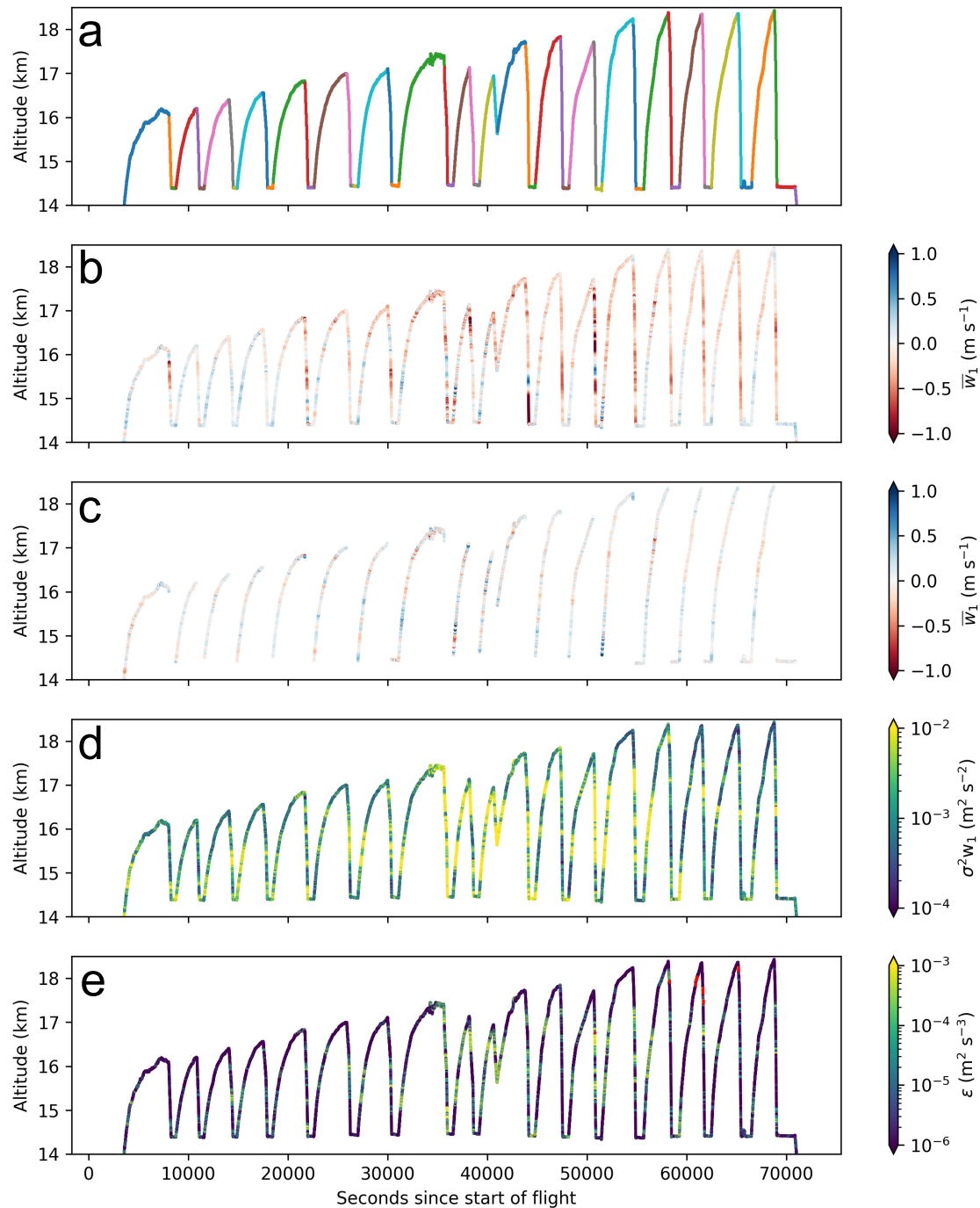
Figure A1. Flight tracks from a flight during ATTREX 2014 shown in time-height space with the color indicating a) different flight legs b) uncorrected mean 1-second uncorrected vertical wind ( \bar{w}_1 ), and Cc ) mean 1-second corrected vertical wind ( \bar{w}_1 ) d) variance in 1-second high frequency (> 1 Hz) vertical wind variance ( \sigma^2 w_1 ) and e) turbulent eddy dissipation rate ( \epsilon ). Outliers in \epsilon are shown in red.
