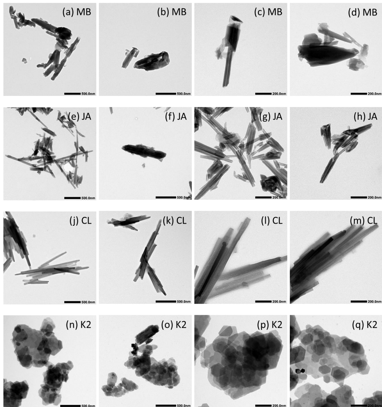
Figure 9: Transmission electron microscopy (TEM) micrographs of untreated samples at two different magnifications (see length bars within the images. Dust sample codes are identical to those in Fig. 2).
