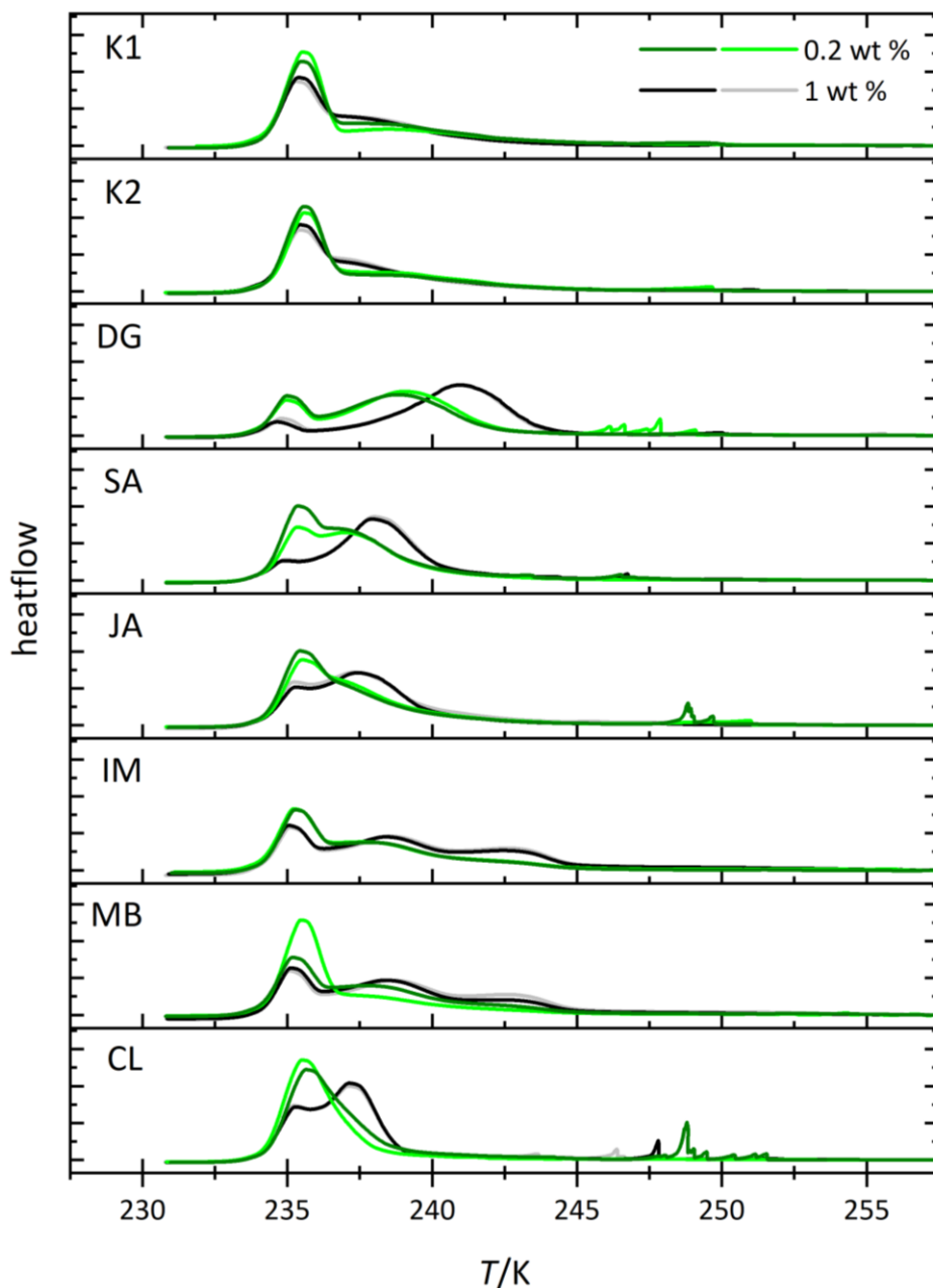
Figure 2: Thermograms from immersion freezing experiments of emulsified kaolinite samples (uppermost two panels) and halloysite samples (lower panels). The DSC was operated at a cooling rate of 1 \text{ K min}^{-1} . Black and grey lines: 1.0 wt % dust suspensions. Dark and light green lines: 0.2 wt % dust suspensions. The curves are normalized with respect to their total integral. Spikes occurring before the heterogeneous freezing signal originate from single large emulsion droplets and are not representative of ice nucleation by halloysite/kaolinite. Dust sample codes for kaolinites: K1 = KGa-1b (“well-ordered” kaolinite); K2 = KGa-2 (“poorly-ordered” kaolinite). Dust sample codes for halloysites: DG = Dragonite (Dragon Mine, Utah, USA); SA = Sigma Aldrich (Utah, USA); JA = Jarrahdale (Western Australia); IM = I-Minerals (Idaho, USA); MB = Matauri Bay (New Zealand); CL = Camel Lake (South Australia). See Table 1 for morphological and compositional details.
