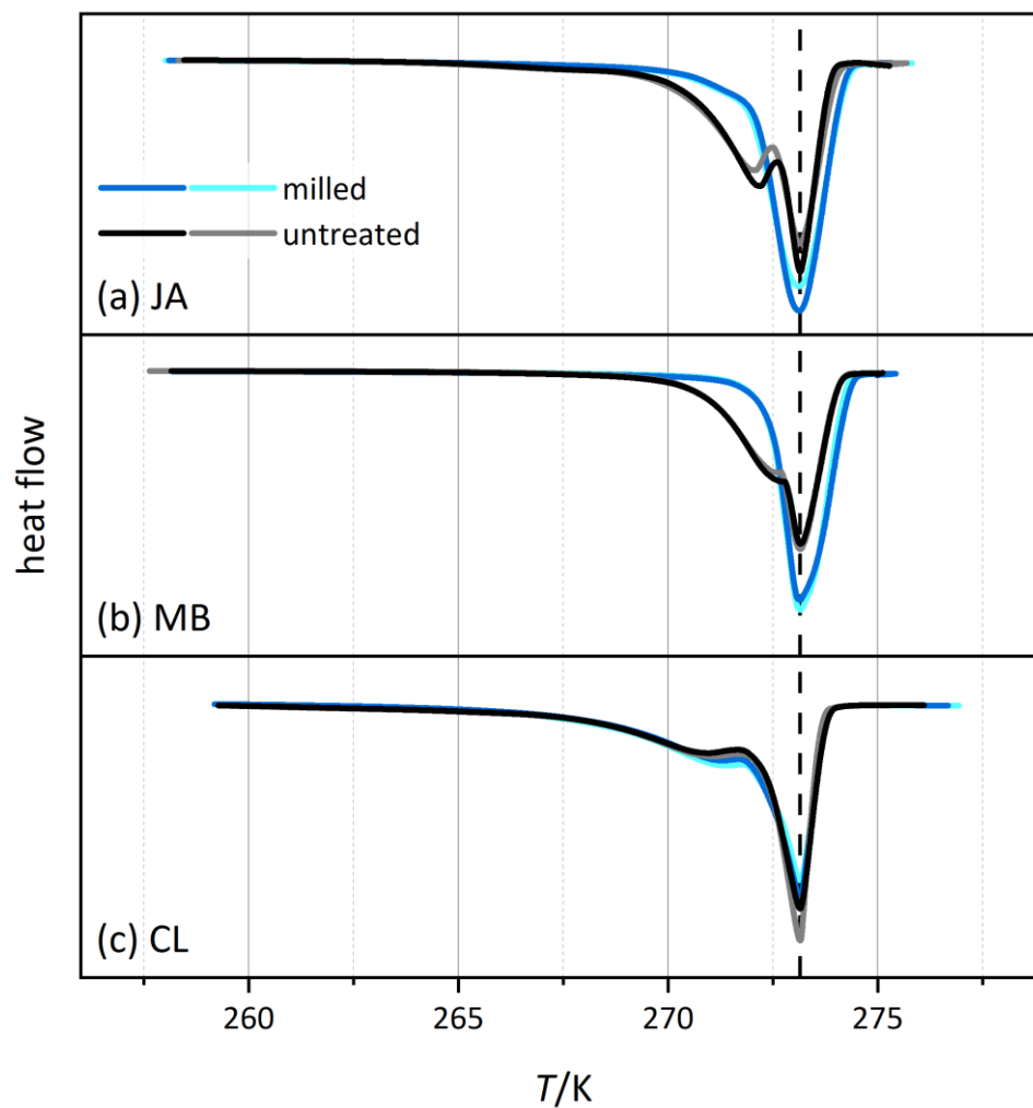
Figure 6: Thermograms from melting experiments of slurries of selected halloysite samples (black/grey) and the corresponding measurements of the milled samples (blue/cyan). The curves are normalized with respect to their total integral. Dust sample codes are identical to those in Fig. 2.
