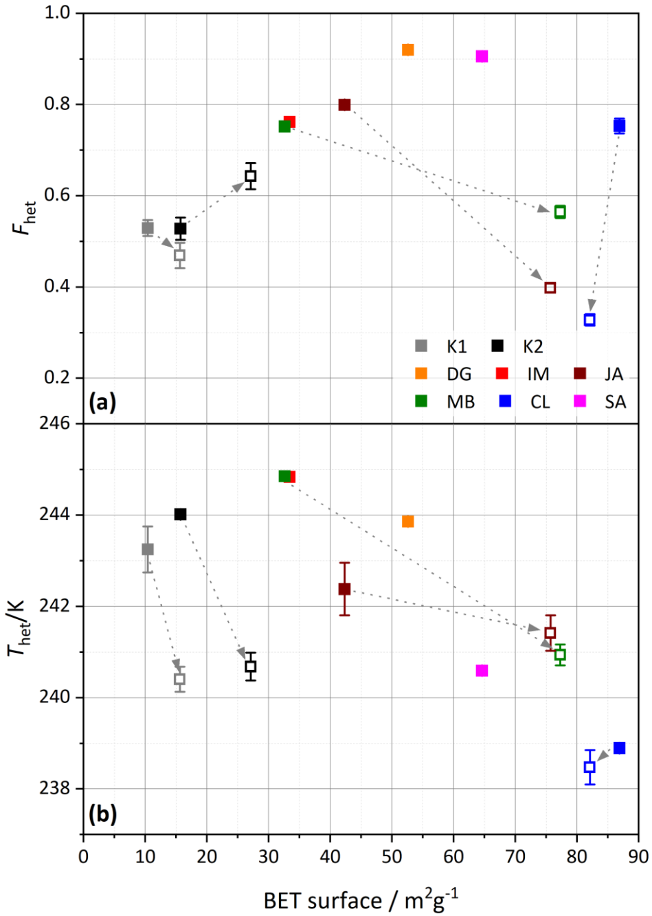
485 Figure 12: Similar as Fig. 11, (a) F_{\text{het}} and (b) T_{\text{het}} , but here plotted against the BET surface area derived from DVS measurements (analysed between 15–35 % RH). Filled symbols depict untreated and open symbols milled samples. The samples are colour coded as indicated by the legend in the top panel. The dashed arrows point from the untreated sample to the corresponding milled sample. Dust sample codes are identical to those in Fig. 2.
