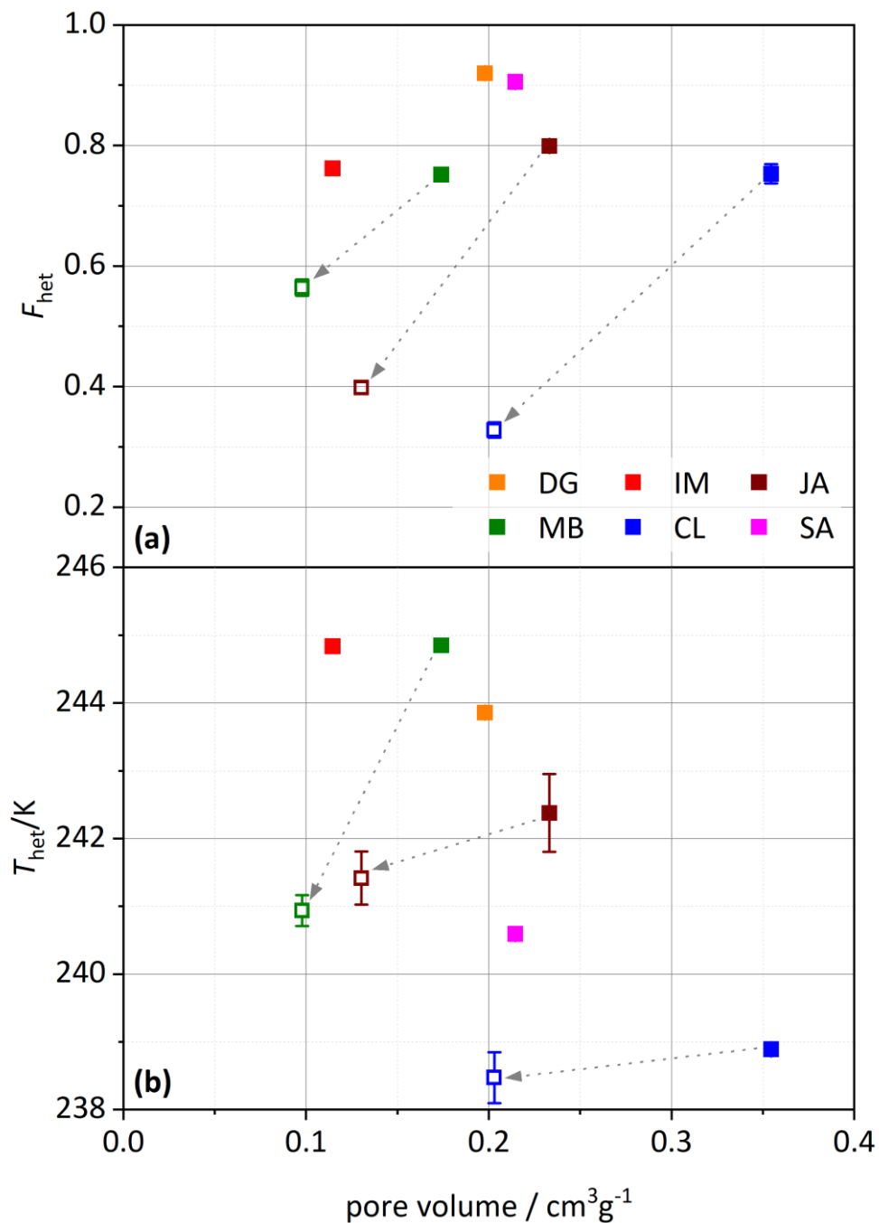
480 Figure 11: (a) Heterogeneously frozen fraction, F_{\text{het}} , and (b) heterogeneous freezing onset temperature, T_{\text{het}} , plotted against the specific pore volume calculated from DVS measurements (analysed between 40–98 % RH). Filled symbols depict untreated and open symbols milled samples. The dashed arrows point from the untreated to the corresponding milled sample. Dust sample codes are identical to those in Fig. 2.
