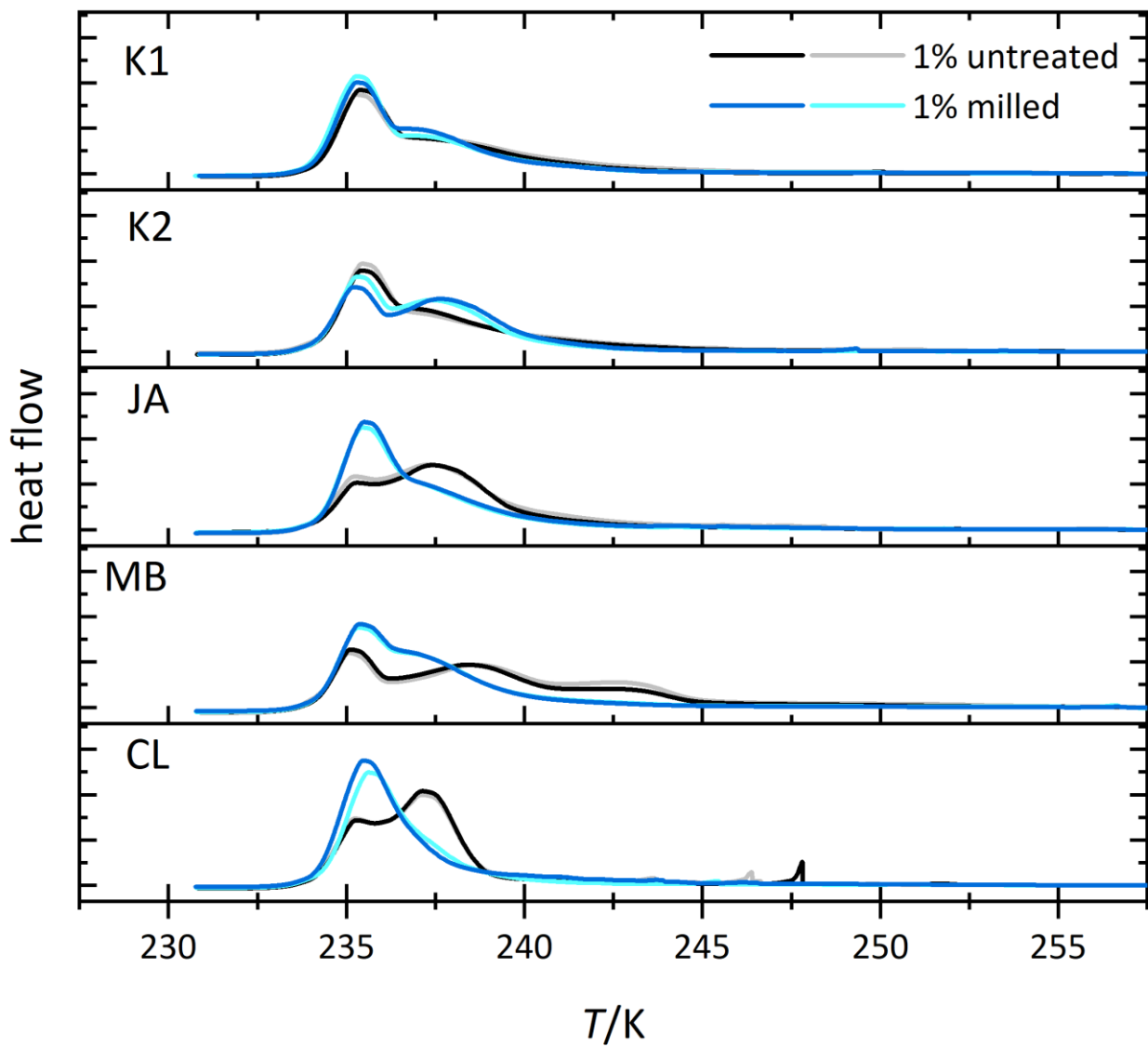
335 Figure 4: Thermograms from immersion freezing experiments of emulsified 1 wt % dust suspensions of kaolinites and selected halloysite samples (black/grey) and the corresponding measurements of the milled samples (blue/cyan). The curves are normalized with respect to their total integral. (Spikes occurring before the heterogeneous freezing signal originate from single large emulsion droplets and are not representative of ice nucleation by halloysite/kaolinite). Dust sample codes are identical to those in Fig. 2.
