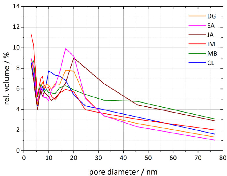
Figure 7: Pore size distributions for each of the six halloysite samples resulting from DVS isotherms analysed between 35 and 98 % RH. Plotted is the relative pore volume against the pore diameter (calculated using Eq. 1 in Sect. 3.3). Dust sample codes are identical to those in Fig. 2.
