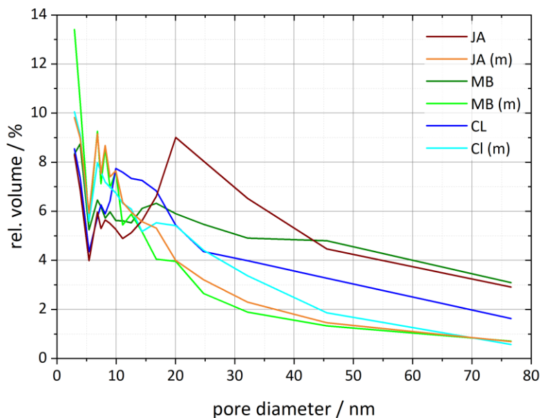
405 Figure 8: Pore size distributions for selected halloysite samples and their corresponding milled samples resulting from DVS isotherms analysed between 35 and 98 % RH (calculated using Eq. 1 in Sect. 3.3). Dust sample codes are identical to those in Fig. 2.
