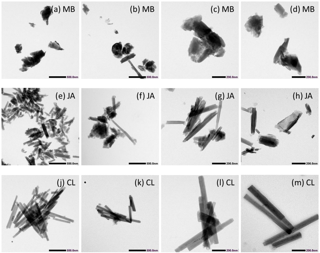
445 Figure 10: TEM micrographs of milled samples at two different magnifications (see length bars within the images. Dust sample codes are identical to those in Fig. 2).
