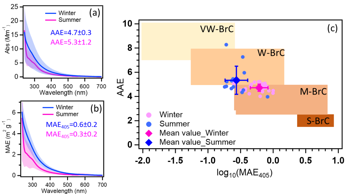
Figure 2. The average Abs (a) and MAE (b) of MS-BrC in winter (blue) and summer (pink). (c) Graphical representation of optical-based BrC classes in AAE- \text{Log}_{10}(\text{MAE}_{405}) space with summer and winter data (Saleh, 2020; Hettiyadura et al., 2021). VW-, W-, M-, and S-BrC, are very weakly absorbing-, weak absorbing-, moderately absorbing-, and strongly absorbing-BrC. AAE reported in this work is calculated for a wavelength range of 300 – 450 nm. Please note that the small shoulder peak at \sim 300 nm for the average summer sample (a & b) is most likely due to some contaminations e.g. from the filter. However, it only occurred in a few filter samples and does not affect our main results.
