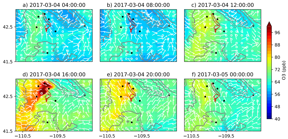
Figure 9. The formation and dissipation of O 3 concentrations over the basin using MOZART chemistry with dry-deposition of gas species turned off (MOZ_ddOff) for the O 3 event on Mar 04, 2017, starting at 04:00 and ending at 24:00, with an interval of four hours in two consecutive figures. All times in the figure are in local time (UTC - 7 hours). The black dots are the location of the seven WYDEQ stations, and the red outline is an approximate location of the PAJF development.
