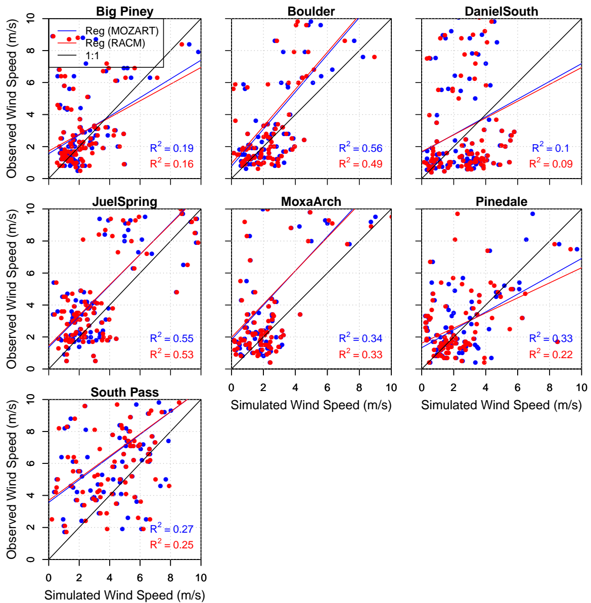
Figure 4. Similar to Figure 3 but for wind speed.
