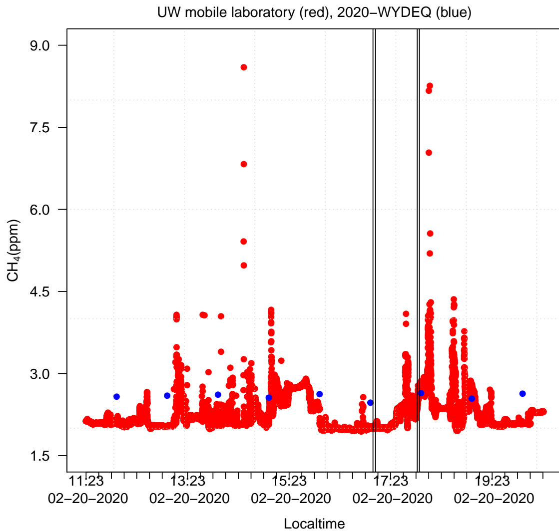
Figure A1. Time series comparison of CH 4 from the UW mobile laboratory (red) and WYDEQ Boulder site (blue) for Feb 20, 2020. The black vertical lines mark the times when the mobile laboratory was passing through the WRF grid box where the WYDEQ Boulder site is located.
