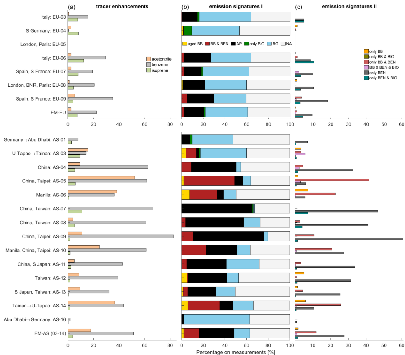
Figure 4: Fractions [%] of (a) enhancements over thresholds observed in acetonitrile, benzene and isoprene, (b) source signatures I ( aged BB , BB & BEN and AP * inferred from observed enhancements only in acetonitrile and benzene; only BIO and BG * inferred with additional isoprene) and (c) source signatures II (inferred from observed enhancements in acetonitrile, benzene and isoprene). Top: EMERGE-Europe, bottom: EMERGE-Asia. EU-05 is not available due to instrument failure. The summary of EMERGE-Asia excludes the non-Asian transfer flights AS-01 and AS-16.
