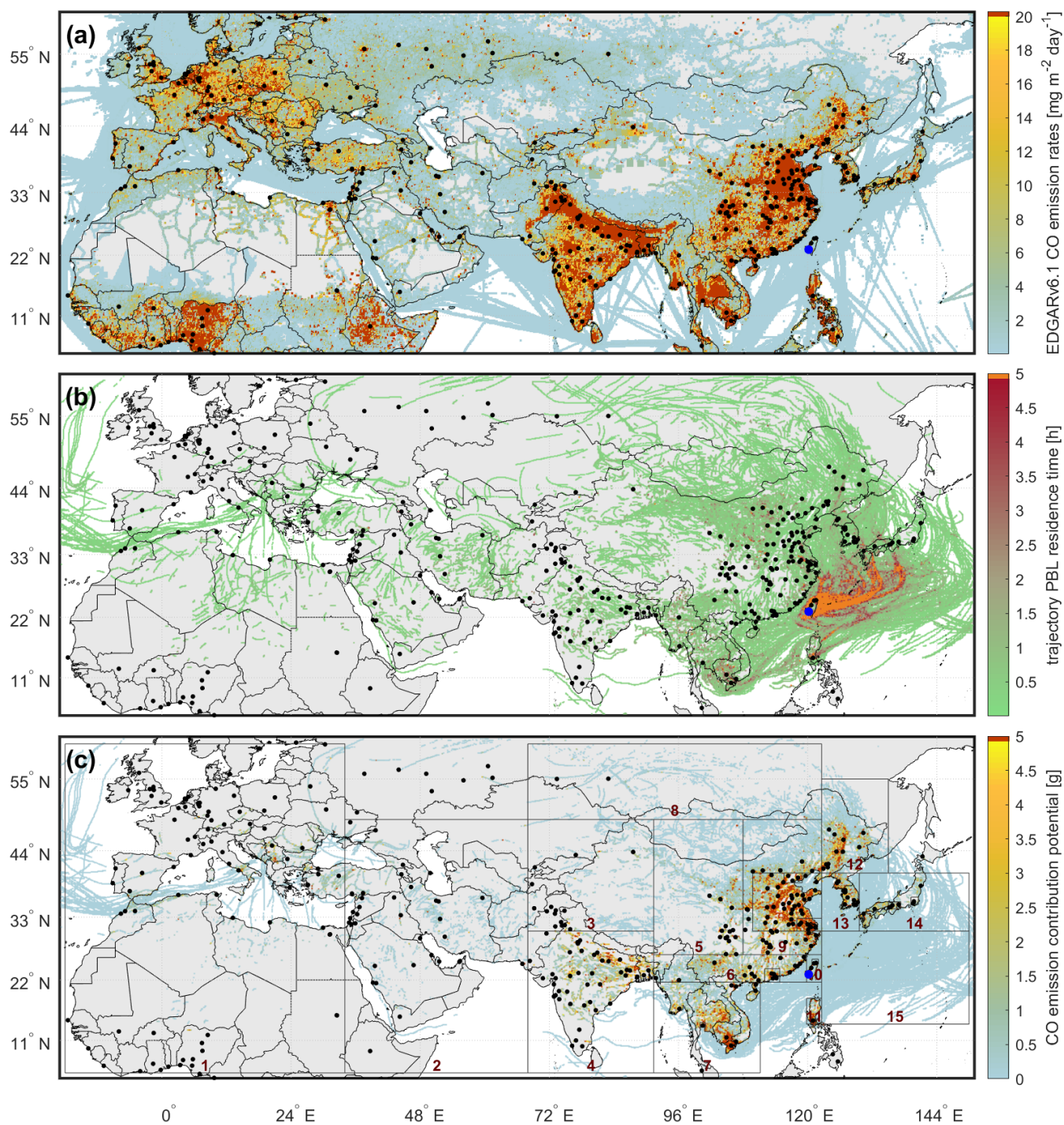
405 Figure 6: (a) EDGARv6.1 CO emission rates from anthropogenic sources (March 2018), for clarity, not colour-coded below 0.01 \text{ mg m}^{-2} \text{ day}^{-1} , (b) PBL residence time of air parcels (for flights AS-03 to AS-14) cumulated for a grid resolution of 0.1^\circ \times 0.1^\circ , (c)
