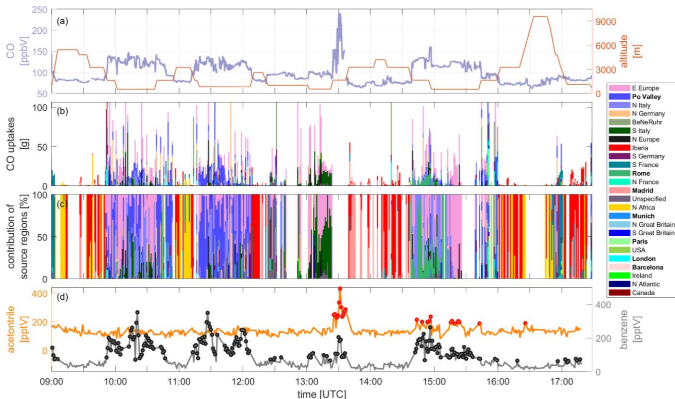
565 Figure 9: Time series of modelled source region specific CO uptakes and measured CO, acetonitrile and benzene for EMeRGe-Europe flight EU-06, 20 July 2017, targeting Italian outflows. (a) CO measurements and flight altitude, (b) modelled CO uptake sums along 10-days back trajectories colour-coded by originating source regions (sorted by total flight uptake sums – top to bottom, MPCs in bold), (c) relative contribution of source regions on CO uptake sums and (d) acetonitrile and benzene measurements with colour-coded tracer enhancements over defined threshold (red and black dots, respectively).
