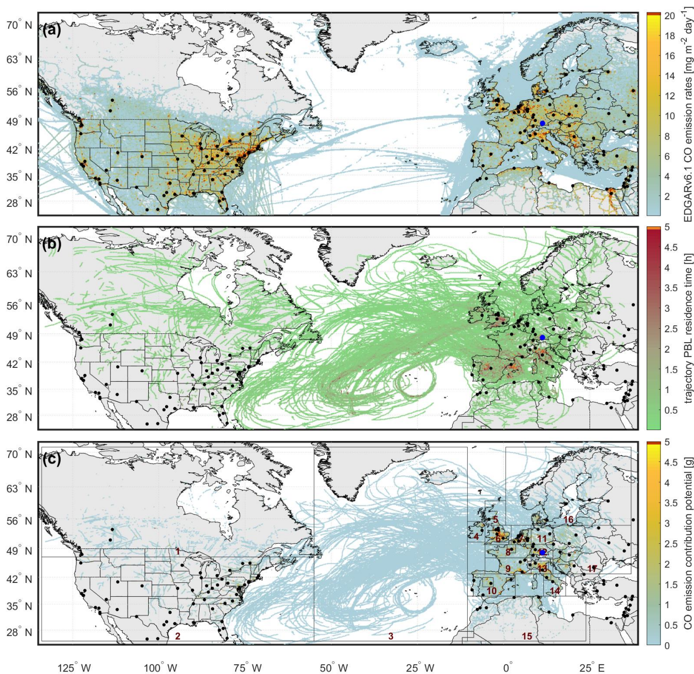
Figure 5: (a) EDGARv6.1 CO emission rates from anthropogenic sources (July 2018), for clarity, not colour-coded below 0.01 mg m -2 day -1 , (b) PBL residence time of air parcels cumulated for a grid resolution of 0.1° x 0.1°, (c) modelled CO emission uptake from the PBL interpreted as emission contribution potential during EMERGe-Europe. Boxes in (c) mark selected study areas (summarised in Table, left). Black dots mark cities with more than one million inhabitants, the blue dot denotes the home base of HALO (airport Oberpfaffenhofen near Munich, Germany) during EMERGe-Europe.
