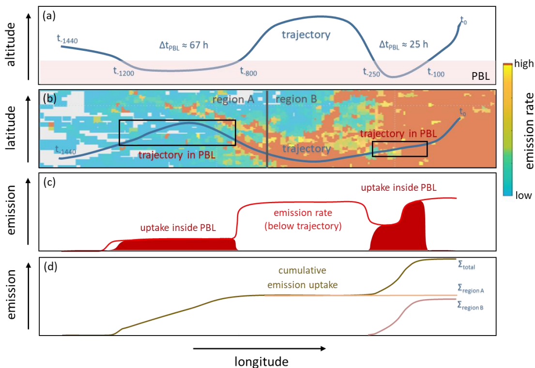
Figure 3: Graphical representation (simplified example) of our Lagrangian CO uptake model based on PBL height and trajectory pathways, with longitude as x-axis. (a) Trajectory altitude. An example trajectory (sampled by the aircraft at time t_0 ) enters the PBL for two different periods, between t_{1200} and t_{800} , as well as between t_{250} and t_{100} ( t_{100} means: 100 backward calculation steps = 1000 min = 16.7 h). During these periods, CO is taken up, that is, the trajectory is loaded with CO emitted on ground. (b) Geographic map: CO emission rates from EDGAR (shaded) with a trajectory (blue line) and rectangles in which the trajectory descends into the PBL. Exemplary, two example regions A and B are defined. (c) Time series: emission rate along the trajectory (red line) and CO uptake periods (filled red regions) along the trajectory. (d) Total and subtotal (region A and B) cumulative CO uptake (dark yellow line) along the trajectory.
