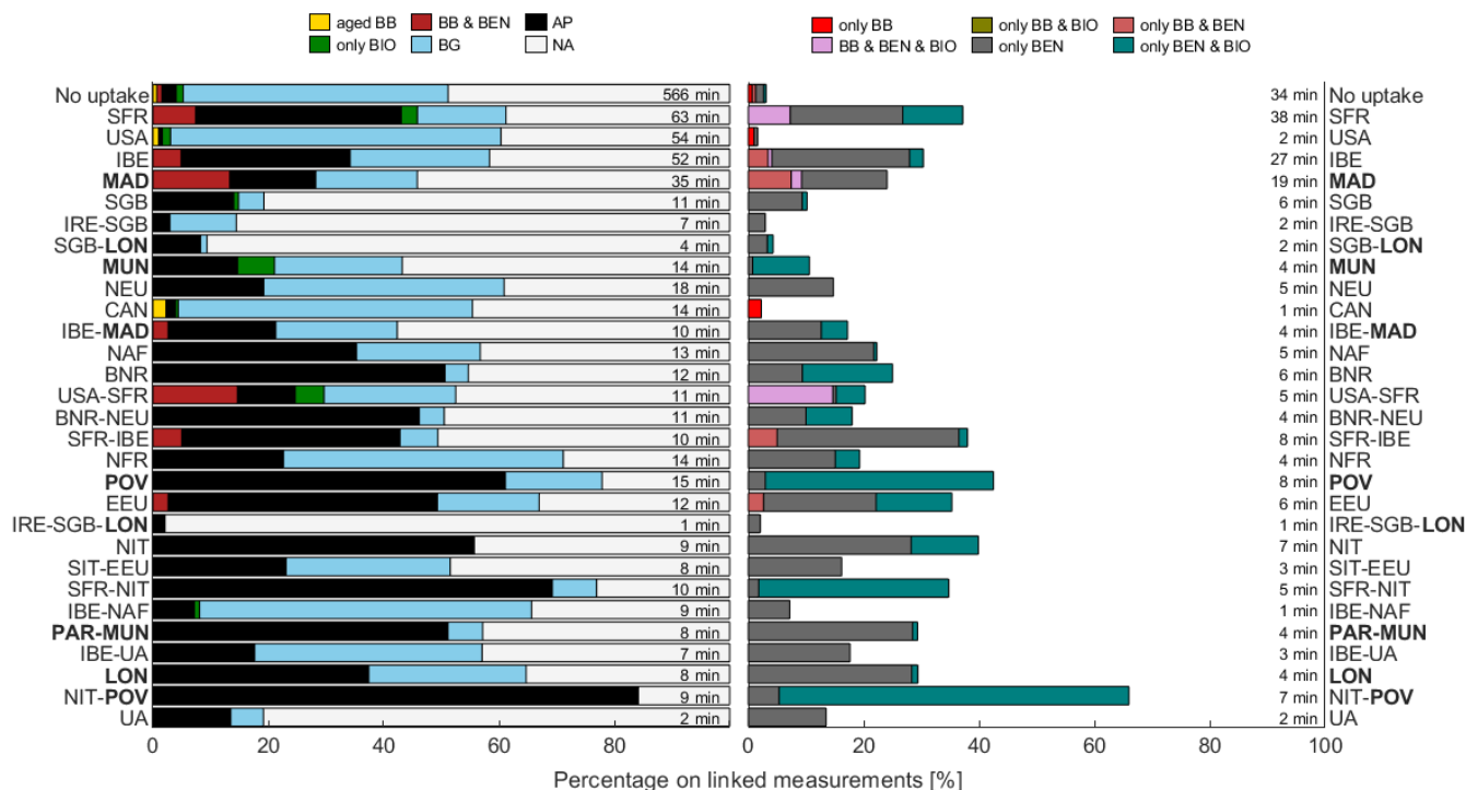
625 Figure 10: Source signatures* (I - left, and II – right, using the tracer acetonitrile, benzene and isoprene) of contributing regions as chemical fingerprints during EMERGe-Europe. The temporal contribution of identified signatures to the measurements is shown on the right-hand side of the bars and differ from signatures I to II due to the usage of two and three tracers, respectively. For full names of source regions see Table 4.
