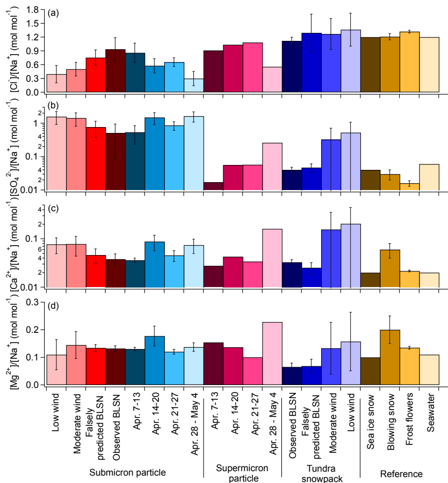
510 Figure 5. Average ( \pm 1\sigma ) [\text{Cl}^-]/[\text{Na}^+] , [\text{SO}_4^{2-}]/[\text{Na}^+] , [\text{Ca}^{2+}]/[\text{Na}^+] , and [\text{Mg}^{2+}]/[\text{Na}^+] molar ratios for submicron particles and local tundra surface snowpack for the categories of low wind, moderate wind, falsely predicted BLSN, and observed BLSN periods, and for multi-day supermicron particles collected on April 7-13 (65% observed BLSN, 35% falsely predicted BLSN), April 14-20 (9% observed BLSN, 29% falsely predicted BLSN, 58% moderate wind, 4% low wind), April 21-27
