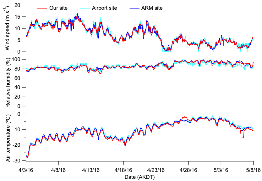
Figure S7. Measured air temperature, relative humidity, and wind speed at the Field Site, Wiley Post-Will Rogers Memorial Airport, and Department of Energy Atmospheric Radiation Measurement (ARM) Observatory. The measurement heights at the Field Site, Airport, and ARM Observatory were 10 m, 7 m, and 8 m above the ground, respectively.
