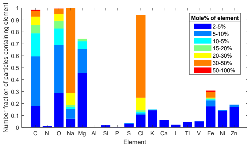
Figure S5. Digital color histogram of individual 0.4-2.8 \mu\text{m} d_p fresh sea spray aerosol particles, collected on aluminum foil. The digital color histogram heights represent the number fractions of individual sea spray aerosol particles containing a specific element, while the colors represent the mole percentage of that element in that number fraction of particles. Aluminum was removed from the EDX spectra due to contributions from the aluminum foil substrate.
