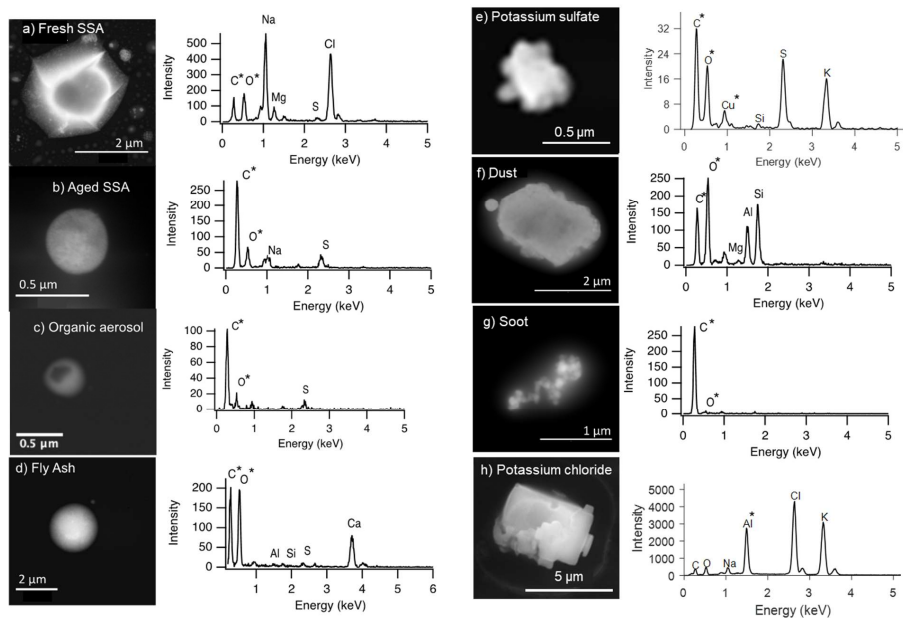
Figure S4. Representative SEM images and EDX spectra of the main particle types observed in April 6 and April 15-16 samples. The C, O, and Cu signals include contributions from the TEM grids in a-g, and the Al signal includes contributions from the aluminum substrate in h.
