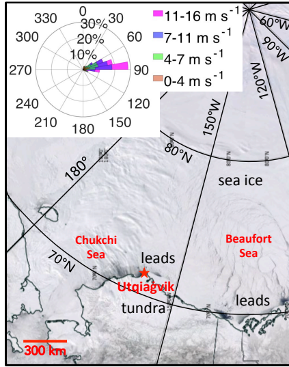
160 Figure 1. Image of the North Slope of Alaska and Beaufort and Chukchi Seas on April 6, 2016 from the Terra satellite Moderate Resolution Imaging Spectroradiometer (MODIS). The dark regions and cracks correspond to leads surrounded by sea ice. The inset plot depicts the percentage distribution of observed wind speeds and directions, measured at a 9.7 m height at the Utqiagvik tundra site from April 3 to May 7, 2016. This figure is modified from NASA Worldview 165 ( https://worldview.earthdata.nasa.gov/ ).
