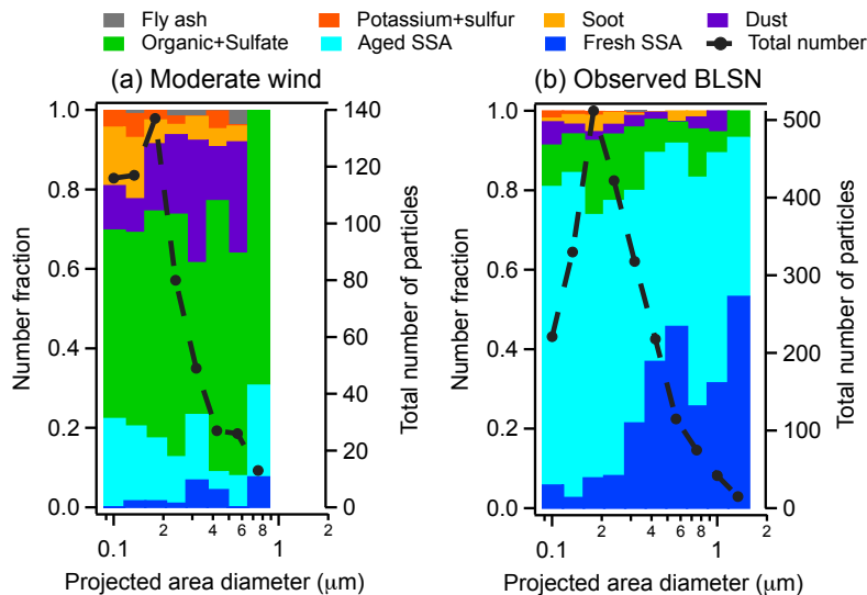
Figure 6. Number fractions of seven individual particle types identified by CCSEM-EDX analysis of stage 3 ( d_a 0.07-0.4 \mu\text{m} ) samples collected during (a) two moderate wind periods (April 15 19:00 – April 16 07:00 AKDT and April 16 08:00–20:00), and (b) two observed blowing snow periods (April 6 07:00–19:00 and April 6 19:00 – April 7 07:00). Total numbers of particles analyzed by CCSEM-EDX per size bin are also shown. SSA refers to sea spray aerosol. All particles were collected on the 0.07-0.4 \mu\text{m} d_a impactor stage; projected area diameters, measured by SEM are shown. Size-resolved counts of particles analyzed by CCSEM-EDX per sample are shown in Figure S3, and representative SEM images and EDX spectra of the particle types are provided in Figure S4.
