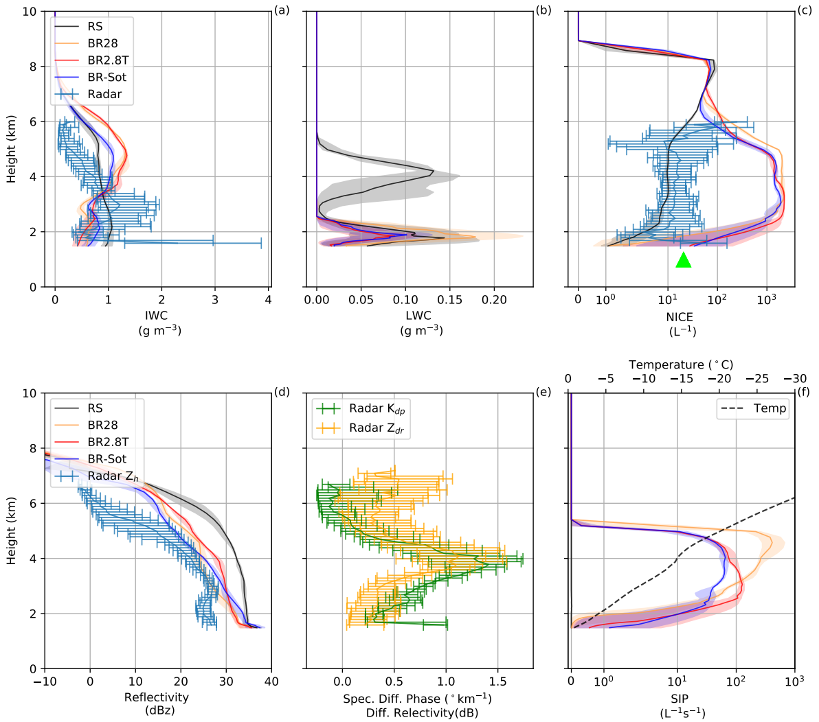
Figure 7. (a) Ice water content (IWC), (b) liquid water content (LWC), (c) ice number concentration (NICE), (d) model and radar reflectivity, (e) Specific differential phase ( K_{dp} ), differential reflectivity ( Z_{DR} ), and (f) secondary ice production (SIP). The solid lines are the mean with shaded areas and errorbars showing the 10th and 90th percentiles for the model simulations and Doppler radar respectively at 15:30 UTC. The green triangle is the 2DVD surface observations for hydrometeors D > 0.2 mm.
