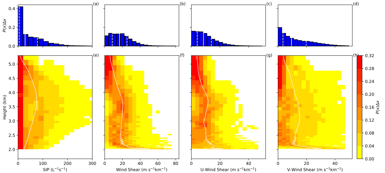
Figure 8. Probability density functions of different variables ( P(x) ) from the BR2.8T simulation from all model levels (top row) and at each model level (bottom row) for (a, e) Secondary Ice Production (SIP) rate, (b, f) Wind shear, (c, g) U-wind shear and (d, h) V-wind shear between 14:30-15:45 UTC. The solid and dashed white lines are the horizontal 50 th percentile and the 25 th and 75 th percentiles respectively of each variable over the 10 km \times 10 km domain.
