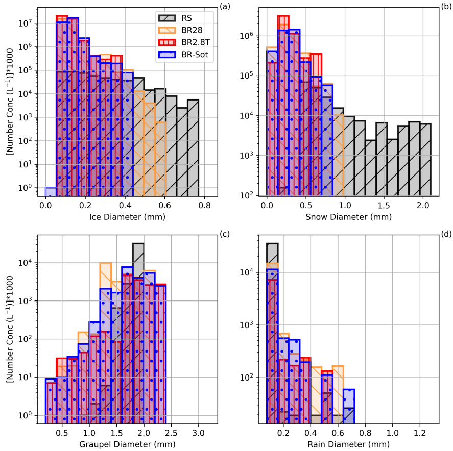
Figure 6. Particle size distribution over the number concentrations for panels (a) ice, (b) snow, (c) graupel and (d) raindrops for all the simulations at 15:30 UTC.
