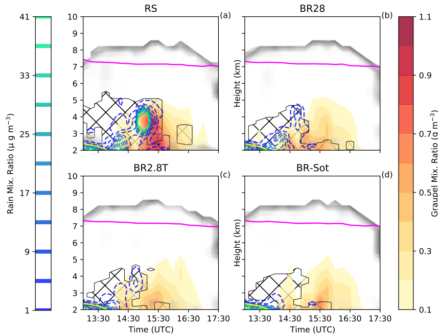
Figure 5. Hovmöller diagrams of graupel and rain mixing ratio for panels (a) RS , (b) BR28, (c) BR2.8T and (d) BR-Sot between 13:00 and 17:30 UTC. The hatched area is defined as the MPC where the cloud droplet mass concentration and ice mass concentration is greater than 10 and 0.1 \text{mg m}^{-3} respectively. The pink line is the homogeneous freezing line at -38^\circ\text{C} , and the shaded gray area is the cloud area fraction.
