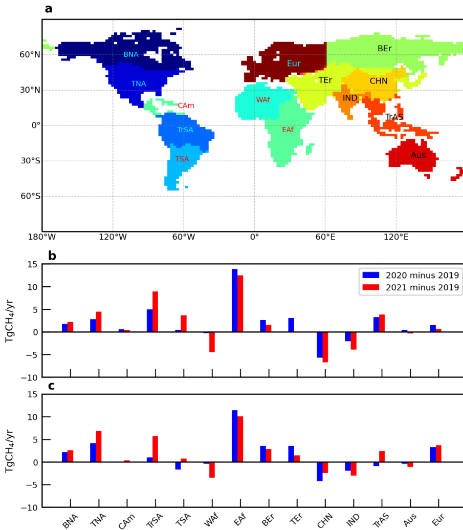
Figure 1 Large-scale geographical regions a) for which we report methane changes ( TgCH_4/yr ) in 2020 and 2021 b) differences between a posteriori emissions from 2020 and 2021 relative to inversion-specific baselines for 2019. Geographical regions, informed by TransCom-3 experiments (Gurney et al. 2004), include boreal North America (BNA), temperate North America (TNA), central America (Cam), tropical South America (TrSA), temperate South America (TSA), Europe (Eur), western Africa (Waf), eastern Africa (Eaf), boreal Eurasia (BEr), temperate Eurasia (TEr), India (IND), China (CHN), tropical Asia (TrAs), and Australia (Aus). Panel c) is the same as b) but for a posteriori methane emission from the joint methane-OH inversion.
