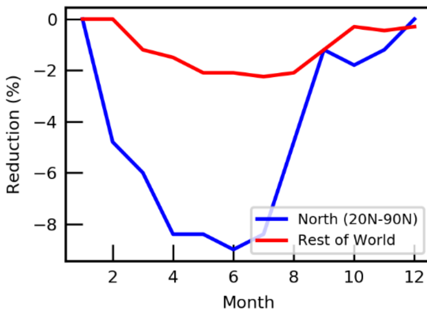
55 Figure A1 Assumed temporal distribution for OH reduction (%) in the northern hemisphere (20°N-90°N, blue line) and the rest of the world (red line) for our sensitivity calculation.
