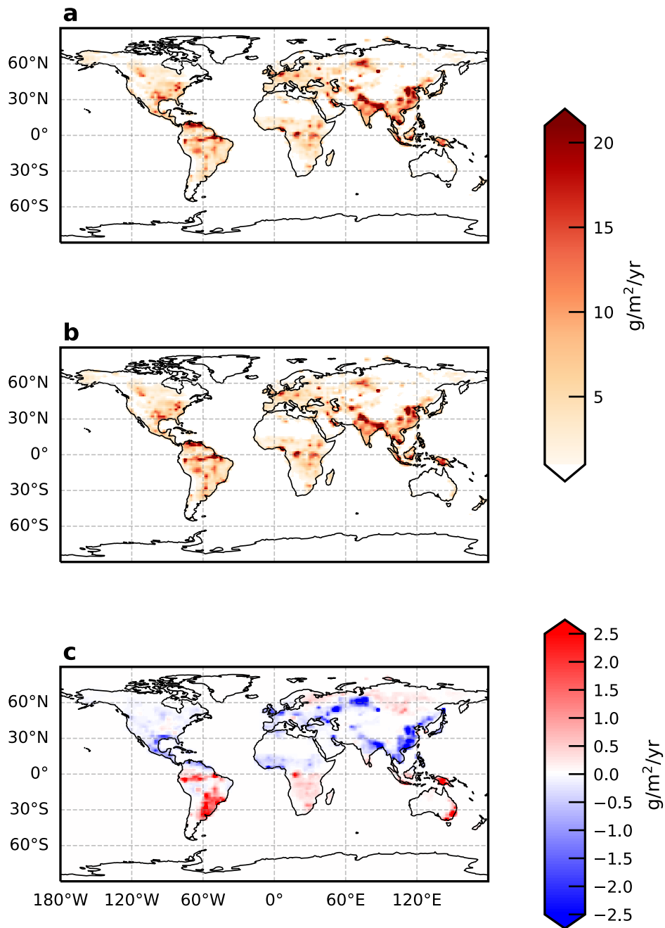
60 Figure A3 Global a posteriori emissions of methane ( \text{g/m}^2/\text{yr} ) inferred from GOSAT methane: \text{CO}_2 column ratio data for the baseline year of 2019, corresponding to a OH climatology (Feng, Palmer, Zhu, et al. 2022) and b the joint methane-OH inversion. Panel c shows the difference of a posteriori emissions of methane corresponding to joint methane-OH inversion minus OH climatology.
