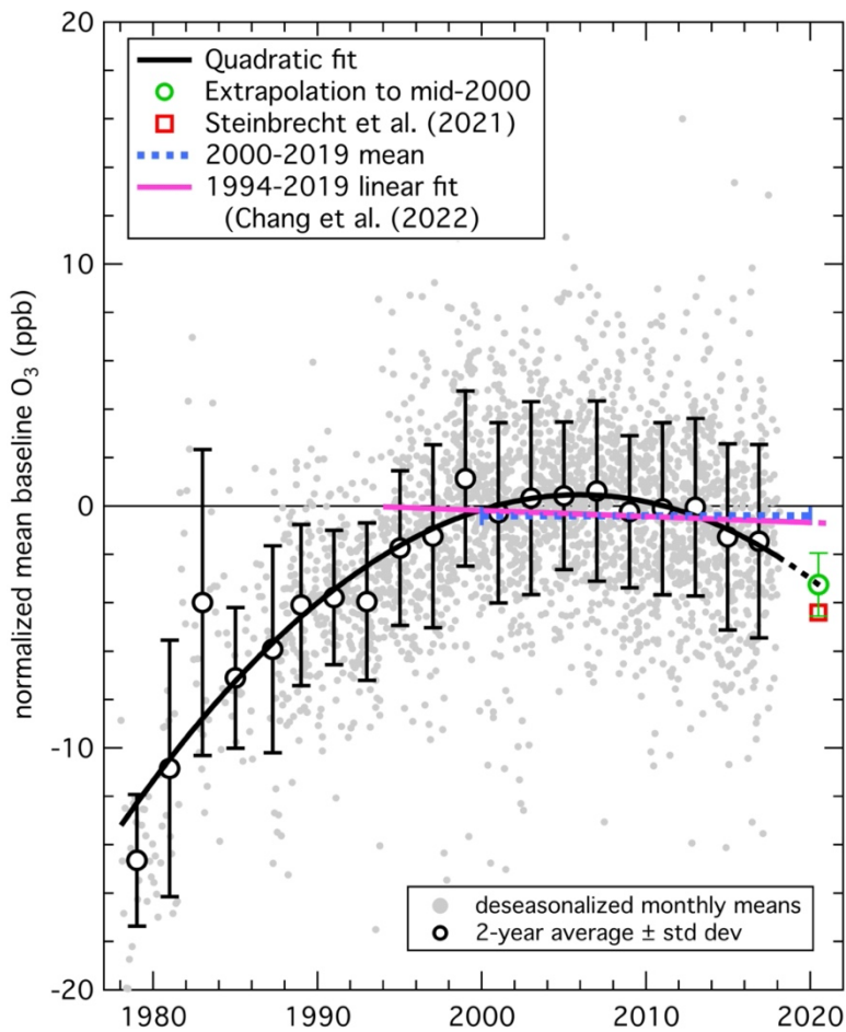
Figure 1: Baseline ozone concentrations at northern midlatitudes over four decades. Gray points are normalized, deseasonalized monthly mean northern midlatitude data; open circles with error bars are 2-year means with standard deviations of the gray points, and the black solid curve is a quadratic polynomial fit to the gray points (Parrish et al., 2020). The dashed black line extrapolates the quadratic fit to mid-2020. The red square and green circle indicate estimates of the year 2020 annual mean from Steinbrecht et al. (2021) and the extrapolation of the quadratic fit, respectively; the error bars on the green circle indicate the estimated 95% confidence limit of the extrapolation. The blue dotted bar indicates the 2000 to 2020 mean normalized baseline ozone derived from integration of the quadratic fit. The violet line segment has a slope equal to the weighted mean of the northern midlatitude linear trends for 1994-2019 given in Table 2 of Chang et al. (2022), normalized to the 1994-2018 2-year means.
