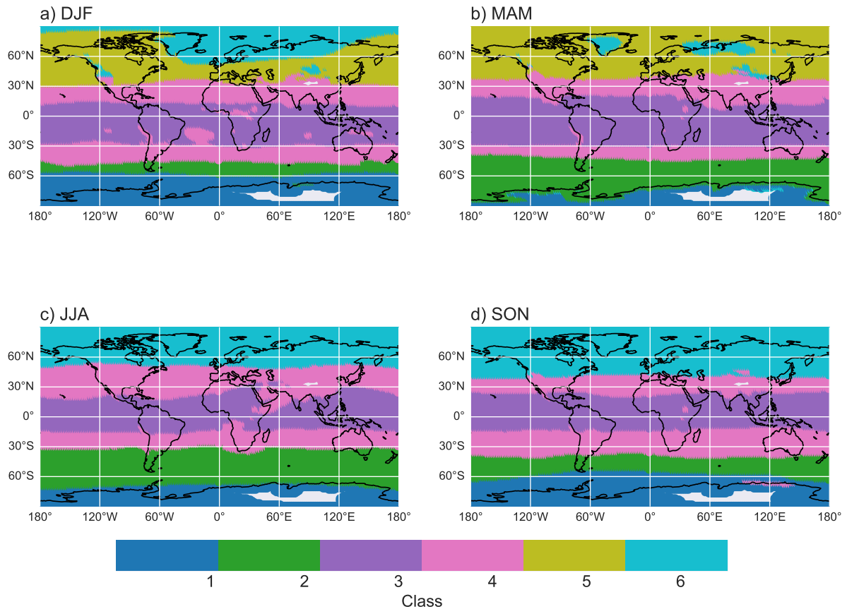
Figure 3. Map of profiles color-coded with the class they have been attributed to for model historical data (seasonal mean profiles covering 2009-2014 at each model grid cell) at 850 hPa.
