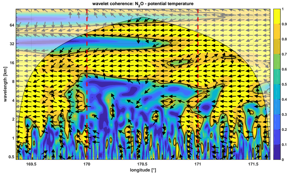
Figure 11. Wavelet coherence of N 2 O and potential temperature (wavelength = period · flight speed (216 m/s), see Eqn. 2). Arrows to the left indicate that N 2 O and potential temperature are shifted by 180°. In regions with a coherence lower than 0.5 the phase indication is removed. The shaded region marks the cone of influence, where edge effects affect the analysis. The solid lines shows the 95 % confidence level as given in paragraph 2.4. Yellow colors indicate a high coherence and blue colors indicate a low coherence. Vertical lines mark the upstream, above mountain, and downstream side.
