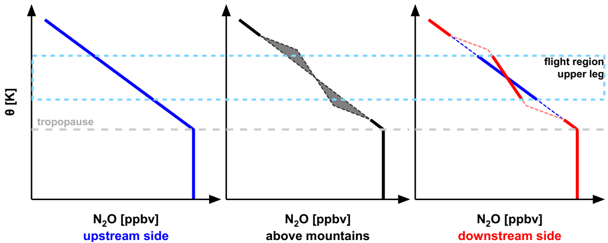
Figure 7. Schematic evolution of potential temperature \Theta versus N_2O in the presence of cross-isentropic mixing (indicated by the gray arrows) at the tropopause (e.g. by orographic wave-induced turbulence). The blue curve (left panel) shows the situation on the upstream side. The relation between N_2O and \Theta (blue) is modified by mixing (dotted black and gray shaded) over the mountains leading to a modified profile on the downstream side (red) compared to the original upstream relation (blue). The gray dashed line shows the tropopause and the light blue dash rectangle the flight region of the upper leg.
