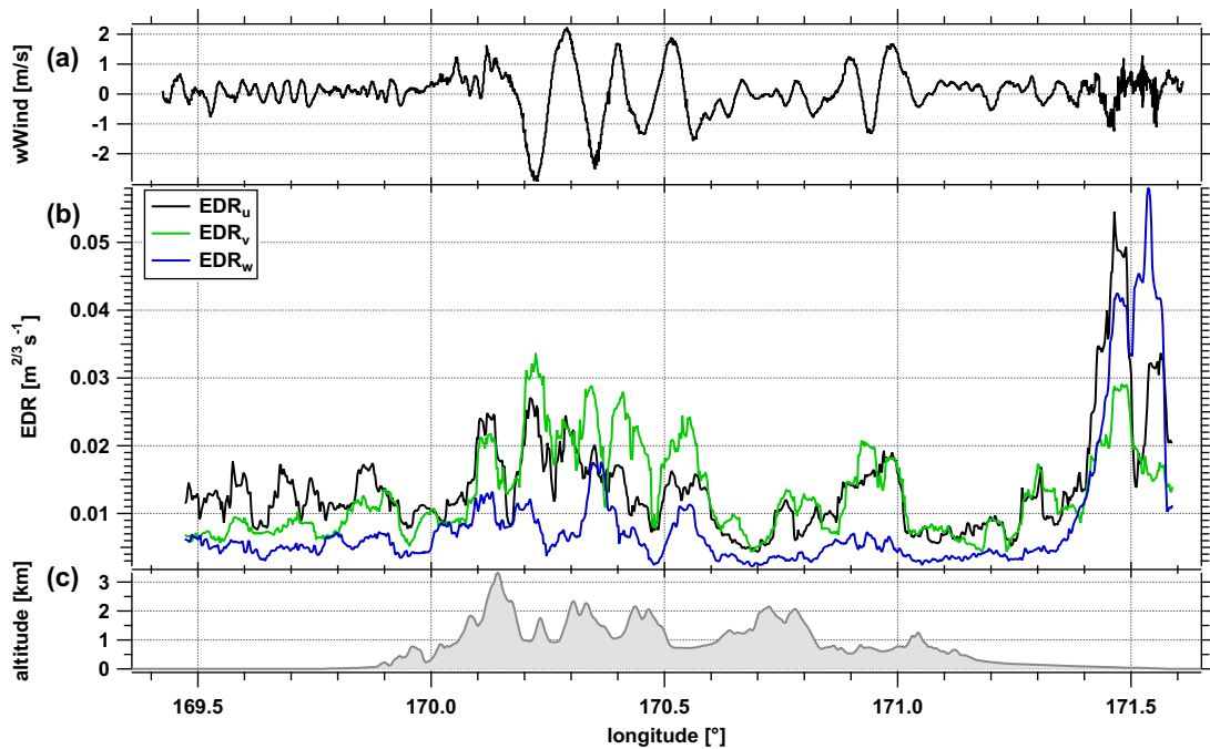
Figure 14. Timeseries Time series of (a) vertical wind, (b) EDR for the measured wind components for the upper flight leg indicating weak, but non-vanishing turbulence during the time of flight above the Southern Alps (orography shown in (c)).
