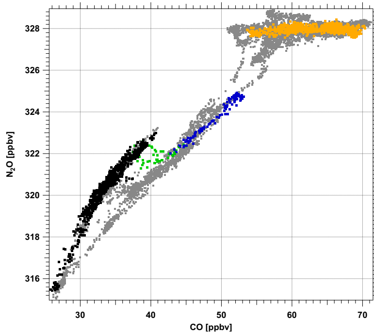
Figure 5. Scatterplot of N_2O versus CO for FF09 on 12 July 2014. The light gray points show the correlation of N_2O and CO for the whole flight. For the upper south-western flight leg from 18:48 UTC to 19:06 UTC in Figure 2 (also compare Fig. 6) the data points are black, blue and green. Black colors indicate potential temperatures \Theta > 328.1 K, blue for \Theta < 326.3 K. The region between these two levels is marked in green. The lower leg lies entirely in the troposphere as indicated by the orange data points of N_2O = 328 ppbv.
