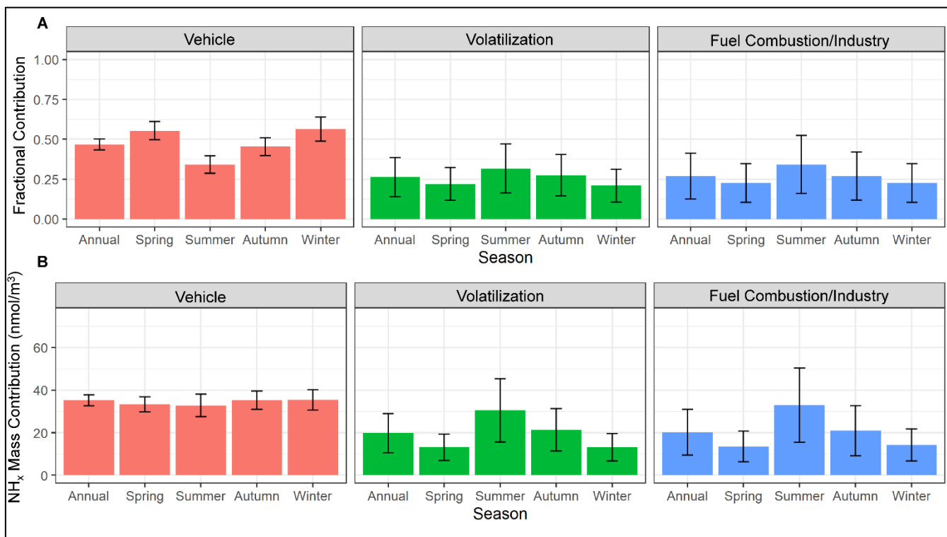
Figure 9. The calculated mean (A) fractional contribution and (B) mass weighted contributed of the major identified emission sources (Vehicle, Volatilization, Fuel Combustion/Industry) to NH x in Providence, RI, utilizing a stable isotope mixing model (SIMMR). The error bars represent the standard deviation of the model simulations.
