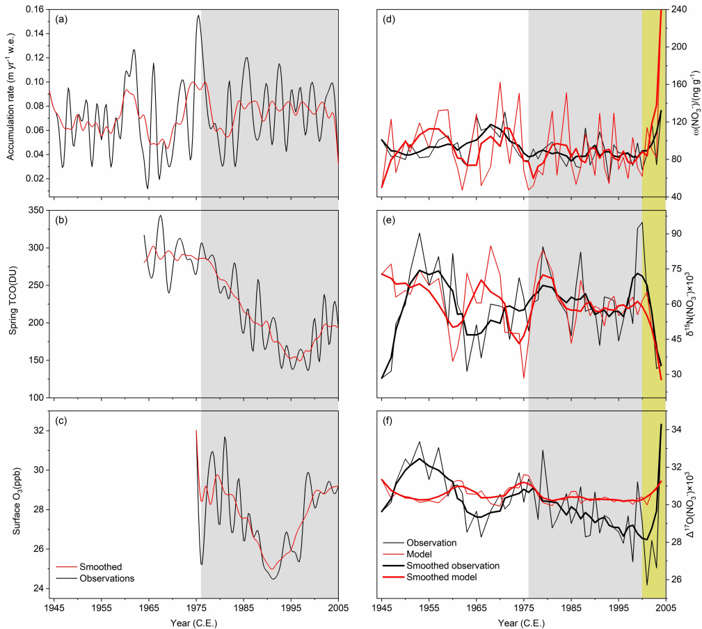
Figure 3. Left panels: time series of annual snow accumulation rate (a), spring (average from September 22 to October 13) TCO (total column ozone) (b), and summer half year surface O_3 concentrations (c) at the South Pole over the period of the ice core record. Red curves are the 5-year moving averages. Right panels: ice core nitrate concentration and isotopic compositions at the South Pole in 1944-2005 (black: observations; red: modeled). The thin lines represent the observed and modeled annual (d) \omega(NO_3^-) , (e) \delta^{15}N(NO_3^-) and (f) \Delta^{17}O(NO_3^-) from 1944-2005. The thick lines represent the 5-year moving averages. Yellow shaded area represents the period with changes in nitrate concentrations and isotopes from surface snow to below the photic zone. Grey shading area represents the ozone hole period.
