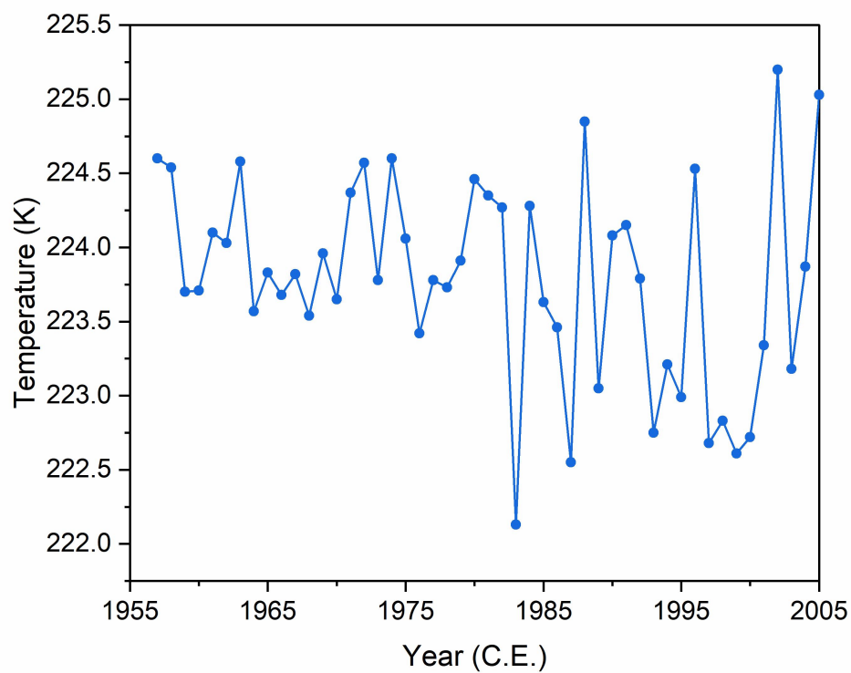
Figure S2 The annual mean atmospheric temperature from 1957 to 2005 at the South Pole (Surface station data of annual atmospheric temperature and wind speed in the South Pole ( https://ramadda.data.bas.ac.uk/repository/entry/show/?entryid=569d53fb-9b90-47a6-b3ca-26306e696706 )).
