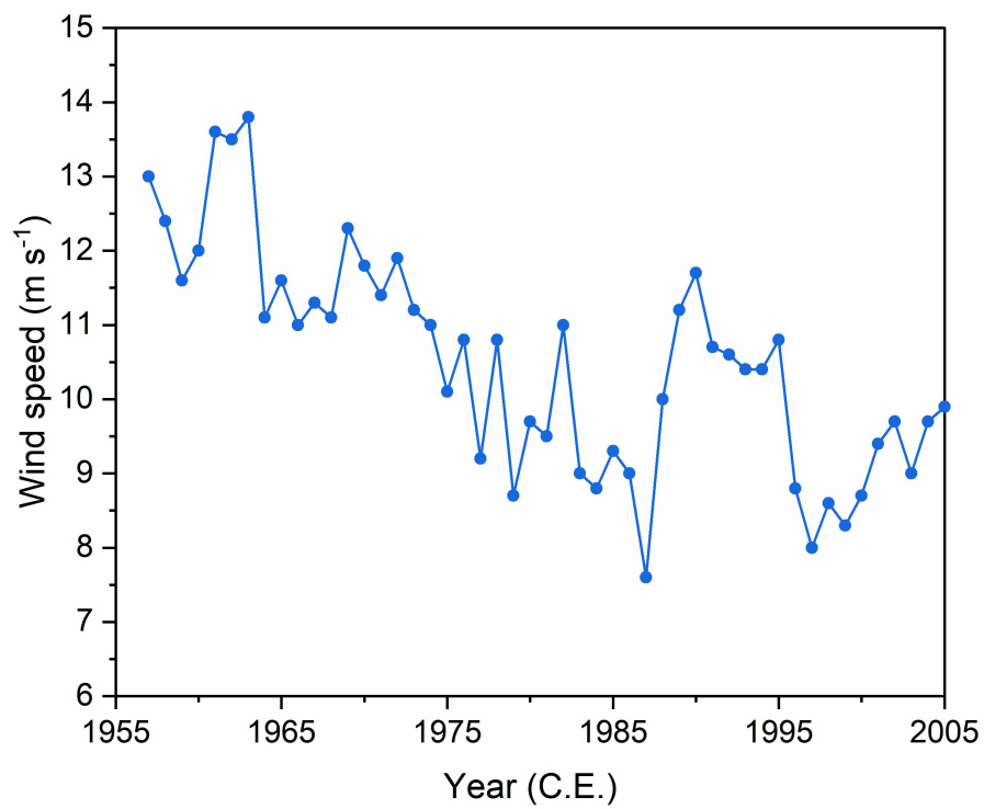
Figure S3 The annual mean wind speed from 1957 to 2005 at the South Pole
