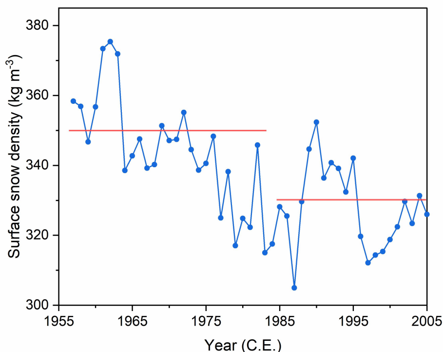
Figure S4 The calculated surface snow density from 1957 to 2005 at the South Pole
