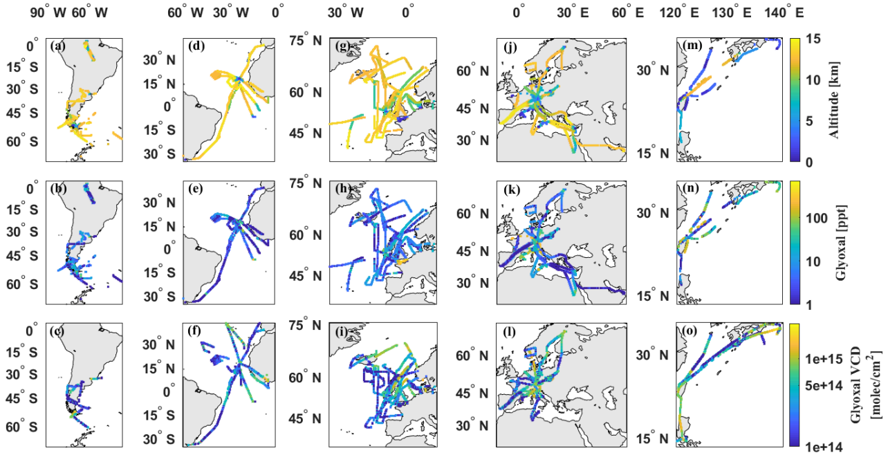
Figure 5. Flight trajectories, measured glyoxal mixing ratios, and VCDs are displayed in the top, middle and bottom rows, respectively, from-over South America (panels a, f, and ka-c), the Tropical Atlantic (panels b, g, and ld-f), the North Atlantic (panels e, h, and mg-i), Continental Europe (panels d, i, and nj-l), and South-East Asia (panels e, j, and om-o). Note the logarithmic colour scale in the two lower rows of the panels (f)–(o).
