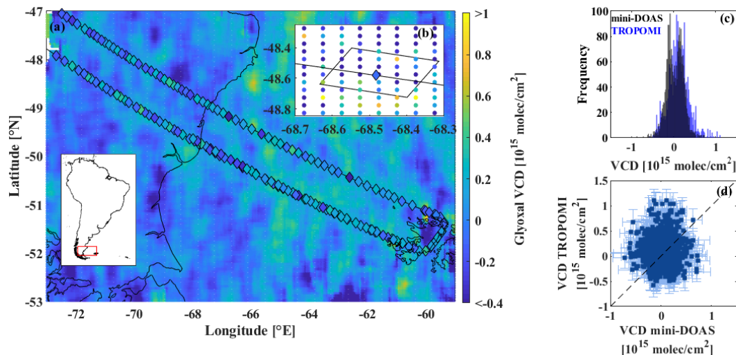
Figure 8. Glyoxal measurements in the pristine marine atmosphere over the South Atlantic between southern Patagonia (Argentina) and the Falkland Islands (UK) on 9 Nov. 2019. Panel (a): along-Along track mini-DOAS glyoxal measurements (diamonds with black contours) with the collocated same-day L3 TROPOMI observations at 0.25^\circ \times 0.25^\circ resolution. For better visibility, only every fifth mini-DOAS measurement is shown. Panel (b): spatial-Spatial gridding of 25 high-resolution TROPOMI measurements around an individual mini-DOAS observation. Panels (c) and (d): Frequency distribution and scatter plot of the inferred glyoxal VCDs from the mini-DOAS instrument versus TROPOMI L3 averaged on 0.25^\circ \times 0.25^\circ according to panel (b).
