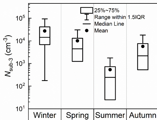
Figure 5. The seasonal variations of number concentrations of sub-3 nm aerosols ( N_{\text{sub-3}} ) on NPF days in urban Beijing. Data during 9:00 – 14:00 were shown in this figure. The vertical lines and circles in the box indicate the median and mean values, respectively. The top and bottom edges represent 75 th and 25 th percentiles, respectively. The IQR is the interquartile range.
