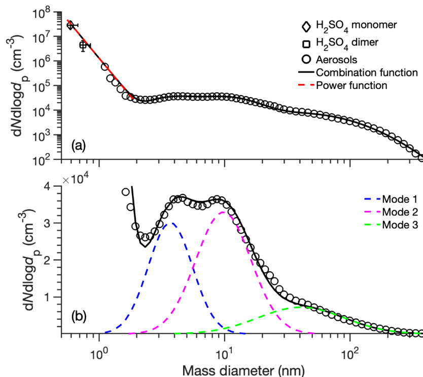
535 Figure 3. The median daytime NPF type number size distributions from H 2 SO 4 monomer to larger aerosols and the fitted size distributions shown in (a) logarithm scale and (b) linear scale of y axis. The x-axis error bars of H 2 SO 4 monomers and dimers indicate the variation range of estimated H 2 SO 4 monomers and dimers diameters by assuming the bulk density to be 1000~1800 kg m 3 . The y-axis error bars of H 2 SO 4 monomers and dimers indicate the 25 th ~75 th range of 540 concentrations. The black and red lines indicate the fitted size distribution in the whole size range and in sub-3 nm size range, respectively. The blue, magenta and green lines present the fitted mode 1, mode 2 and mode 3, respectively. The diamonds, squares, and circles represent the distribution function (dN/dlogd p ) of H 2 SO 4 monomers, dimers and aerosols, respectively.
