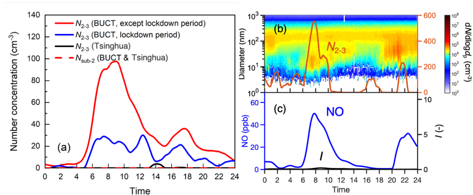
560 Figure 6. (a) Median diurnal variations of number concentrations of 2-3 nm aerosols ( N_{2-3} ) on non-NPF days at the BUCT site during COVID-19 lockdown period (Jan. 24, 2020 – Feb. 25, 2020) and other time period (except lockdown period), and at the Tsinghua site (Mar. 7, 2016 – Apr. 6, 2016). The median diurnal variations of number concentrations of sub-2 nm aerosols ( N_{sub-2} ) are near zero on non-NPF days at both BUCT and Tsinghua sites. The temporal pattern of (b) aerosol size distributions, N_{2-3} , (c) NO concentration and the indicator I on a non-NPF day (Mar. 13, 2018).
