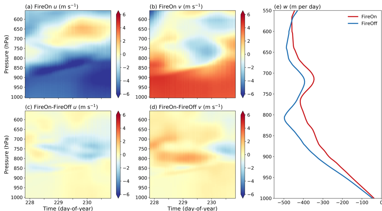
560 Figure 6. Lagrangian curtains of horizontal winds and averaged profiles of subsidence. Zonal and meridional winds are shown for (a-b) FireOn and (c-d) the FireOn-FireOff difference, respectively. The (e) subsidence profiles are averaged over all times.
