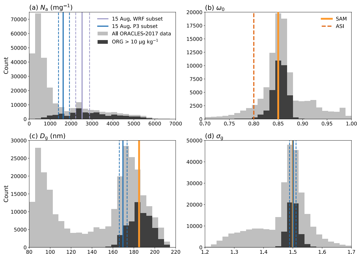
Figure 4. ORACLES-2017 flight statistics and assumed aerosol size distribution and optical properties for SAM. All flight data is represented as light grey histograms and data with organic aerosol concentrations (ORG) greater than 10 \mu\text{g kg}^{-1} as dark grey histograms for (a) aerosol number concentration, (b) dry single-scatter albedo at 550 nm, and the (c) geometric mean diameter and (d) geometric standard deviation of the aerosol size distribution. Blue solid and dashed lines denote mean and interquartile values, respectively, for the 15 August 2017 flight between 1100 and 1300 UTC for \text{ORG} > 10 \mu\text{g kg}^{-1} . The purple solid and dashed lines in (a) denote the mean and interquartile values, respectively, of WRF-CAM5 FireOn aerosol number concentration subset along the P3 flight track from 1100 to 1300 UTC on 15 August 2017 for \text{ORG} > 10 \mu\text{g kg}^{-1} . Values selected for use in the standard SAM aerosol representation are shown as gold lines. The dashed orange line in (b) represents the average single-scatter albedo value observed during the LASIC campaign (ASI) for August 2017.
