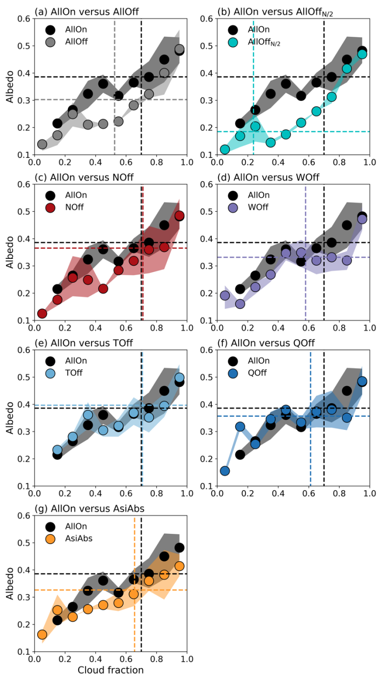
870 Figure 17. Scene albedo-cloud fraction summary plots for each simulation. Binned AllOn values are compared with (a) AllOff, (b) AllOff N/2 , (c) NOff, (d) WOff, (e) TOff, (f) QOff, and (g) AsiAbs. Dashed lines correspond to mean daytime values over the course of the simulation and markers and shading correspond to the mean and interquartile range of scene albedo for each cloud fraction bin, respectively.
