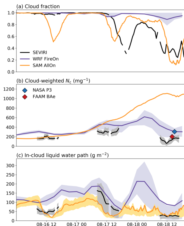
965 Figure 21. Comparison of SEVIRI retrievals and model output over the course of the Lagrangian trajectory. Lines represent mean values and shading interquartile ranges for (a) cloud fraction, (b) cloud droplet number concentration, and (c) in-cloud liquid water path. The markers in (b) represent the average N_c weighted by cloud water content for the ORACLES (blue) and CLARIFY (red) flights.
