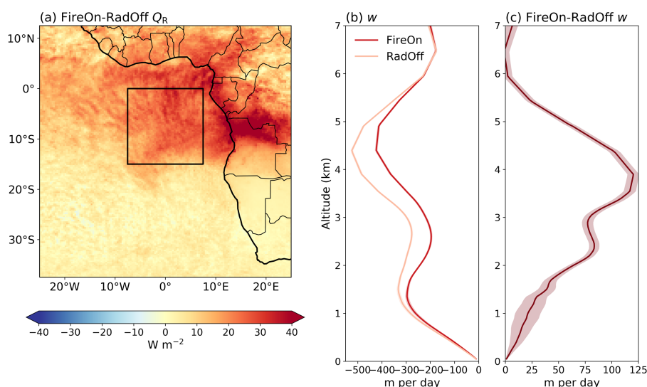
Figure 10. Atmospheric column radiative heating and vertical profile of subsidence differences between FireOn and RadOff. Subsidence values averaged over the region from 0° to 15° S, 7.5° W to 7.5° E and over the full 14-20 August 2017 period, demarcated in black in (a), are shown separately for FireOn and RadOff in (b) and as the FireOn-RadOff difference in (c). Shading in (b-c) represents two standard errors of the mean.
