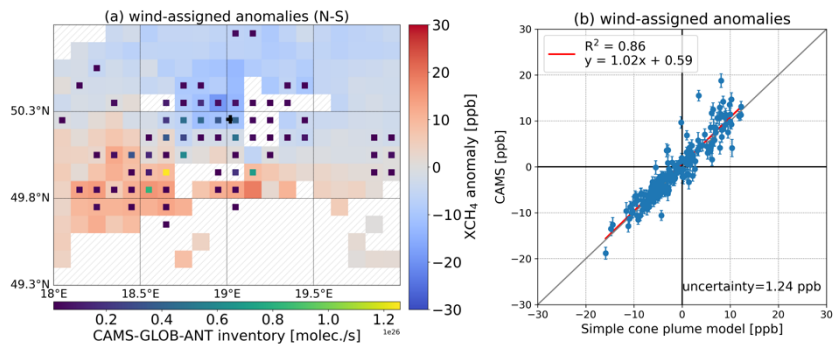
Figure 10: Similar figures to Figure 5b-c. Results are derived from CAMS XCH 4 , CAMS emission inventory and ERA5 wind at 330 m but using a new wind category (N and S).
