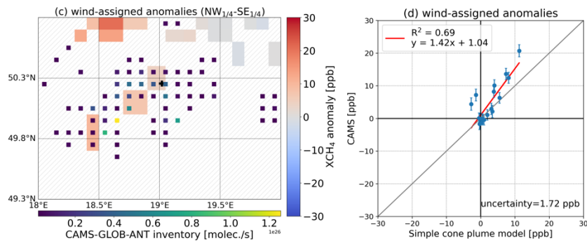
360 Figure 9: Similar figures to Figure 5b-c. Results are derived from CAMS XCH 4 , CAMS emission inventory and ERA5 wind at 330 m for (a)-(b) narrow wind coverage (NE 1/4 and SW 1/4 ), and (c)-(d) narrow wind coverage (NW 1/4 and SE 1/4 ).
