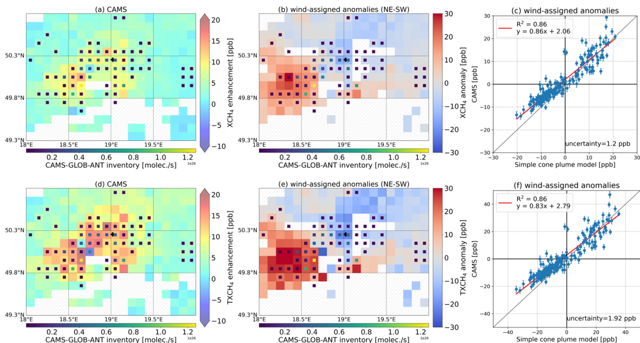
Figure A- 4: Similar to Figure 5 but using ERA5 wind at 10 m.
