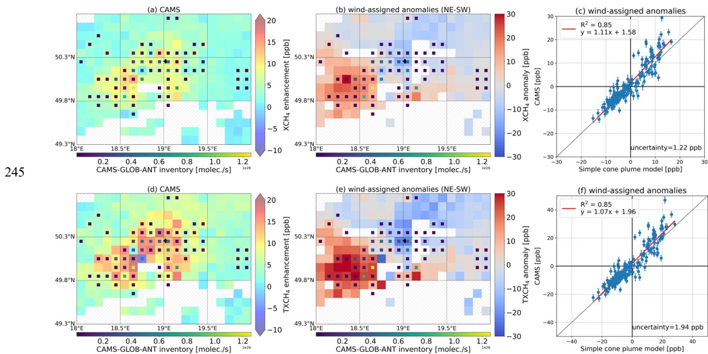
Figure 5: (a)-(c): CAMS XCH 4 enhancement (XCH 4 -background), the wind-assigned anomalies (NE-SW), and correlation plot of the wind-assigned anomalies between CAMS and the simple cone plume model with using the CAMS-GLOB-ANT inventory ( 9.7E26 molec./s in total) and ERA5 wind at 330 m during November 2017-December 2020 over the USCB region. (d)-(f): the same as for the upper panel but for CAMS TXCH 4 . The square symbols represent the locations of the CAMS-GLOB-ANT ( >1E24 molec./s) inventory and different colors denote the amount of emission rates. The hatched areas in (a)-(b) and (d)-(e) represent no data in these grids. The uncertainties in (c) and (f) represent the mean error bars, i.e., error propagation of the background uncertainty and the CAMS standard deviation.
