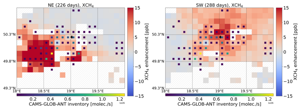
480 Figure A- 3: The enhancements for wind coming from NE and SW.
