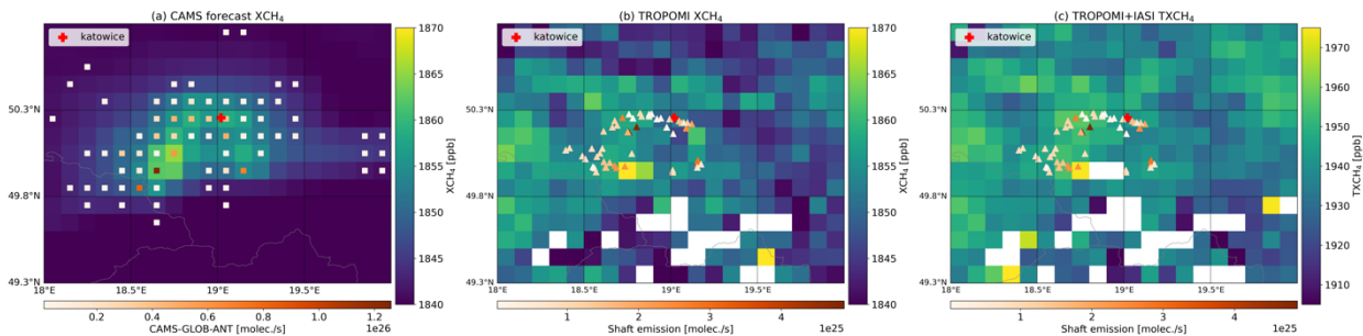
230 Figure 4: Averaged (a) CAMS forecast XCH 4 , (b) TROPOMI XCH 4 , and (c) TROPOMI+IASI TXCH 4 in the USCB region on a 0.1° × 0.1° latitude/longitude grid during November 2017-December 2020. The square and triangle symbols represent the locations of CAMS-GLOB-ANT sources (for better viewing, only the emission strengths larger than 1E24 molec./s are shown here) and the active coal mine shafts from the CoMet inventory (Galkowski et al., 2021), respectively. Different colors denote the amount of emission rates. The white grids represent no data from TROPOMI or the number of the points in the grid less than 5. A zoom version of panel (b) is shown in the appendix (Figure A- 2). Note, a different colorbar has been used in panel (c).
