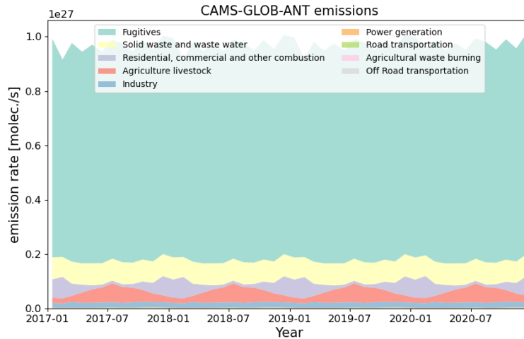
140 Figure 1: Stacked area plot for different sectors of the monthly averaged CAMS global anthropogenic emissions ( >1E20 molec./s) in the USCB region for 2017-2020 ( https://permalink.aeris-data.fr/CAMS-GLOB-ANT , last access: 22 December 2021. Granier et al., 2019).
