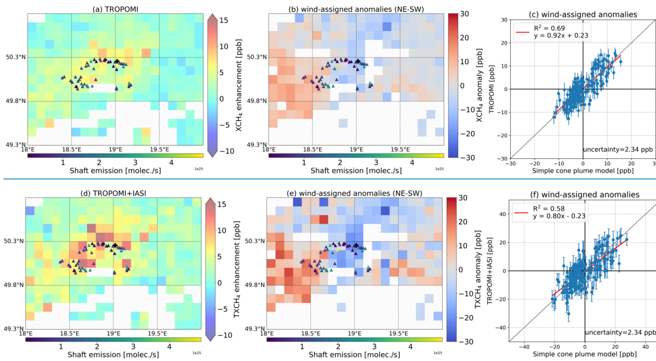
330 Figure 7: Similar to Figure 5, but for (a-c) TROPOMI XCH 4 and (d-f) TROPOMI+IASI TXCH 4 . The a priori knowledge of sources are based on the CoMet inventory (6.6E26 molec./s in total, Galkowski et al., 2021). The triangle symbols represent the locations of the active coal mine shafts and different colors denote the amount of emission rates.
