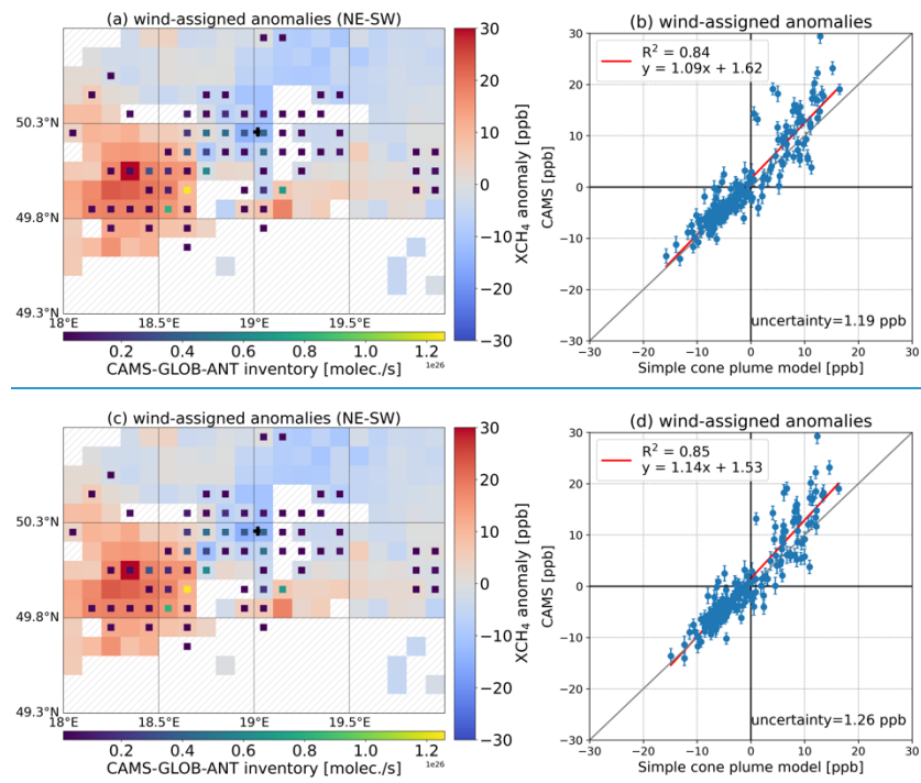
Figure 11: Similar figures to Figure 5b-c. Results are derived from CAMS XCH 4 , CAMS emission inventory and ERA5 wind at 330 m for (a)-(b) \alpha = 50^\circ , and (c)-(d) \alpha = 70^\circ .
