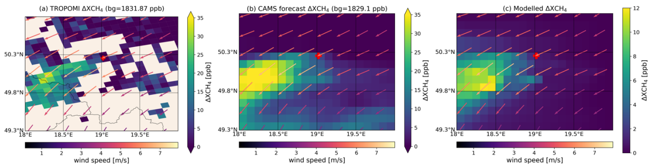
Figure 6: \Delta XCH_4 together with the ERA5 wind at 12:00 UTC from (a): TROPOMI observations at 11:34 UTC, (b): CAMS forecast at 12:00 UTC, and (c): from the simple cone plume model (averaged over the daytime) based on the CAMS-GLOB-ANT inventory
