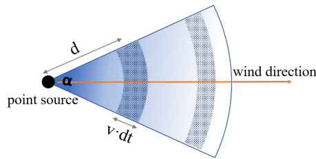
Figure A- 1: Sketch of the simple cone plume model used to explain the CH 4 emission estimation method. The methane at the point source is distributed along the wind direction (wind speed: v ) in the cone-shaped area with an opening angle of \alpha . The point source emits the methane at an emission rate of \epsilon . We assumed the methane molecules are evenly distributed in the dotted area A, and the distance from area A to the point source is d . Therefore, the emitted methane in dt time period equals to the amount of methane in the area A. It yields the equation \epsilon \times dt \approx \Delta column \times \frac{\alpha}{\pi} \times \pi \times d \times v \times dt . This figure is adopted from Tu et al. (2022).
