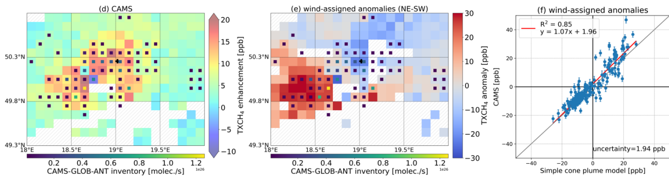
Figure 5: (a)-(c): CAMS XCH 4 enhancement (XCH 4 -background), the wind-assigned anomalies (NE-SW), and correlation plot of the wind-assigned anomalies between CAMS and the simple cone plume model with using the CAMS-GLOB-ANT inventory (9.7E26 molec./s in total) and ERA5 wind at 330 m during November 2017-December 2020 over the USCB region. (d)-(f): the same as for the upper panel but for CAMS TXCH 4 (colorbars in (d) and (e) are different from that for XCH 4 ). The square symbols represent the locations of the CAMS-GLOB-ANT (>1E24 molec./s) inventory and different colors denote the amount of emission rates. The hatched areas in (a)-(b) and (d)-(e) represent no data in these grids. The uncertainties in (c) and (f) represent the mean error bars, i.e., error propagation of the background uncertainty and the CAMS standard deviation.
