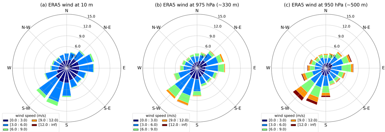
Figure 3: Windrose plots for daytime (08:00 UTC – 18:00 UTC) from November 2017 to December 2020 for the ERA5 model wind at different vertical levels (10 m, ~330 m and ~500 m). The days for the three-year average coincide with the TROPOMI overpass days.
