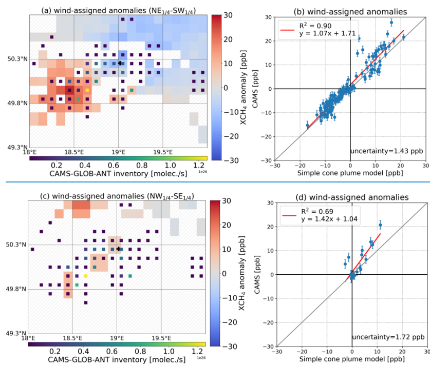
Figure 9: Similar figures to Figure 5b-c. Results are derived from CAMS XCH 4 , CAMS emission inventory and ERA5 wind at 330 m for (a)-(b) narrow wind coverage ( NE_{1/4} and SW_{1/4} ), and (c)-(d) narrow wind coverage ( NW_{1/4} and SE_{1/4} ).
