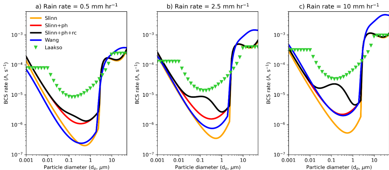
Figure 3. BCS rate ( \Lambda , Eq. 2) as a function of aerosol diameter for 5 BCS models (Section 2), and for rain rates representing (a) drizzle, (b) moderate rain, and (c) heavy rain
