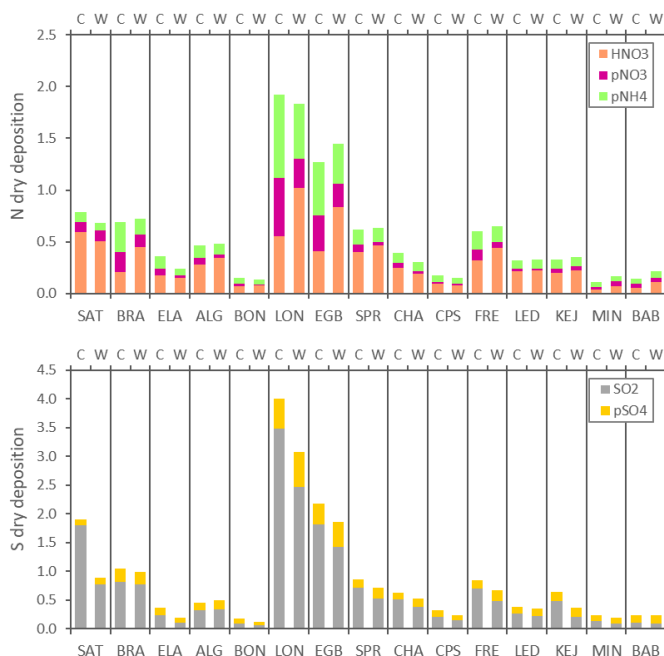
410 Figure 3: Mean dry deposition fluxes of N and S species ( \text{kg N or S ha}^{-1} \text{ yr}^{-1} ) during the cold (Nov-Apr) and warm (May-Oct) seasons during 2000-2018 at CAPMoN sites. C: cold season; W: warm season. Gaseous species: \text{HNO}_3 and \text{SO}_2 ; particulate (p) species: \text{pNO}_3 , \text{pNH}_4 and \text{pSO}_4 . Sites are listed in order longitudinally from west (left) to east (right).
