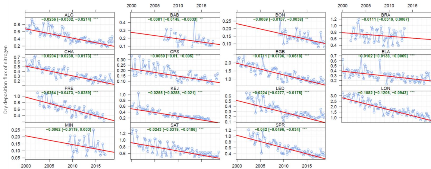
Figure 4: Annual trends in dry deposition fluxes of nitrogen at CAPMoN sites ( \text{kg N ha}^{-1} \text{yr}^{-1} ). Theil-Sen slope and 95% confidence interval (green text); trendline de-seasonalized using LOESS (red line); observed seasonal mean dry deposition fluxes (blue time-series). Note: excludes \text{NH}_3 and other \text{NO}_y dry deposition. Statistically significant trends shown with *** ( p < 0.001 ) or ** ( p < 0.01 ).
