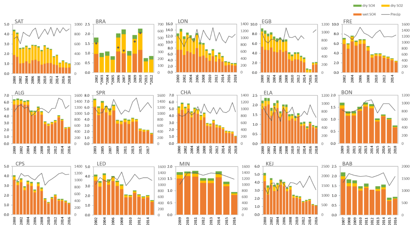
665 Figure 10: Long-term annual trends in total (dry+wet) deposition of sulfur at CAPMoN sites, 2000-2018. Total deposition (kg S ha -1 yr -1 , primary y-axis); precipitation (mm yr -1 , secondary y-axis); * indicates dry or wet deposition data were not available because data completeness criteria were not met.
