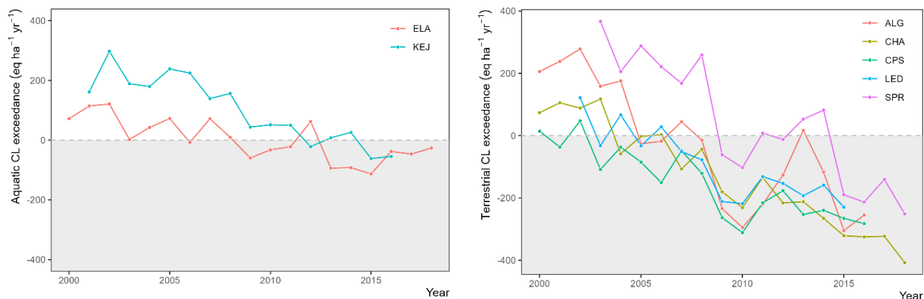
Figure 11: Critical load (CL) exceedances from total sulfur and nitrogen deposition near selected CAPMoN stations at Algoma (ALG), Chalk River (CHA), Chapais (CPS), Experimental Lakes Area (ELA), Lac Edouard (LED), Kejimikujik National Park (KEJ), and Sprucedale (SPR) for lakes (left) and soils (right). Stations with deposition fluxes below CL in every year from 2000-2018 are not shown. The grey area represents non-exceedance.
