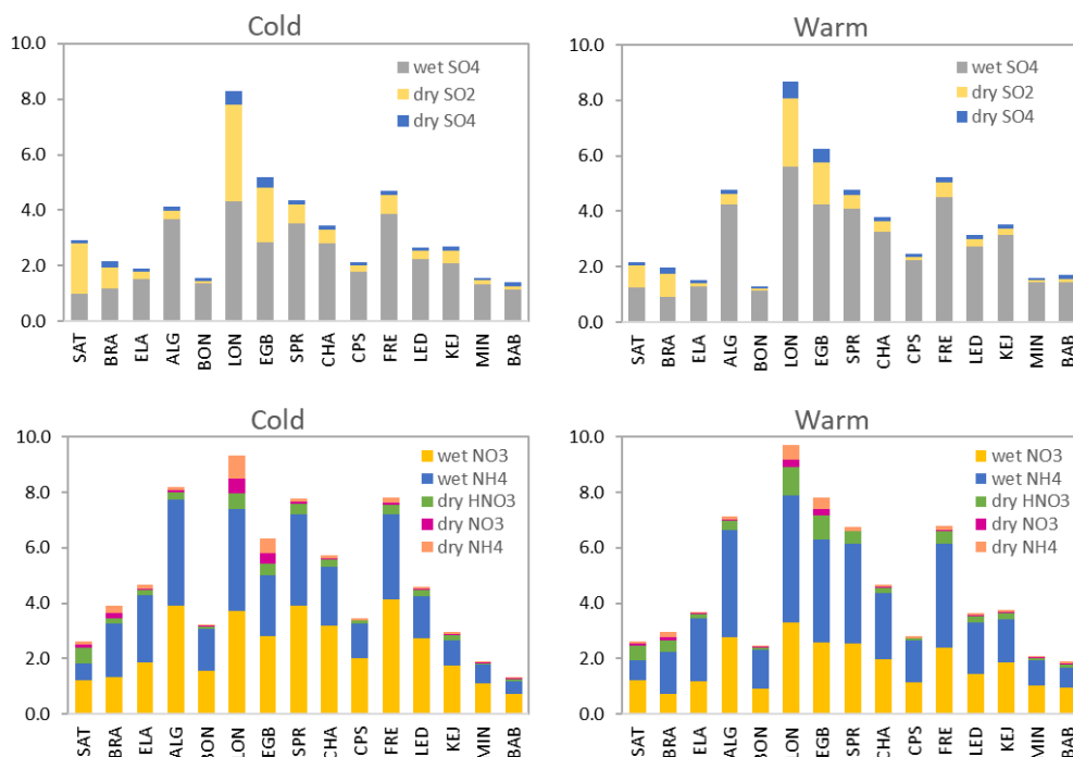
580 Figure 8: Mean total (dry+wet) deposition fluxes of N and S species in kg N or S ha -1 yr -1 during the cold (Nov-Apr) and warm (May-Oct) seasons at CAPMoN sites during 2000-2018. Sites are listed in order longitudinally from west (left) to east (right).
