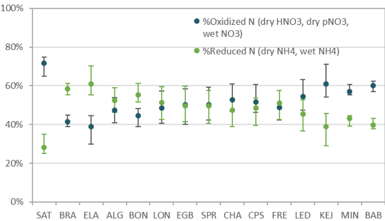
500 Figure 6: Percentage of oxidized and reduced N species in annual total deposition of N at CAPMoN sites during 2000-2018. Mean (circle); range or annual variability (error bars). Sites are listed in order longitudinally from west (left) to east (right).
