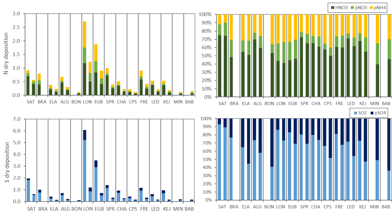
Figure 2: Dry N and S deposition fluxes ( \text{kg N or S ha}^{-1} \text{ yr}^{-1} ) and the percentage of N or S species in dry deposition for the 5-year period in 2000-2004 and in 2014-2018 at CAPMoN sites. For each site, the first bar represents the 2000-2004 values and the second bar represents the 2014-2018 values. Gaseous species: \text{HNO}_3 and \text{SO}_2 ; particulate (p) species: \text{pNO}_3^- , \text{pNH}_4^+ and \text{pSO}_4 . Sites are listed in order longitudinally from west (left) to east (right).
