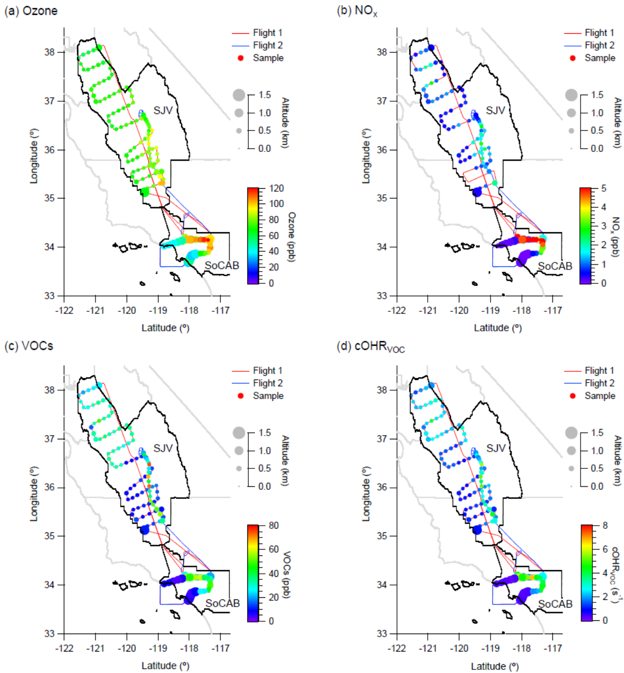
85 Figure 1: Spatial distribution of (a) O 3 , (b) NO x , (c) VOCs, and (d) cOHR voc . The flight tracks and sample locations are represented by colored lines and points, respectively. The points are sized by flight altitude and colored by the mixing ratios of O 3 , NO x , VOCs, and cOHR voc values in (a), (b), (c), and (d), respectively, with the scales shown in the legend. The background map (grey) shows the boundaries of the California air basins, with black indicating the SoCAB and SJV.
