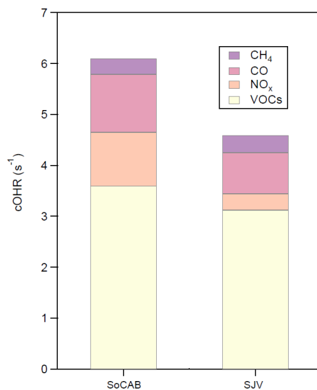
Figure 3: The total measured \Theta_{HRcOHR} for the SoCAB and SJV.
