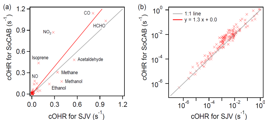
Figure 45: Scatter plot of \Theta_{HRcOHR}_{SoCAB} versus \Theta_{HRcOHR}_{SJV} for the individual species in (a) linear scale and (b) logarithmic scale. The red line represents linear regression using the orthogonal distance regression method.
