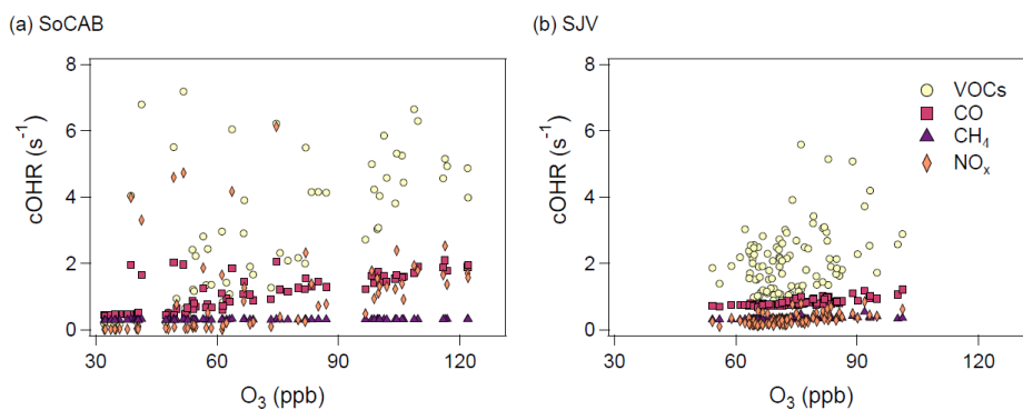
Figure 4: Scatter plot of \text{OHR}_{\text{VOC}} , \text{OHR}_{\text{CO}} , \text{OHR}_{\text{CH}_4} , and \text{OHR}_{\text{NO}_x} versus \text{O}_3 for the (a) SoCAB and (b) SJV.
