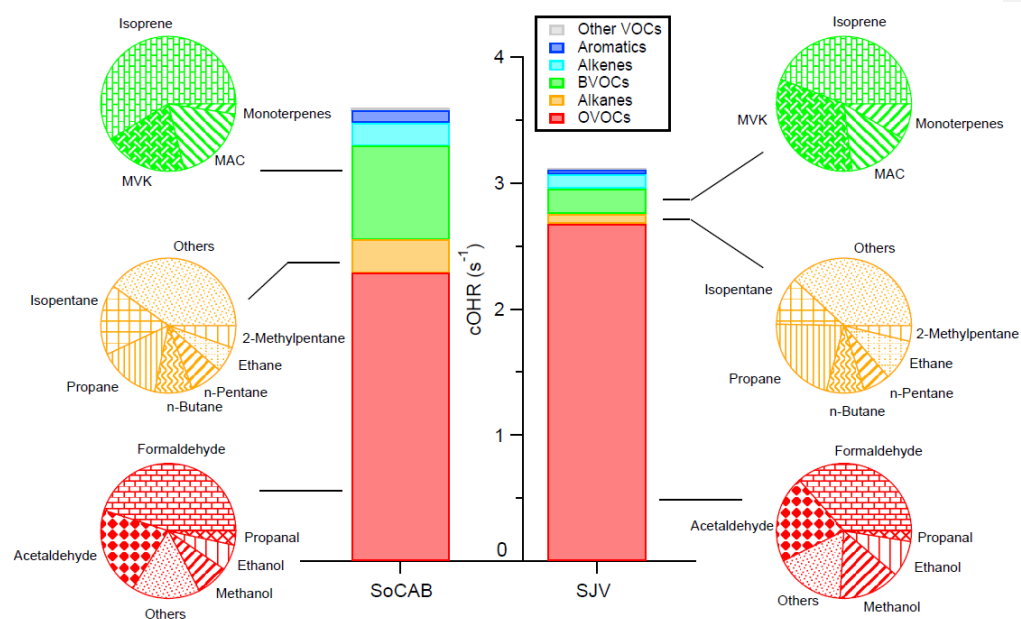
335 Figure 56: The measured \Theta_{HR}cOHR of VOCs in the SoCAB and SJV.
