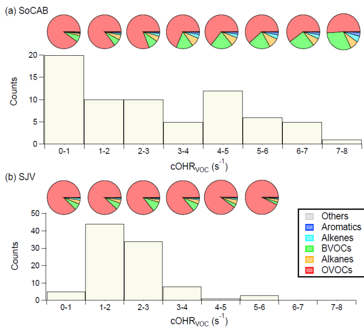
Figure 67: Frequency distribution of \overline{OHr_cOHR}_{VOC} in the (a) SoCAB and (b) SJV. Also shown above each 1-s^{-1} binned \overline{OHr_cOHR}_{VOC} range is a pie chart presenting the average contribution to the \overline{OHr_cOHR}_{VOC} by VOC categories (shown in the legend).
