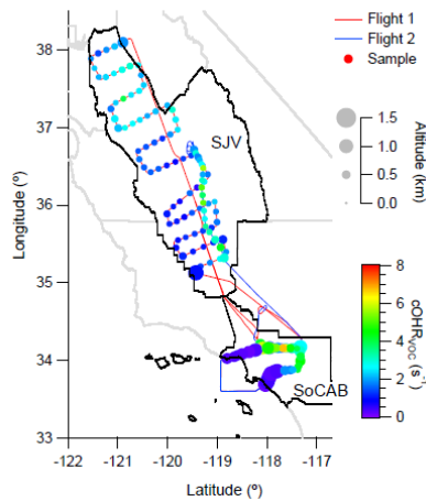
Figure 1: Spatial distribution of (a) O 3 , (b) NO x , (c) VOCs, and (d) \text{cOHR}_{\text{VOC}} . The flight tracks and sample locations are represented by colored lines and points, respectively. The points are sized by flight altitude and colored by the mixing ratios of O 3 , NO x , VOCs, and \text{cOHR}_{\text{VOC}} values in (a), (b), (c), and (d), respectively, with the scales shown in the legend. The background map (grey) shows the boundaries of the California air basins, with black indicating the SoCAB and SJV.
