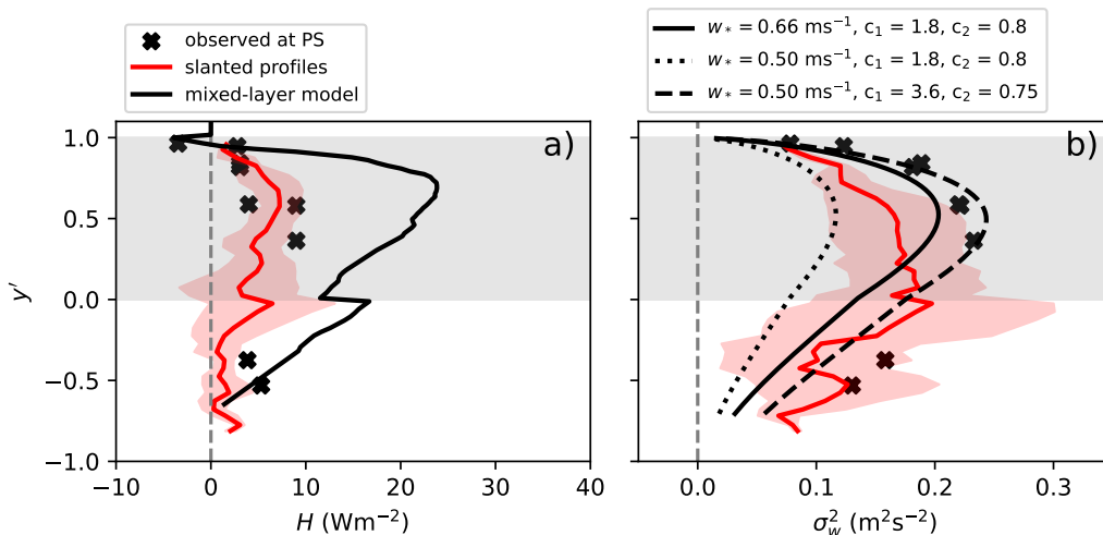
Figure 14. Observed and diagnosed turbulent heat flux profiles for 5 June (a) and vertical velocity variance (b) obtained using the Lenschow et al. (1980) parameterization (Equation C17) with w_* = 0.5 \text{ m s}^{-1} and w_* = 0.66 \text{ m s}^{-1} and with modified constants c_1 and c_2 .
