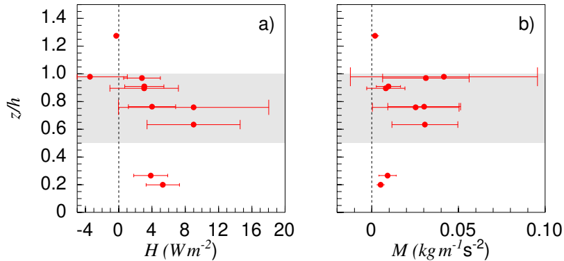
Figure A2. Left panel: Fluxes of sensible heat and of absolute values of momentum as measured on 5 June 2017. Whiskers in both panels show the sampling error \epsilon determined following Friehe et al. (1991)
