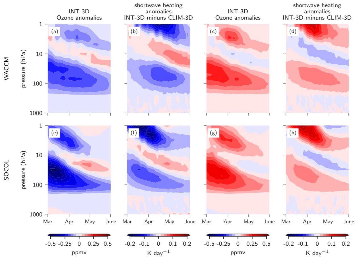
Figure A6. Ozone and shortwave heating anomalies in high and low ozone springs. Ozone anomalies in experiments with interactive ozone chemistry in low (a, e) and high (c, g) ozone springs as well as differences in shortwave heating anomalies between INT-3D and CLIM-3D in low (b, f) and high (d, h) ozone springs in WACCM (upper panel) and Socol-MPIOM (lower panel).
