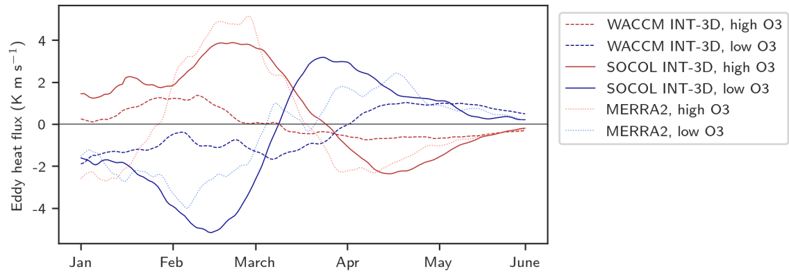
Figure A5. Heatflux at 100 hPa in high and low ozone springs. Eddy heat flux anomalies ( \text{K m s}^{-1} , 30 day running mean) averaged over 45\text{-}75^\circ\text{N} at 100 hPa for high and low ozone springs for WACCM and SOCOL-MPIOM INT-3D simulations, as well as for MERRA2.
