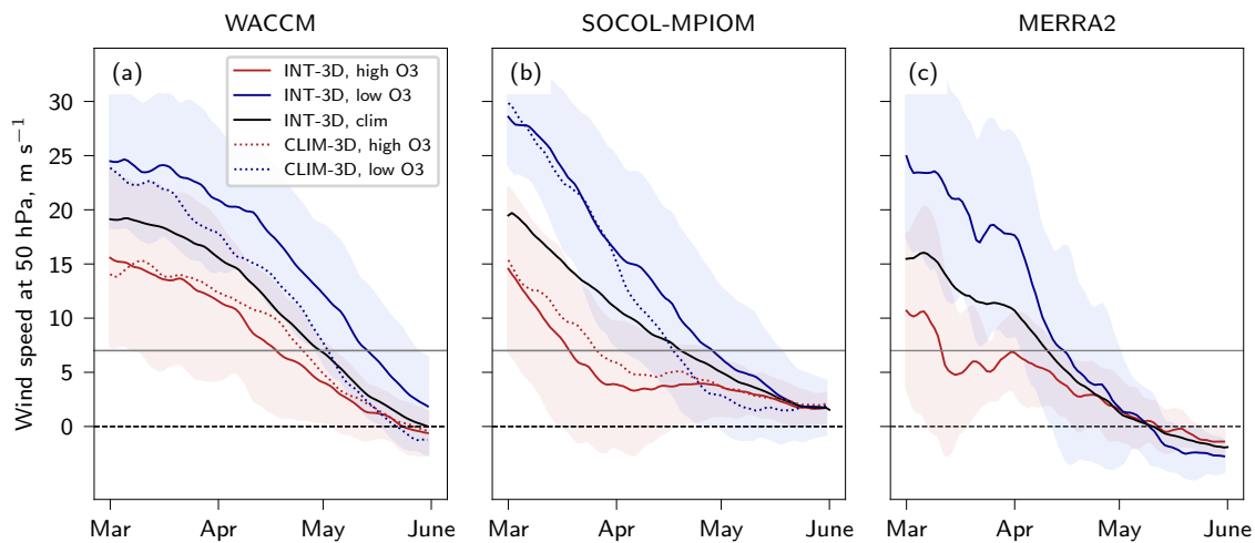
Figure A1. Zonal wind evolution in high and low ozone springs. Zonal mean zonal wind at 50 hPa averaged between 55 and 75°N in high (red) and low (blue) ozone springs in INT-3D (solid line) and CLIM-3D (stippled line) as well as the wind climatology (black) in (a) WACCM and (b) SOCOL-MPIOM. The grey line indicates the wind threshold of 7 \text{ m s}^{-1} used to define the FSW date at 50 hPa. Shaded areas show the standard deviation in high and low ozone springs in INT-3D simulations.
