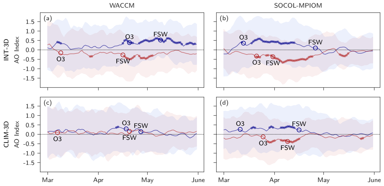
Figure A4. AO evolution in high and low ozone springs. Evolution of the Arctic Oscillation in the 25% of springs with the lowest (blue) and highest (red) ozone concentrations in WACCM (first column) and SOCOL-MPIOM (second column) in INT-3D (a, b) and CLIM-3D (c,d). Dots mark days where the AO is significantly different from zero on a 5% level based on a Student t-test. Shaded areas show the standard deviation across ozone high/low years. Circles mark mean ozone maximum/minimum dates and mean FSW dates in high/low ozone springs.
