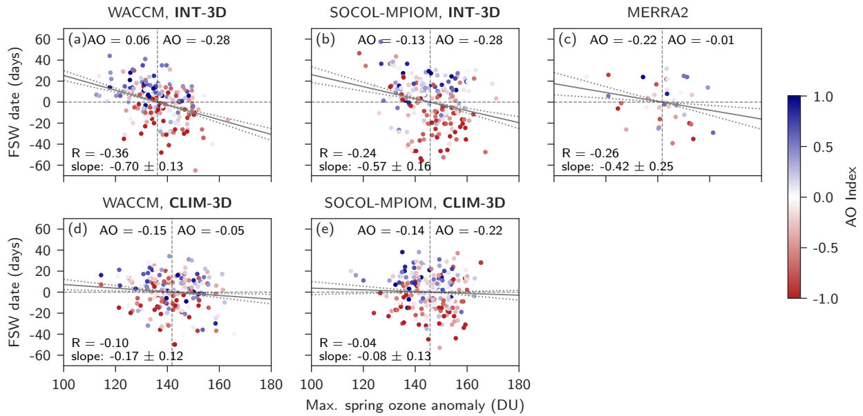
Figure 3. Correlation of the FSW date and preceding spring ozone. Linear regression of the maximum 5-day running mean partial ozone column between February 20th and the FSW in the respective year in WACCM INT-3D (a), SOCOL-MPIOM INT-3D (b) and MERRA2, as well as in WACCM CLIM-3D (d) and SOCOL-MPIOM CLIM-3D (e). Colors represent the AO Index in the month after the FW date, grey solid lines the linear regression lines. "R" denotes the Pearson correlation coefficient. Vertical grey stippled lines mark the mean ozone value over all years. Mean AO Indices are given for years with especially high (left) or low (right) ozone.
