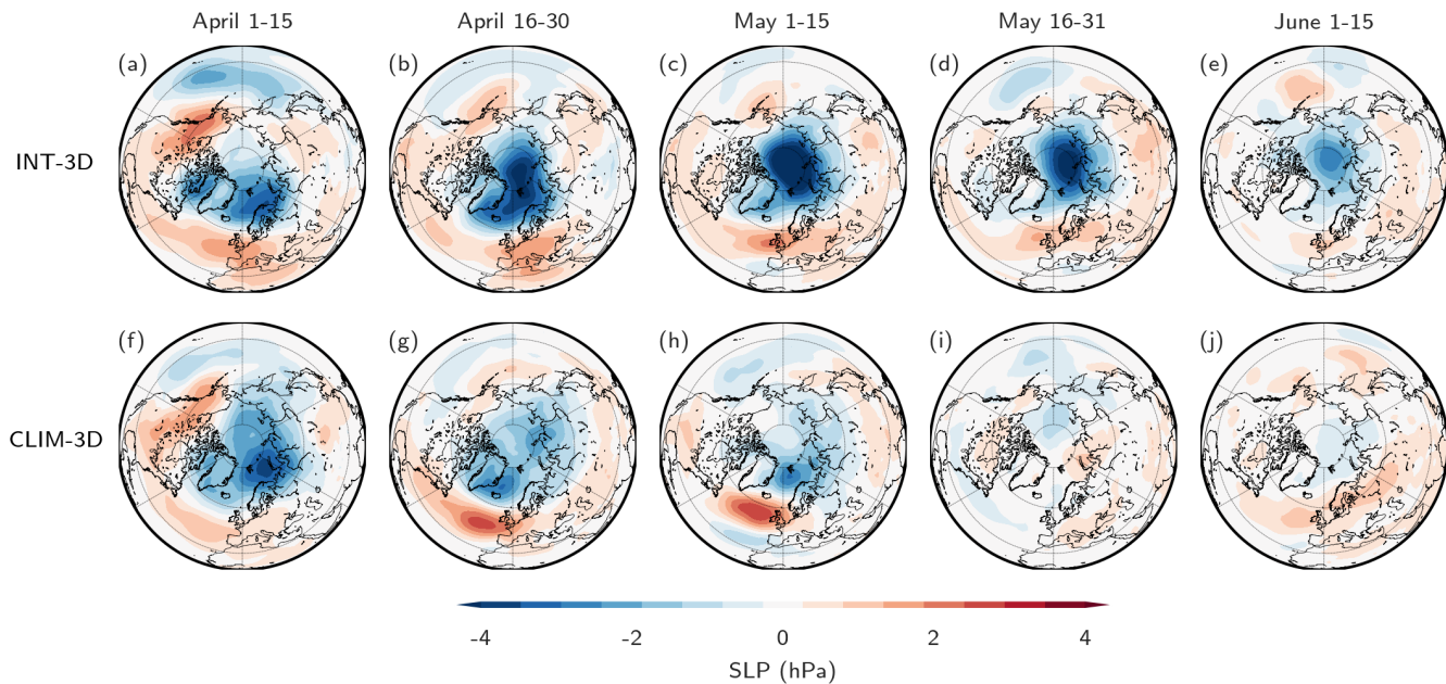
Figure 6. Seasonal evolution of SLP anomalies in low ozone years in WACCM. Evolution of SLP anomalies from April to June in low ozone springs in WACCM simulations with interactive ozone chemistry (a-e) and climatological ozone (f-j). The mean ozone minimum date in INT-3D simulations is April 20, the mean FSW date is May 10.
