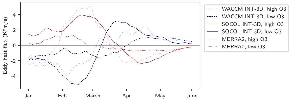
Figure A5. Heatflux at 100 hPa in high and low ozone years. Eddy heat flux anomalies (K*m/s, 30 day running mean) averaged over 45-75°N at 100hPa for high and low ozone years for WACCM and SOCOL-MPIOM INT-3D simulations, as well as for reanalysis.
