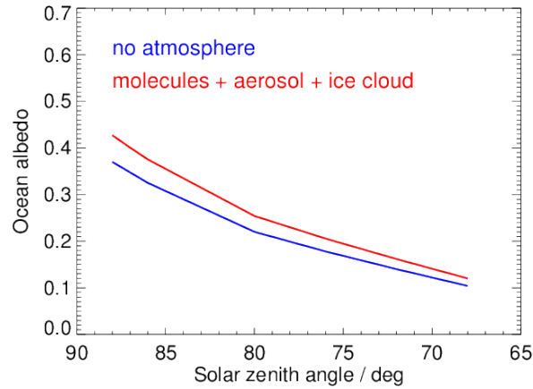
Figure 7. Broadband albedo at the ocean surface as a function of solar zenith angle after Payne (1972) for an atmospheric transmission transmission of 1.0 (blue curve) and for the atmosphere on 25 January 2016 containing molecules, aerosol particles, and an ice cloud (red curve).
