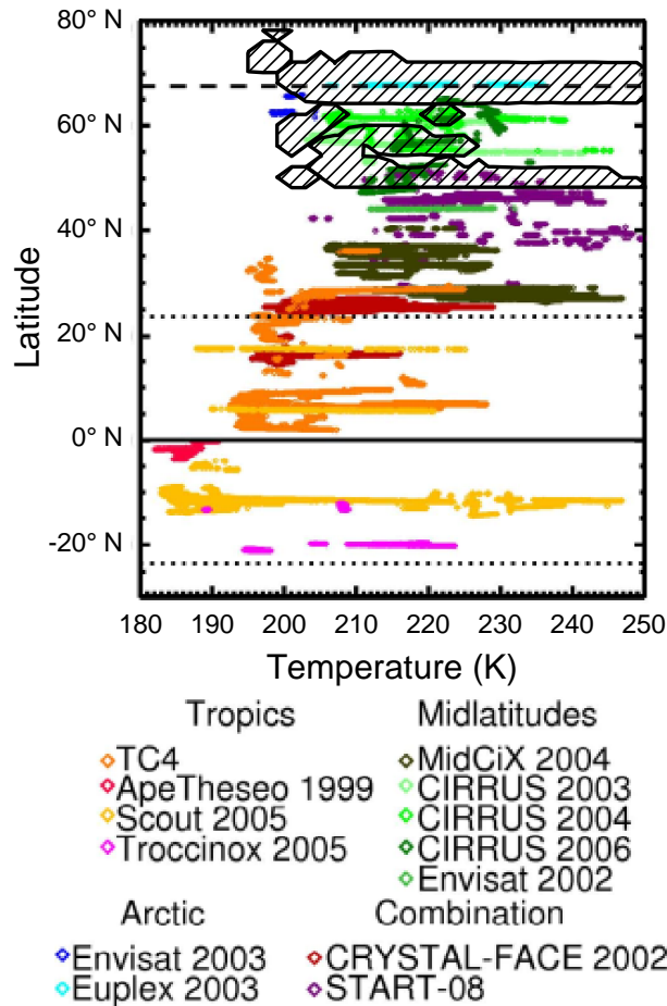
Figure 3. The original of this figure is found in Luebke et al. (2013). It shows black contour and diagonal stripes sketch the coverage of literature airborne cirrus missions (different colors, legend in the original publication) measurements during POLSTRACC with respect to latitude and temperature. For this work, the original of this figure from Luebke et al. (2013) is adapted to sketch, showing the additional coverage of literature airborne in situ cirrus measurements during POLSTRACC by a black contour and diagonal stripes missions.
