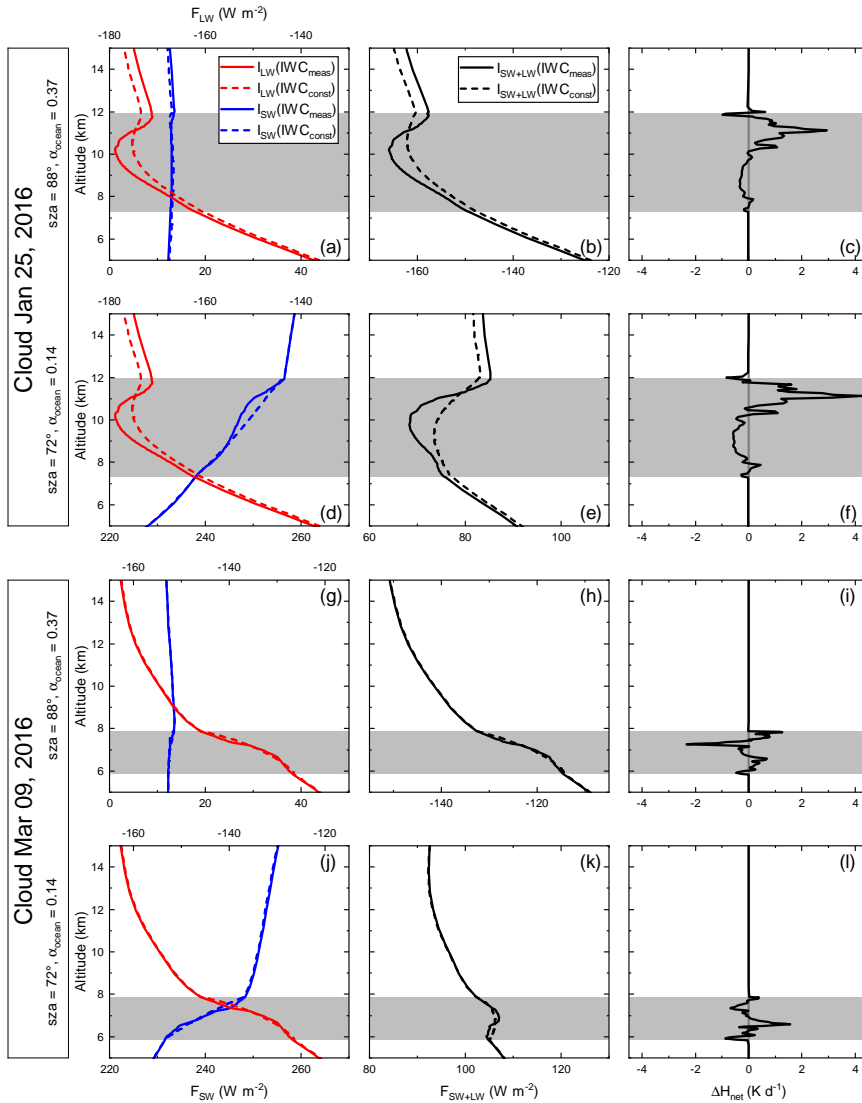
Figure 11. Irradiance profiles of measured (solid) and constant (dashed) IWC profiles for selected values of solar zenith angle and albedo as indicated. Left column: LW (red, top axis scale) and SW (blue, bottom axis scale) irradiances. The top axis is shown in negative numbers since F_{LW} is upward directed. Centre column: net irradiances. All irradiance scales span a range of 50 \text{ W m}^{-2} , albeit at different absolute positions. Right column: Difference of the net heating rate profile between the measured and the constant IWC profile.
