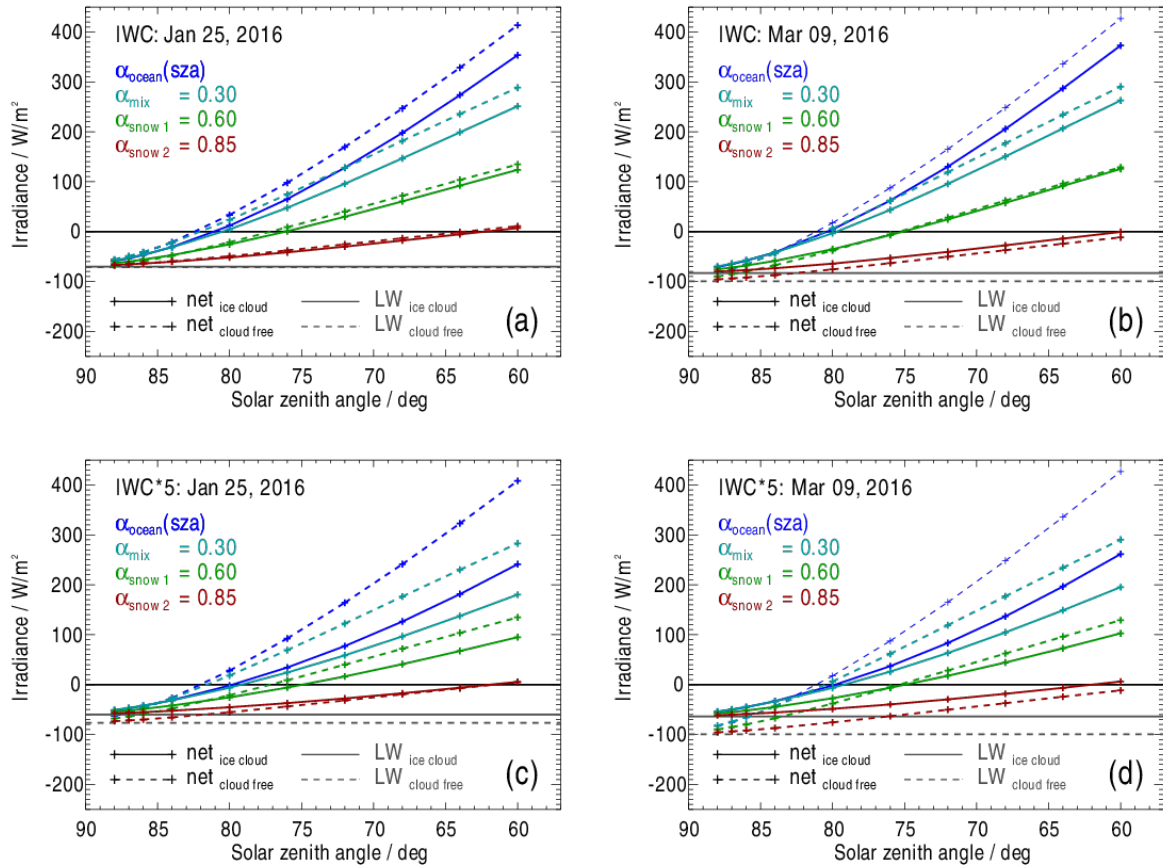
Figure 9. Net irradiances Irradiance at the bottom of the atmosphere (surface), otherwise as in Fig. 8.
