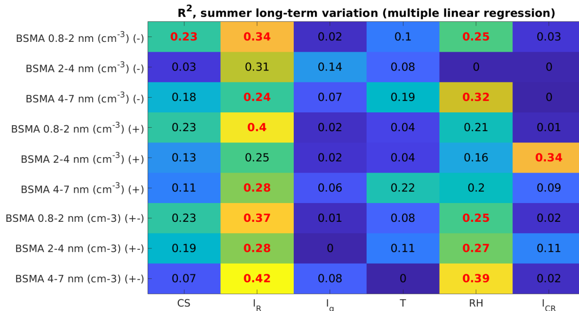
A3: The amount of variation explained by our chosen explanatory variables for each size range and polarity. The data points selected are only between June and August and represent changes in summertime concentrations. The symbol (-) denotes negative polarity, (+) a positive polarity and (+-) the sum of both polarities. The bolded red values are statistically significant ( p < 0.05 ).
