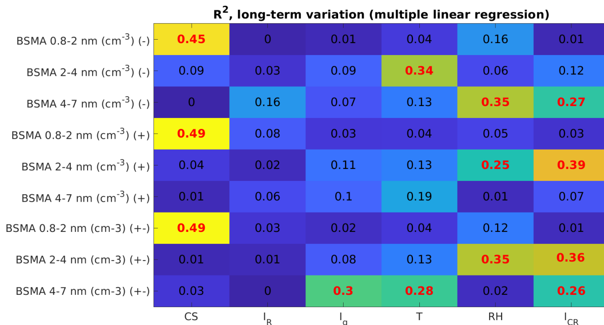
270 Figure 8: The amount of variation explained by our chosen explanatory variables for each size range and polarity for BSMA. The symbol (-) denotes negative polarity, (+) a positive polarity and (+-) the sum of both polarities. The bolded red values are statistically significant ( p < 0.05 ).
