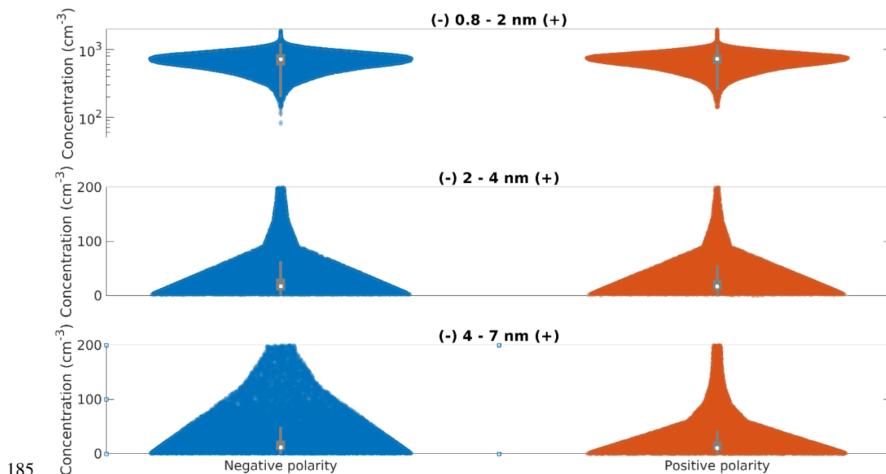
Figure 3: Measured ion concentrations. Negative polarity is on the left in blue and positive polarity is on the right in orange. The cluster ion (0.8 – 2 nm) concentrations are on the top row, and intermediate ion concentrations are in the middle and bottom, 2 – 4 nm and 4 – 7 nm, respectively. The white dot is the median concentration and the whiskers mark the location of the 95th and 5th percentile data points.
