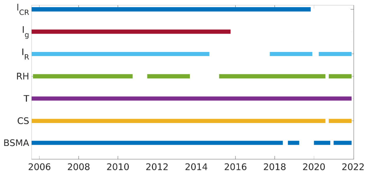
Figure 2: Time periods when data is available for variables we used in our analysis. I_{CR} is the cosmic ray ionization rate, I_g is the gamma ionization rate, I_R is the radon ionization rate, RH is relative humidity, T is temperature and CS is the condensation sink. BSMA is the ion spectrometer used in the study.
