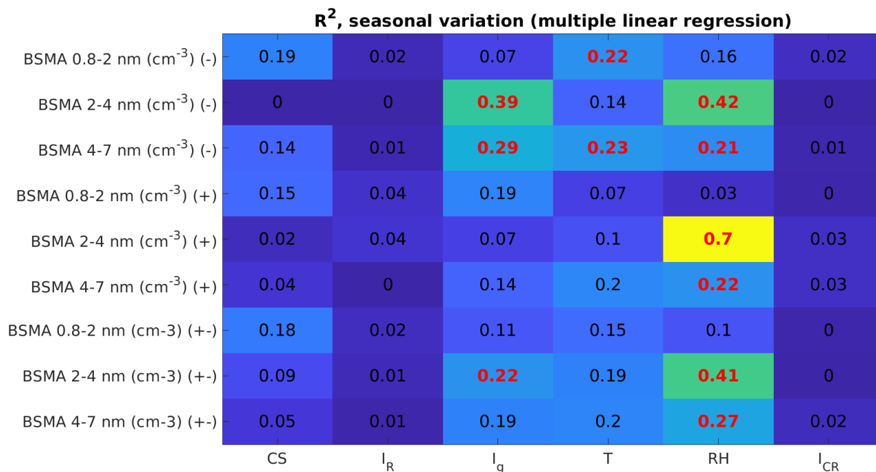
310 Figure 9: The amount of seasonal variation explained by our chosen explanatory variables for each size range and polarity. The symbol (-) denotes negative polarity, (+) a positive polarity and (+-) the sum of both polarities. The bolded red values are statistically significant ( p < 0.05 ).
