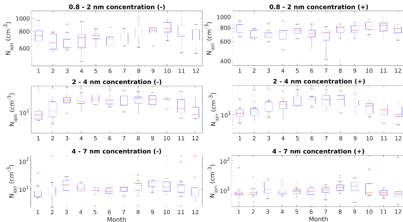
235 Figure 6: The annual variance of ion concentrations in the size bins, 0.8 – 2 nm, 2 – 4 nm and 4 – 7 nm. The left-hand side boxplots are in the negative polarity and the right-hand side are in the positive polarity. The numbers on the x-axis are month numbers (Jan-Dec). The red line is the median concentration, and the blue box contains 50% (25 th to 75 th percentile) of all data points. The whiskers mark the location of the 95 th and 5 th percentile data points.
