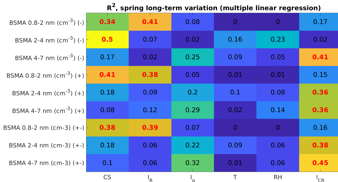
A2: The amount of variation explained by our chosen explanatory variables for each size range and polarity. The data points selected are only between March and May and represent changes in springtime concentrations. The symbol (-) denotes negative polarity, (+) a positive polarity and (+-) the sum of both polarities. The bolded red values are statistically significant ( p < 0.05 ).
