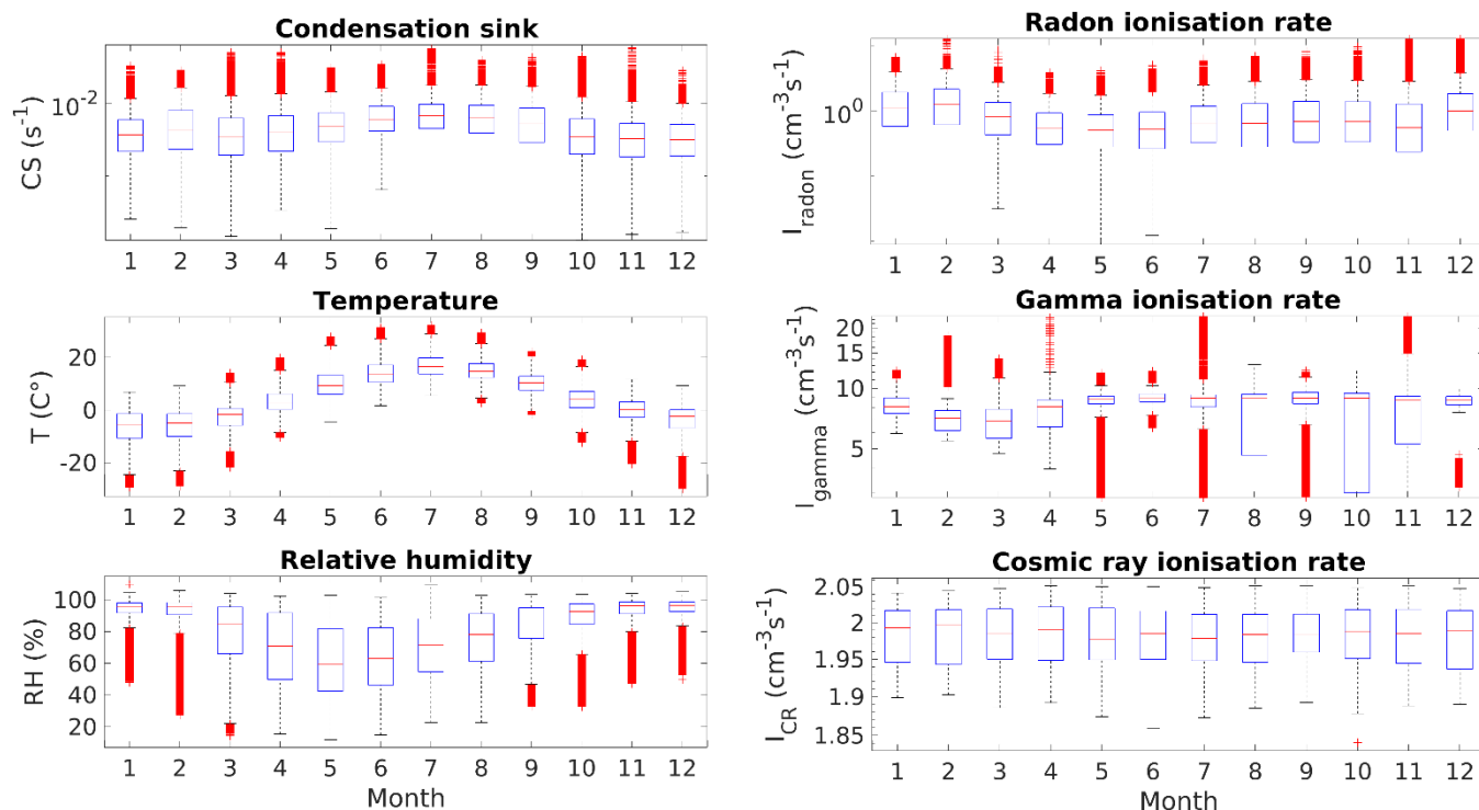
250 Figure 7: The annual variation of CS, T, RH, I_r , I_g , I_{CR} . The red line is the median concentration, and the blue box contains 50% (25 th to 75 th percentile) of all data points. The whiskers mark the location of the 95 th and 5 th percentile data points. The numbers on the x-axis are month numbers.
