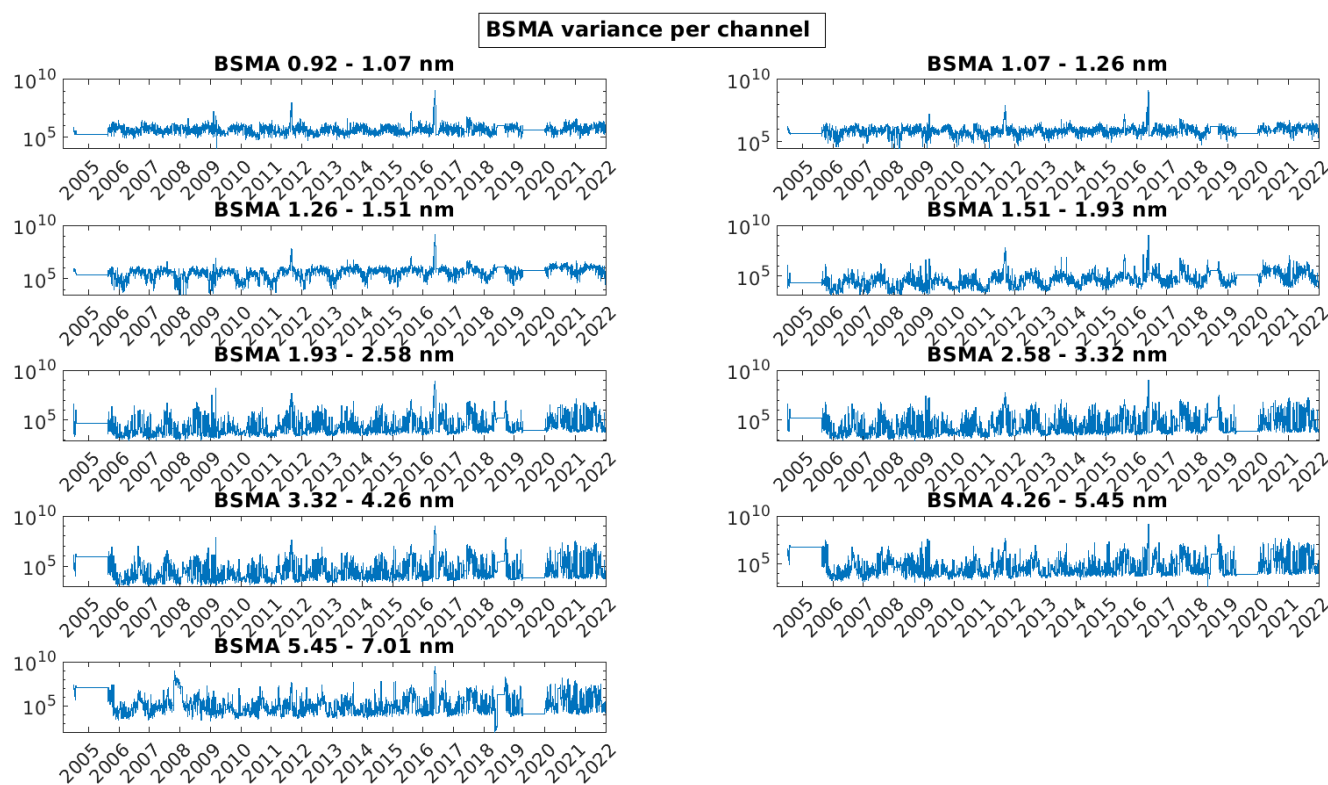
605 A1: Variance of the concentration time series of the BSMA size channels.
