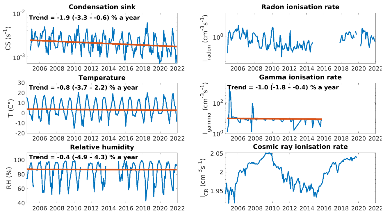
Figure 5: The time series of main sources and sinks as well as temperature and relative humidity. The relative changes per year have been calculated from Sen's slopes.
