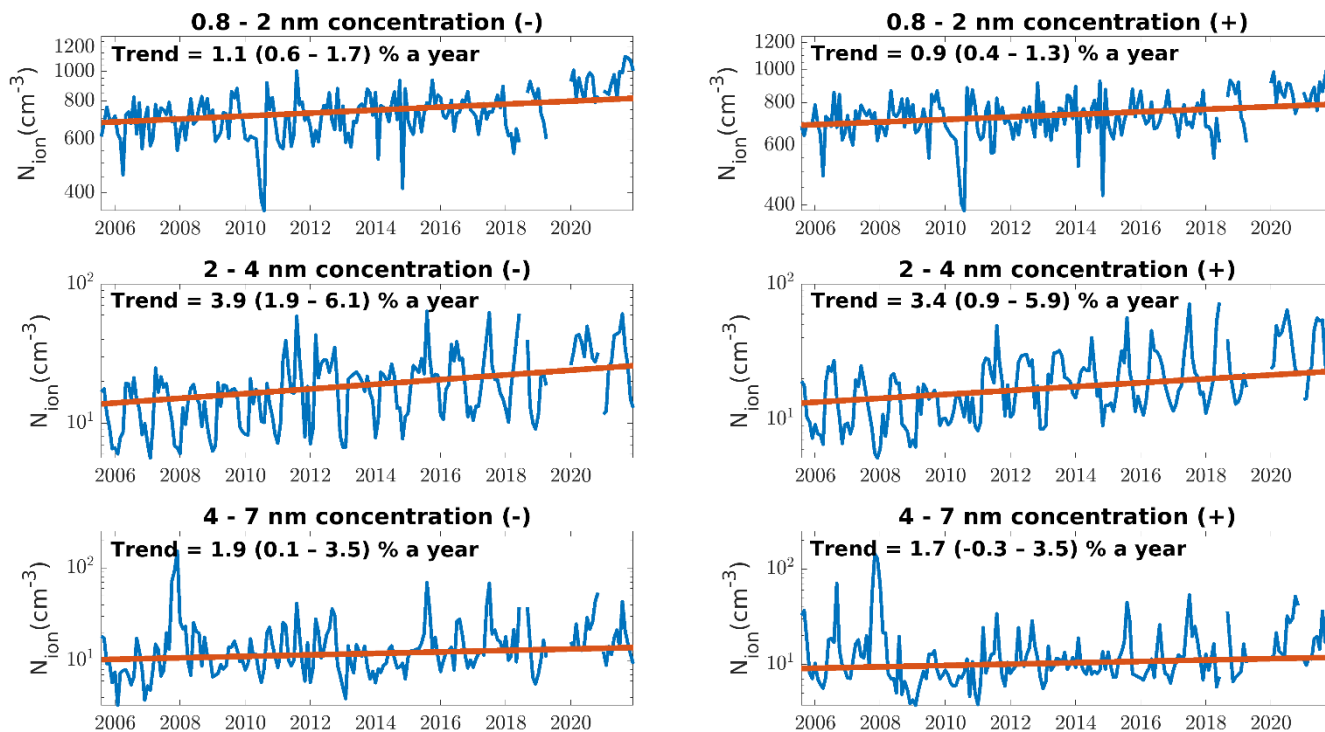
205 Figure 4: The time series of the cluster and intermediate ion concentrations. The relative changes per year have been calculated from Sen's slopes.
