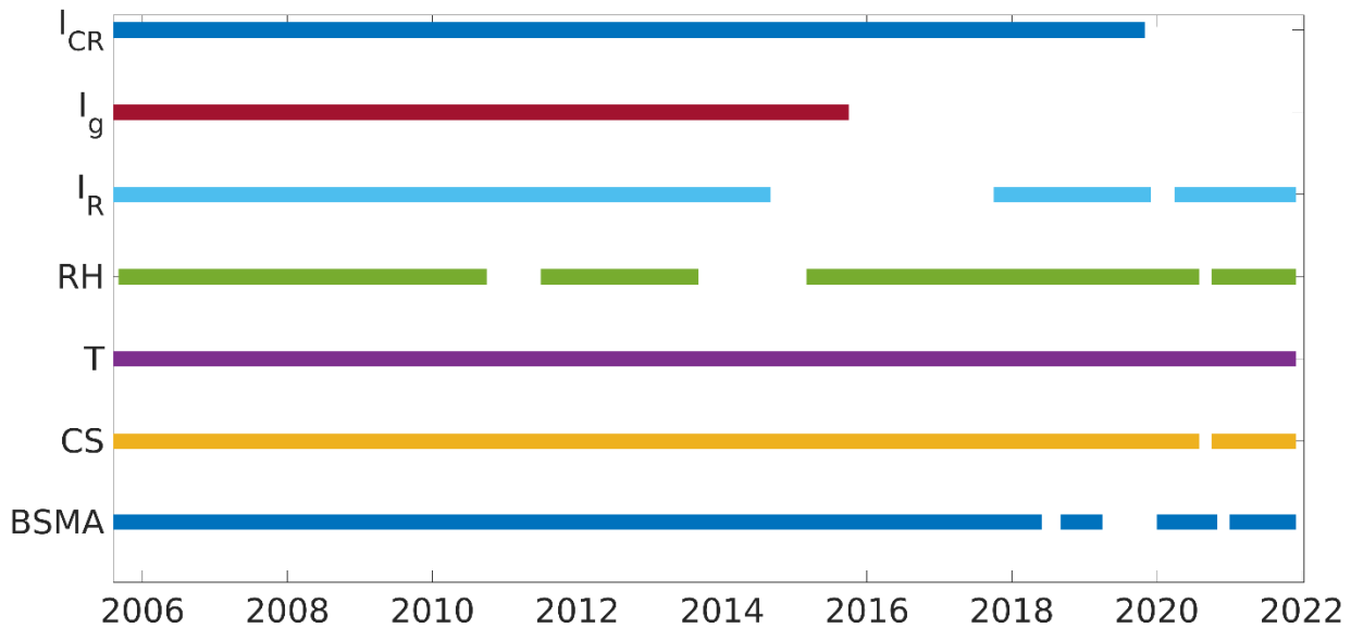
Figure 2: Time periods when data are available for variables we used in our analysis. I_{CR} is the cosmic ray ionization rate, I_g is the gamma ionization rate, I_R is the radon ionization rate, RH is relative humidity, T is temperature and CS is the condensation sink. BSMA is the ion spectrometer used in the study.
