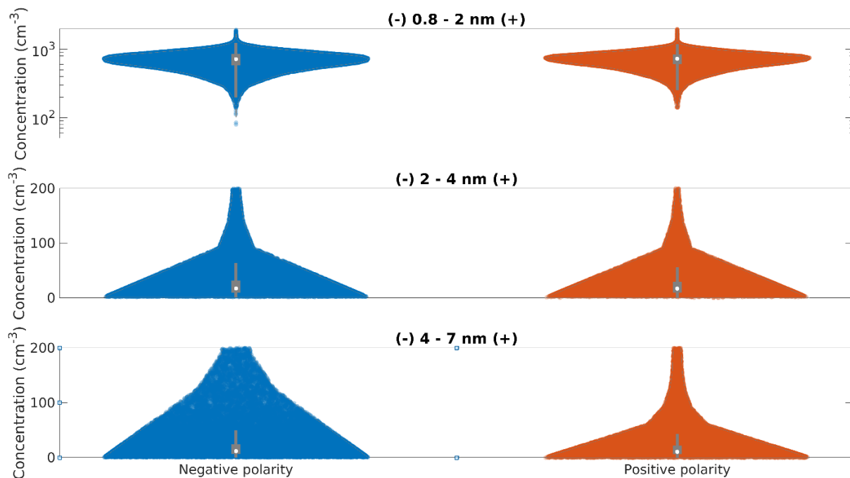
205 Figure 3: Measured ion concentrations. Negative polarity is on the left in blue and positive polarity is on the right in orange. The cluster ion (0.8 – 2 nm) concentrations are on the top row, and intermediate ion concentrations are in the middle and bottom, 2 – 4 nm and 4 – 7 nm, respectively. The white dot is the median concentration and the whiskers mark the location of the 95th and 5th percentile data points.
