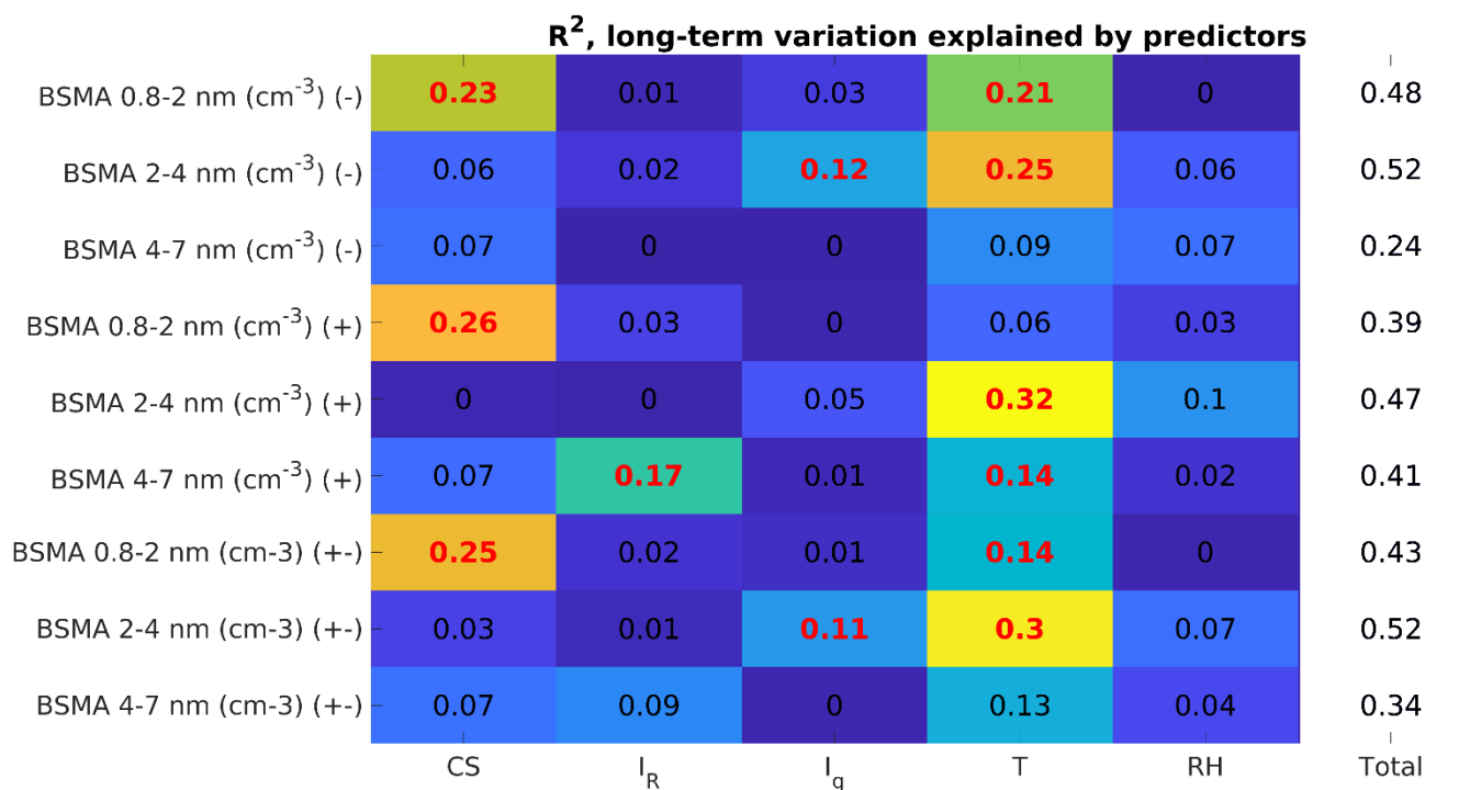
Figure 8: The amount of variation explained by our chosen explanatory variables for each size range and polarity for BSMA. The symbol (-) denotes negative polarity, (+) a positive polarity and (+-) the sum of both polarities. The bolded red values are statistically significant ( p < 0.05 ).
