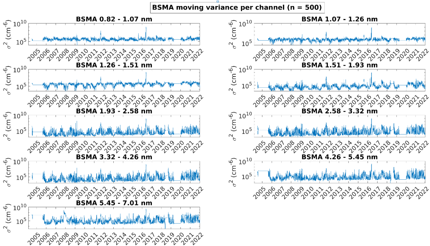
660 A1: Moving variance of the concentration time series of the BSMA size channels. The symbol n indicates the number of closest data points used for the calculation of the variance at each point. The time resolution is the time resolution of the instrument which is 12 minutes.
