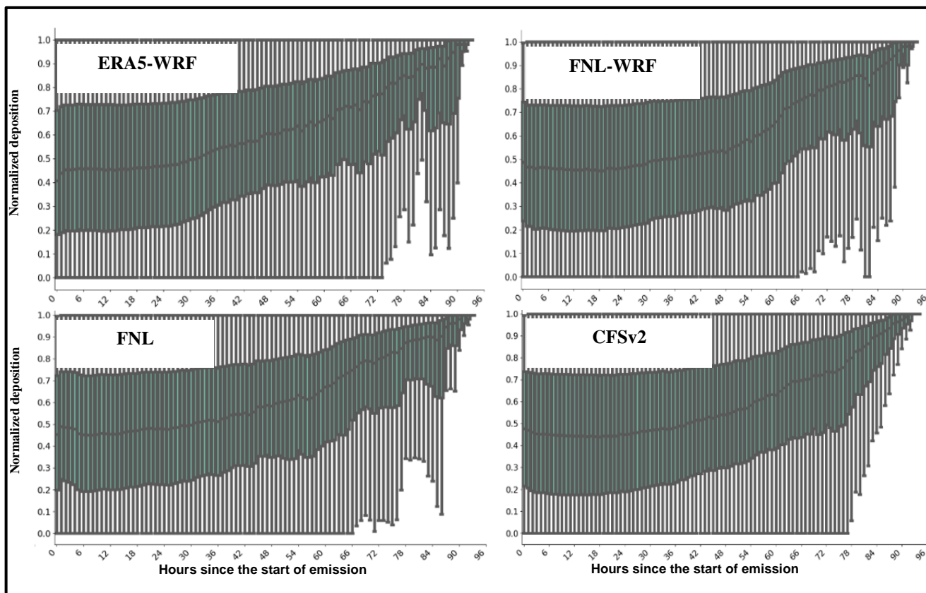
Figure 4 the deposition of ^{137}\text{Cs} normalized to the total amount of each four-day simulation period at each grid cell. This plot (S5) shows simulations in winter (other seasons). The x-axis shows the age of Lagrangian particles and the y-axis is the normalized deposition. Error bars show the 25th and 75th percentiles (the lower and upper quartiles) and the range of normalized deposition (the upper and lower extremes) within the study area.
