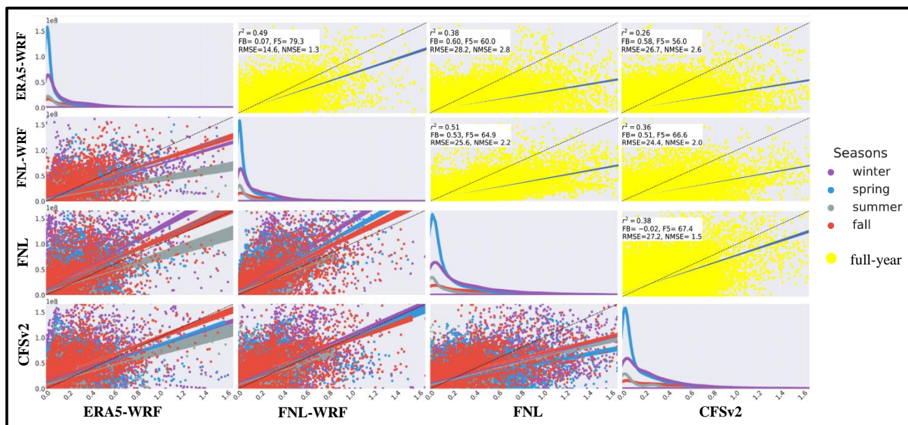
Figure 11 The inter-comparison of the 96-hour integrated simulations of ^{131}\text{I} column densities (Bq/m 2 ) from FLEXPART and FLEXPART-WRF runs. The reported model metrics, in the upper triangle of evaluation matrix plot, show the performance of
