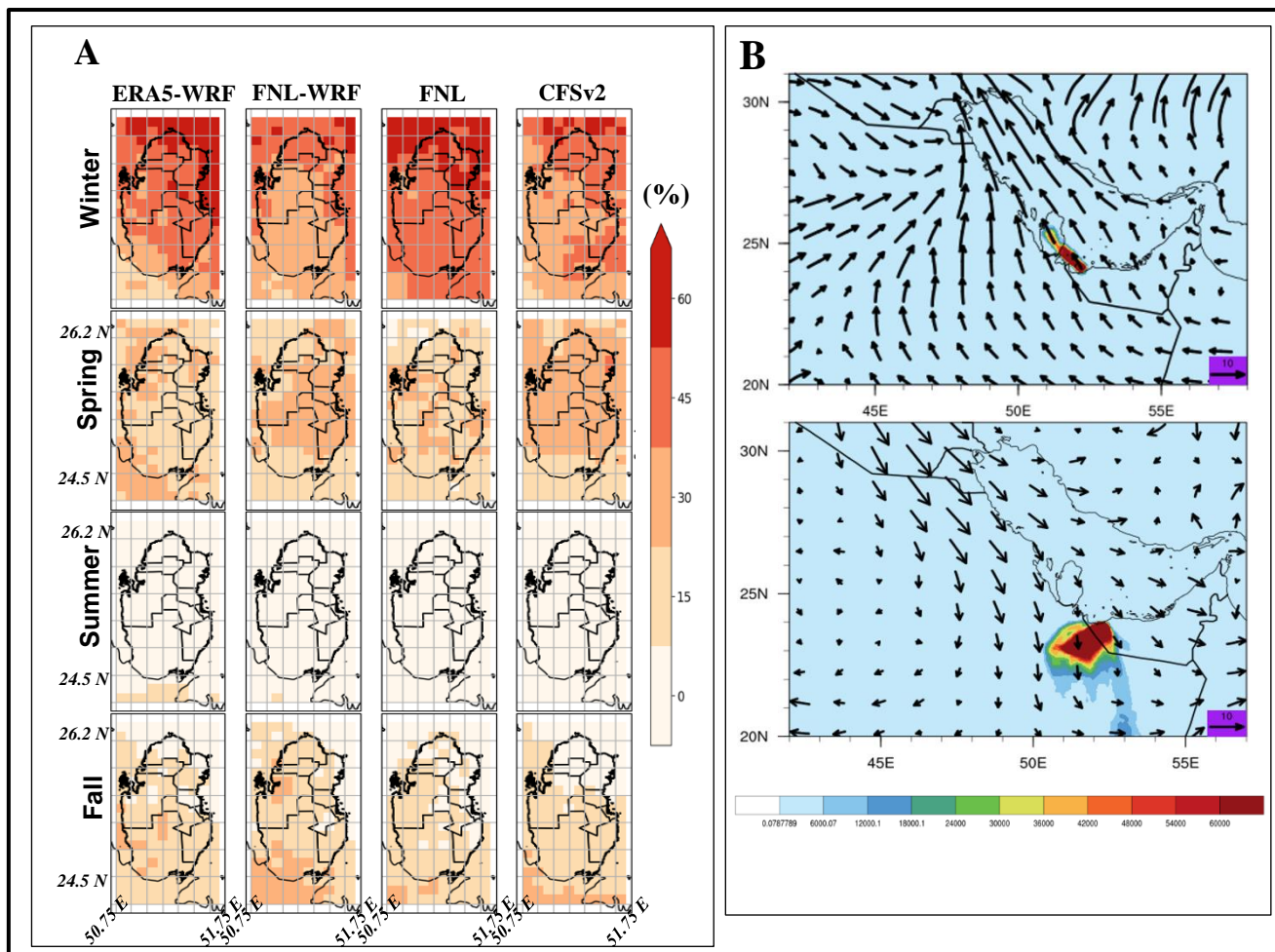
Figure 9 A: The frequency of occurrence (%) of ^{131}\text{I} column densities above the respective 66 th percentile. B: ERA5-WRF ^{131}\text{I} column density ( \text{Bq m}^{-3} ) on January 14, 2019, at noon (top) and the summertime average of ^{131}\text{I} column density (bottom). Overlying vectors show wind streams at 150 m agl. To represent atmospheric circulations during the release of radionuclides, wind data at 12 p.m. on the first day of the four-day simulation period was used.
