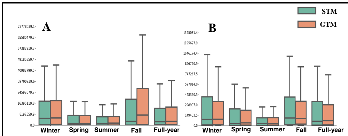
Figure 10 Panels A and B show the 96-hour integrated simulations of column densities of ^{131}\text{I} (Bq/m 2 ) and total deposition of ^{137}\text{Cs} (Bq/m 2 ) from ERA5-WRF with STM (green, sensitivity run) and GTM (brown, control run), respectively. The same outputs for FNL-WRF are shown in S11.
