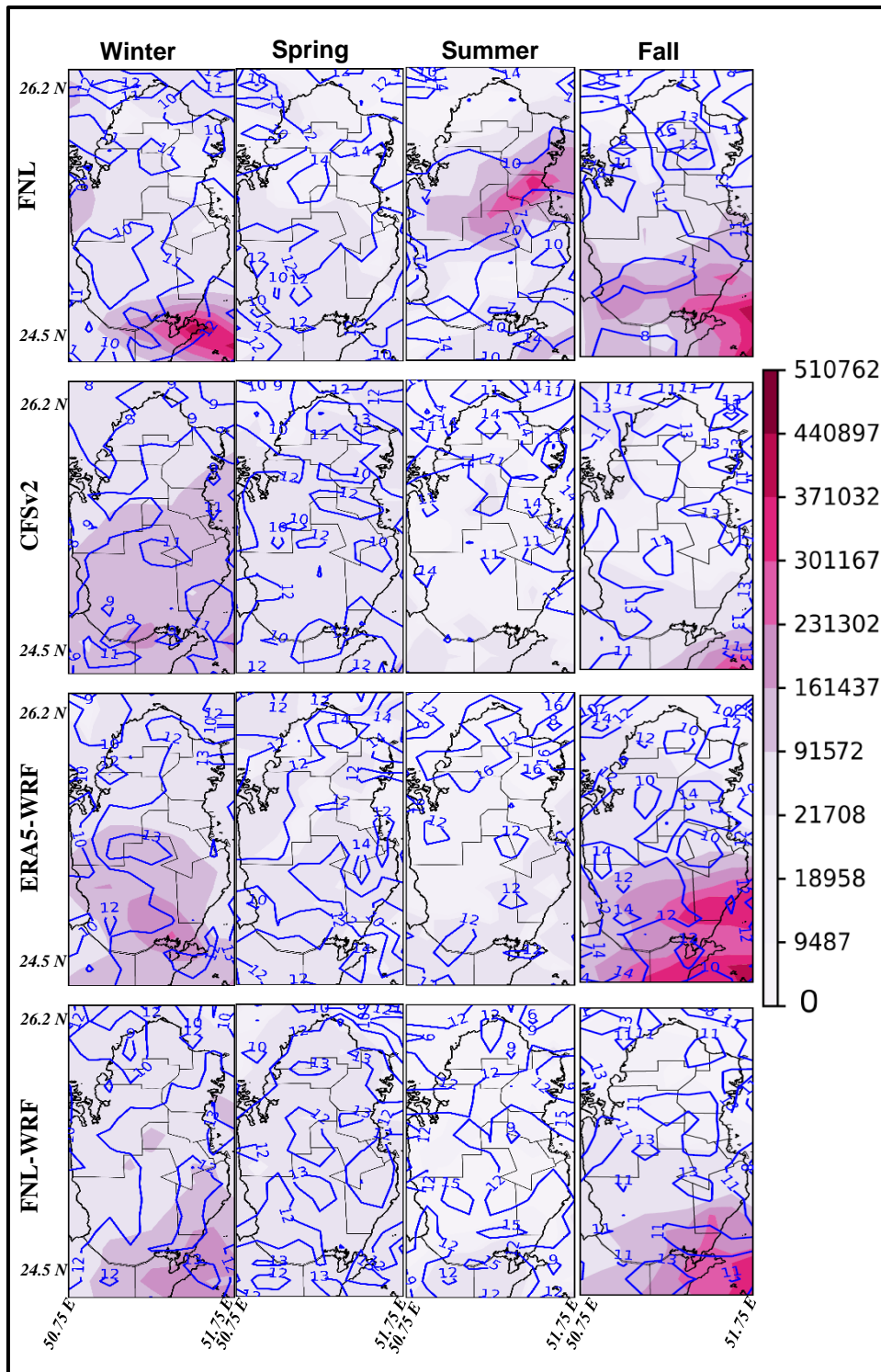
Figure 6 Same as 5, but for the seasonal median of ^{137}\text{Cs} deposition ( ^{137}\text{Cs}_{\text{tot\_depos\_seas}} ) in the unit of \text{Bqm}^{-2} .
