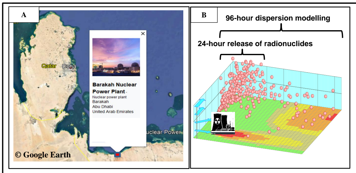
200 Figure 1 A is the study area embracing the B-NPP (red square) and the state of Qatar. The base map and overlaying information are taken from Google Earth. B is the schematic illustration of the LPDM simulation cycle. The original figure is available at https://www.janicke.de/en/lasat.html (last access: 4 October 2022).
