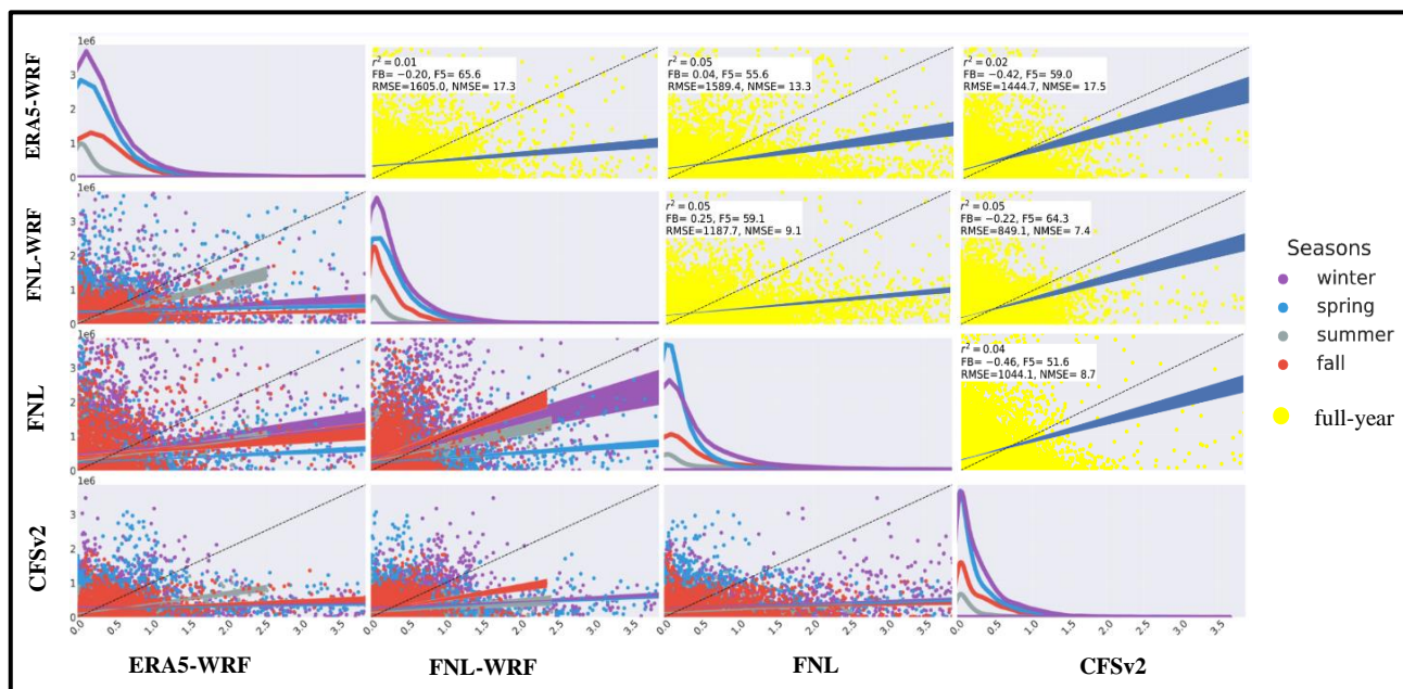
485 Figure 12 Same as Figure 11 but for ^{137}\text{Cs} deposition
