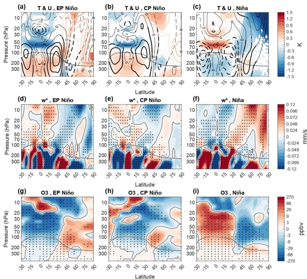
150 Figure 1. Latitude - pressure cross sections of the composite of NDJF zonal mean (a-c) temperature (colors) and zonal wind (black contours), (d-f) vertical component of the residual circulation w^* and (g-i) ozone mixing ratio anomalies for (from left to right) EP El Niño, CP El Niño and La Niña events. Contours in upper panels are drawn every 0.6 m s -1 for zonal wind and 0.15 K for temperature. Solid (dashed) contours denote positive (negative) anomalies. The NDJF mean tropopause is indicated by the thick grey line. Color shading (upper panels) denotes statistically significant anomalies at the 95 % confidence level for temperature and 155 black dots (middle and bottom panels) the same for w^* and ozone mixing ratio. Thick black contours (upper panels) denote statistically significant anomalies for zonal wind.
