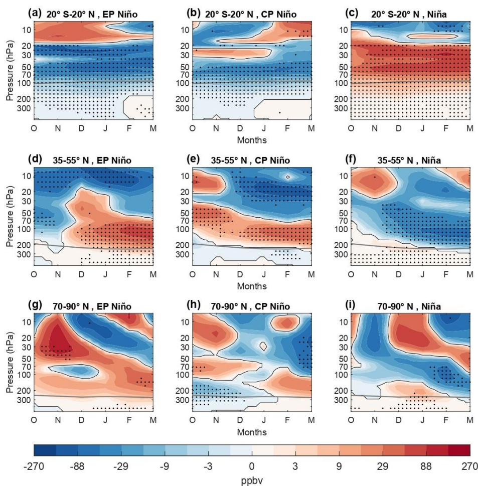
270 Figure 3. October to March composite evolution of ozone mixing ratio anomalies (ppbv) as a function of pressure (a-c) in the tropics ( 20^{\circ} S- 20^{\circ} N), (d-f) at mid-latitudes ( 35^{\circ} - 55^{\circ} N) and (g-i) in the Arctic ( 70^{\circ} - 90^{\circ} N) for (from left to right) EP El Niño, CP El Niño and La Niña events. Black dots denote statistically significant anomalies at the 95 % confidence level. The tropopause is indicated by the thick grey line.
