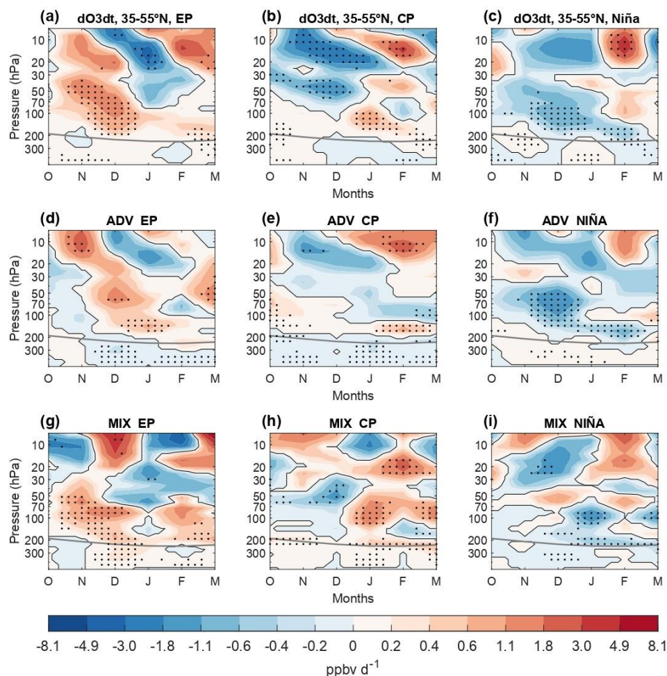
Figure 5. As in Fig. 4 but average over 35-55° N and for anomalies in DO3dt (a-c), ADV (d-f), and MIX (g-i), which represents changes related to mixing.
