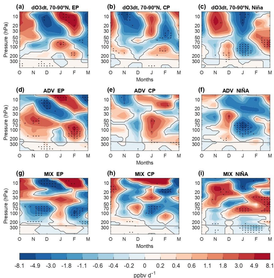
Figure 7. As in Fig. 5 but average over 70-90° N.
