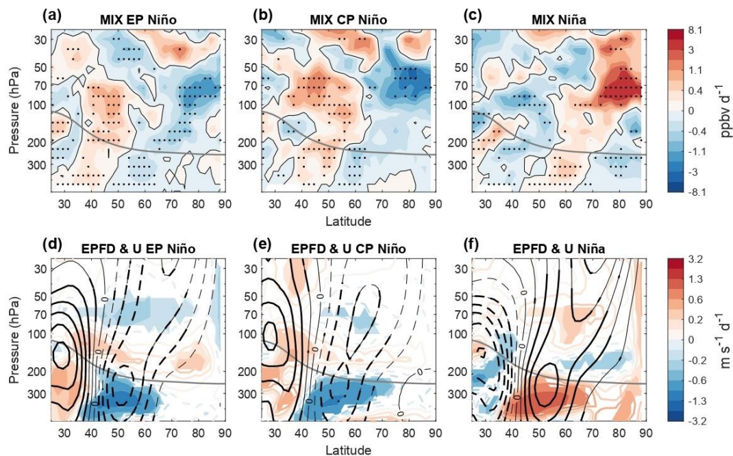
Figure 6. Latitude-pressure cross sections of the composite of NDJFM zonal mean (EP El Niño) and JFM (CP El Niño and La Niña) (a-c) Ozone tendency related to mixing and (d-f) EPFD (colors) and zonal wind (black contours) for (from left to right) EP El Niño, CP El Niño and La Niña events. Contours in bottom panels are drawn every 0.5 m s -1 for zonal winds. Solid (dashed) contours denote positive (negative) anomalies. The NDJFM or JFM mean tropopause is indicated by the thick grey line. Color shading (bottom panels) and black dots (upper panels) denote statistically significant anomalies at the 95 % confidence level; thick contours denote statistically significant anomalies for zonal wind.
