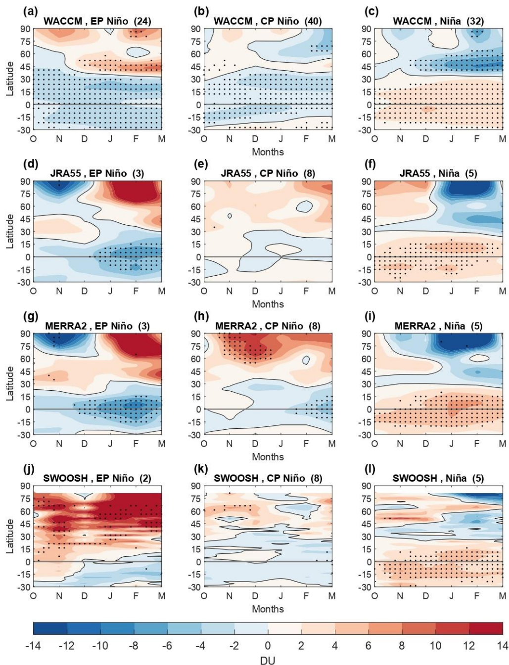
Figure 2. October to March composite evolution of total column ozone (TCO) anomalies (DU) as a function of latitude in (a-c) WACCM, (d-f) JRA55, (g-i) MERRA2 and (j-l) SWOOSH for (from left to right) EP El Niño, CP El Niño and La Niña events. Numbers in brackets indicate the number of events in each composite. Black dots denote statistically significant anomalies at the 95 % confidence level.
