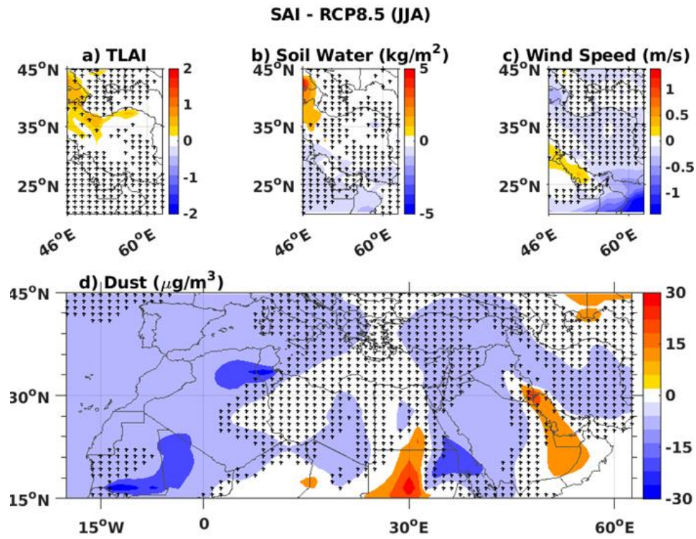
Figure S1: differences of SAI and RCP8.5 simulations for mean values of (a) total leaf area index, (b) soil water and (c) wind speed for the Middle East region in summer time. (d) difference of SAI and RCP8.5 dust concentration in the MENA region in summer time.
