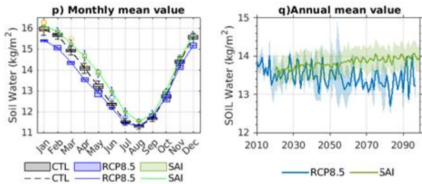
645 Figure 8: The same as Fig 5 but for the top 10 cm soil water
