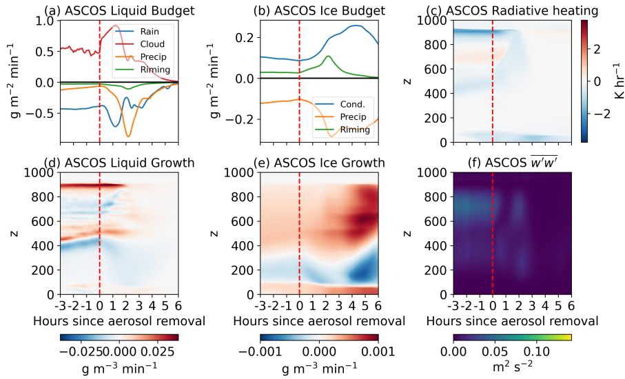
Figure 8. Same as Figure 7 for ASCOS.
