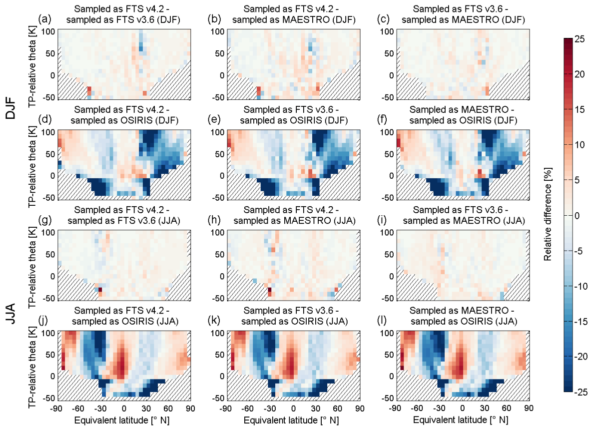
Figure 6. Same as Fig. 3, but for ozone, and including an additional two rows for comparisons involving climatologies constructed from the OSIRIS measurement pattern. Note that the DJF and JJA comparisons are now spread over two rows each, with the top two rows corresponding to the former, and the bottom two to the latter.
